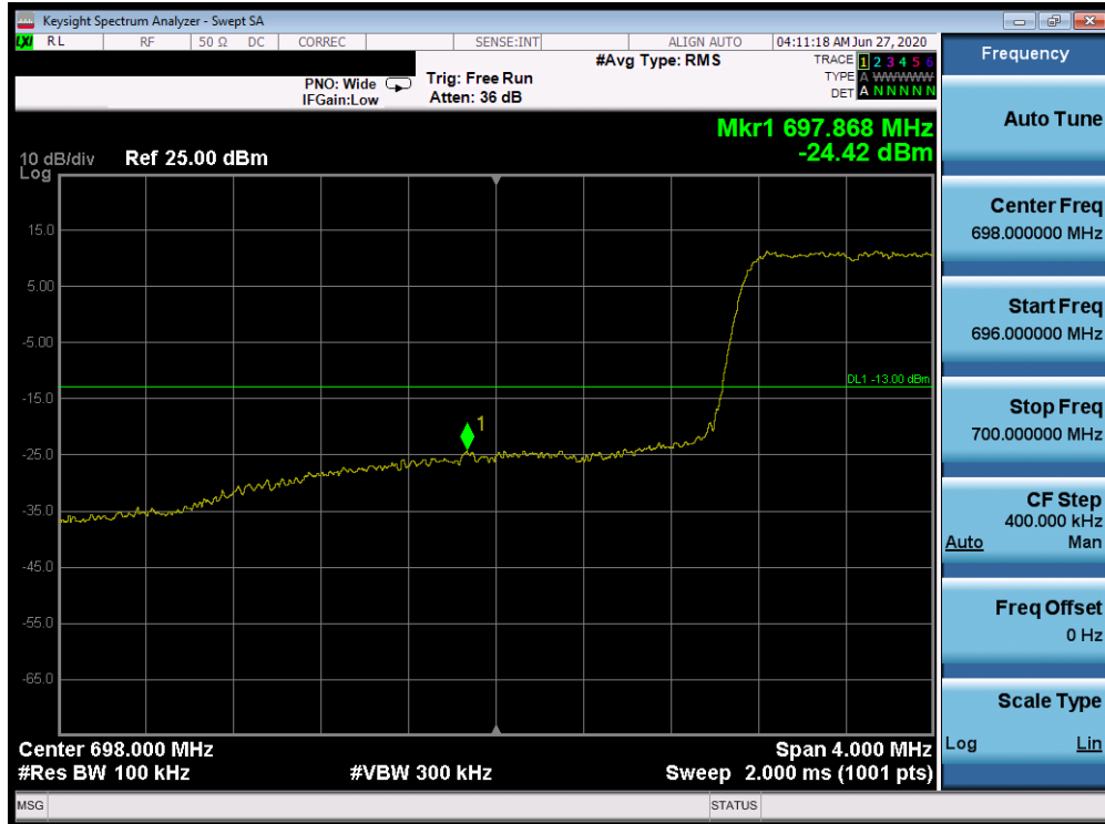
Plot 7-392. Lower Band Edge Plot (Band 12 - 3.0MHz QPSK - Full RB Configuration)
