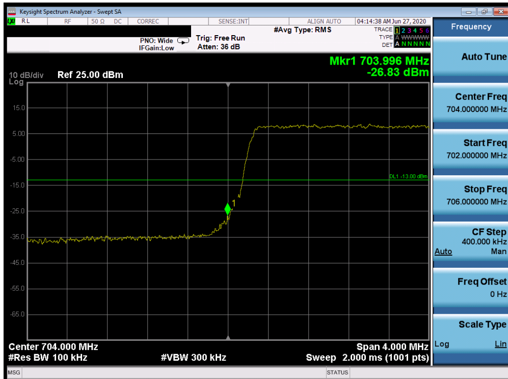
Plot 7-395. Lower Band Edge Plot (Band 17 - 5.0MHz QPSK - Full RB Configuration)
