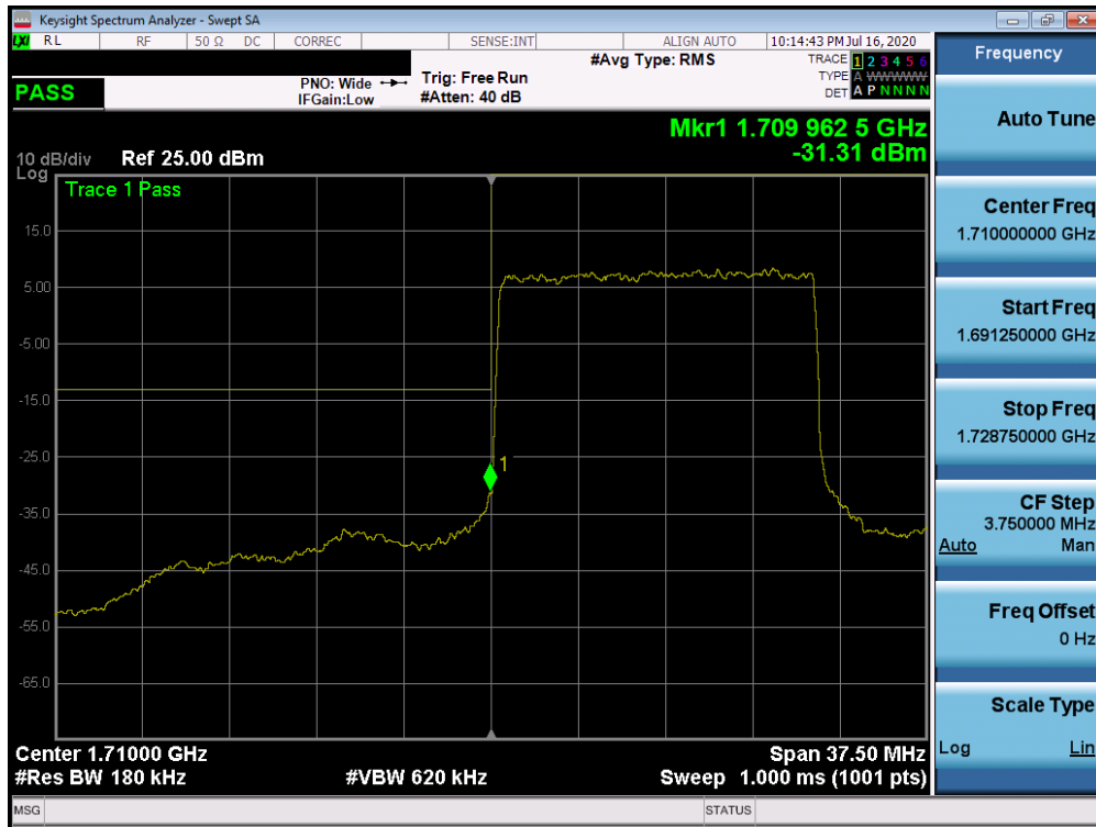
Plot 7-476. Lower Band Edge Plot (n66 - 15MHz DFT-s-OFDM-QPSK - Full RB Configuration)
