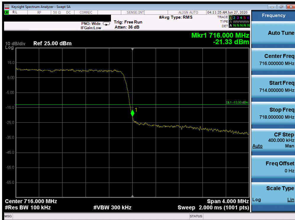
Plot 7-393. Upper Band Edge Plot (Band 12 - 3.0MHz QPSK - Full RB Configuration)
