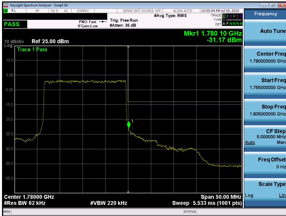
Plot 7-462. Upper Band Edge Plot (n66 - 20MHz DFT-s-OFDM-QPSK - Full RB Configuration)
