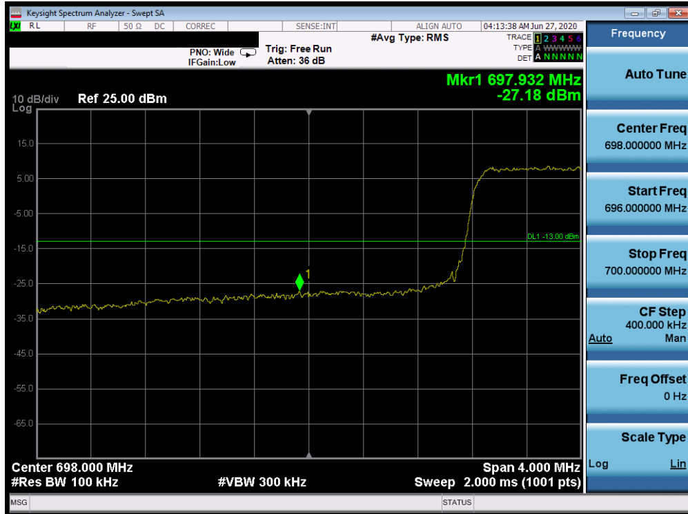
Plot 7-394. Lower Band Edge Plot (Band 12 - 5.0MHz QPSK - Full RB Configuration)
