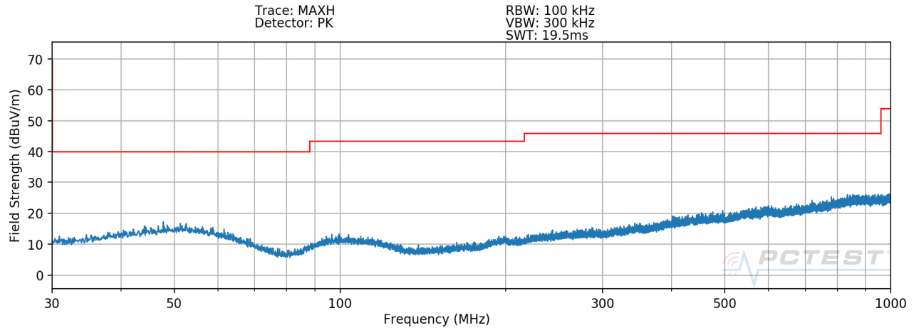
Plot 7-4. Radiated Spurious Plot 30MHz – 1GHz (Pol. H)
