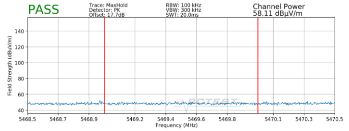
Plot 7-197. Radiated Lower Band Edge Plot SISO ANT2 (Peak - UNII Band 2C)
