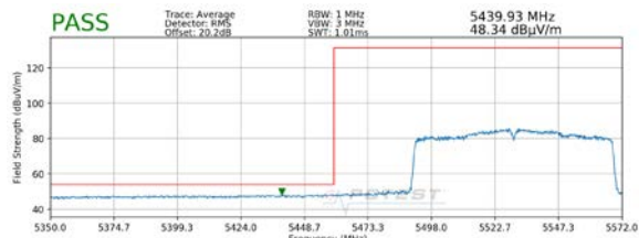
Plot 7-19. Radiated Lower Band Edge Plot SISO ANT1 (Average – UNII Band 2C)
