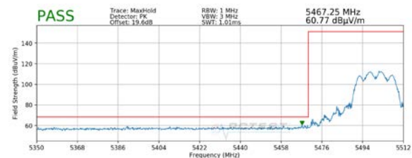
Plot 7-27. Radiated Lower Band Edge Plot MIMO (Peak – UNII Band 2C)
