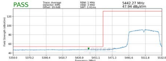
Plot 7-12. Radiated Lower Band Edge Plot SISO ANT1 (Average – UNII Band 2C)
