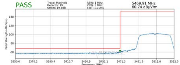
Plot 7-13. Radiated Lower Band Edge Plot SISO ANT1 (Peak – UNII Band 2C)
