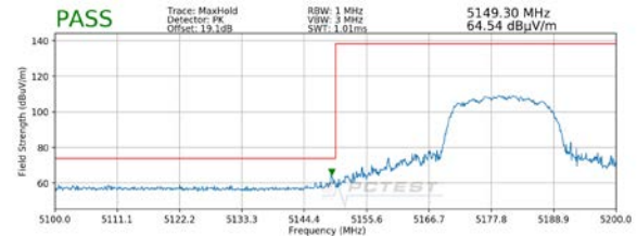
Plot 7-23. Radiated Lower Band Edge Plot MIMO (Peak – UNII Band 1)
