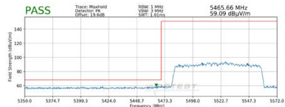
Plot 7-45. Radiated Lower Band Edge Plot MIMO (Peak – UNII Band 2C)
