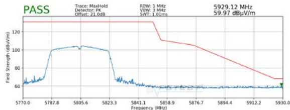
Plot 7-14. Radiated Upper Band Edge Plot SISO ANT1 (Peak – UNII Band 3)
