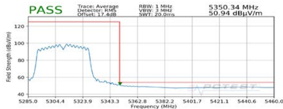
Plot 7-38. Radiated Upper Band Edge Plot MIMO (Average – UNII Band 2A) with Dual Display
