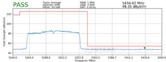
Plot 7-42. Radiated Upper Band Edge Plot MIMO (Average – UNII Band 2A)
