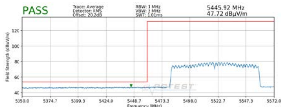
Plot 7-44. Radiated Lower Band Edge Plot MIMO (Average – UNII Band 2C)
