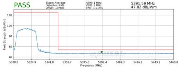
Plot 7-3. Radiated Upper Band Edge Plot SISO ANT1 (Average – UNII Band 2A)
