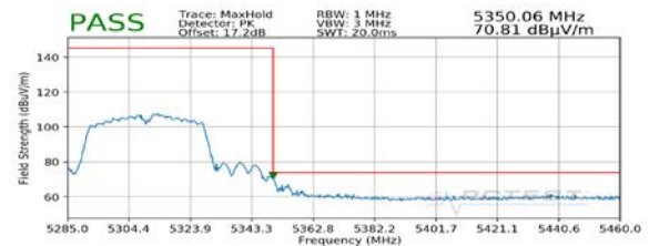
Plot 7-39. Radiated Upper Band Edge Plot MIMO (Peak – UNII Band 2A) with Dual Display
