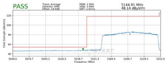
Plot 7-15. Radiated Lower Band Edge Plot SISO ANT1 (Average – UNII Band 1)
