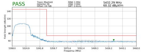
Plot 7-4. Radiated Upper Band Edge Plot SISO ANT1 (Peak – UNII Band 2A)
