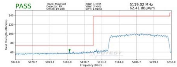
Plot 7-41. Radiated Lower Band Edge Plot MIMO (Peak – UNII Band 1)
