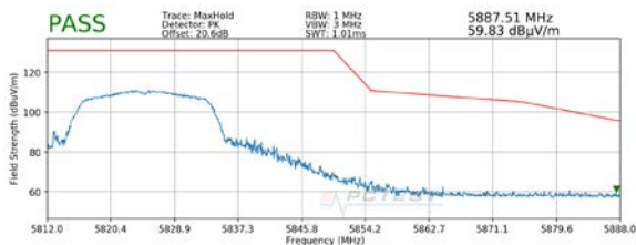
Plot 7-7. Radiated Upper Band Edge Plot SISO ANT1 (Peak – UNII Band 3)
