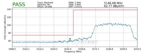
Plot 7-32. Radiated Lower Band Edge Plot MIMO (Peak – UNII Band 1)
