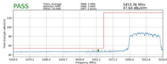
Plot 7-35. Radiated Lower Band Edge Plot MIMO (Average – UNII Band 2C)
