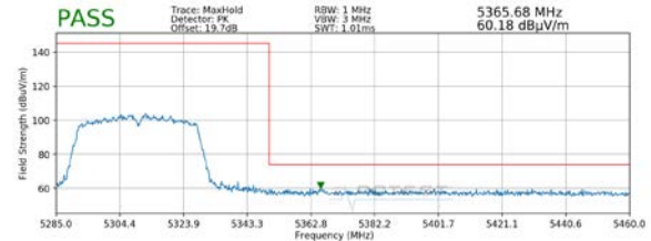
Plot 7-34. Radiated Upper Band Edge Plot MIMO (Peak – UNII Band 2A)
