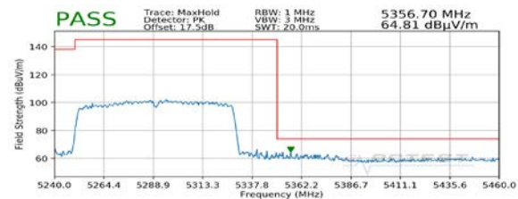
Plot 7-48. Radiated Upper Band Edge Plot MIMO (Peak – UNII Band 2A) with Dual Display
