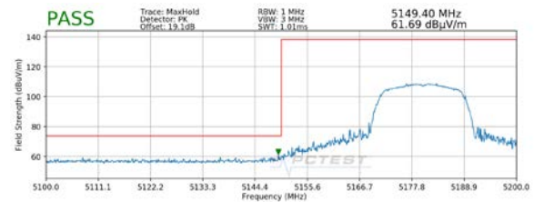
Plot 7-2. Radiated Lower Band Edge Plot SISO ANT1 (Peak – UNII Band 1)
