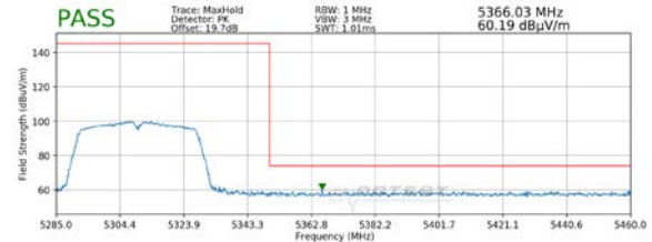
Plot 7-11. Radiated Upper Band Edge Plot SISO ANT1 (Peak – UNII Band 2A)
