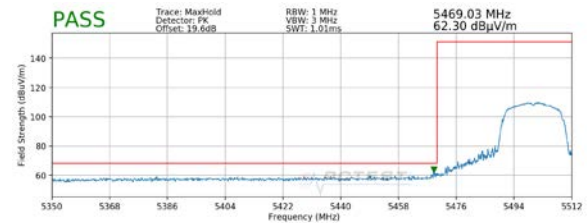
Plot 7-6. Radiated Lower Band Edge Plot SISO ANT1 (Peak – UNII Band 2C)
