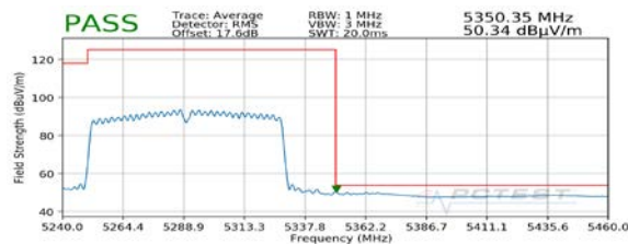
Plot 7-47. Radiated Upper Band Edge Plot MIMO (Average – UNII Band 2A) with Dual Display
