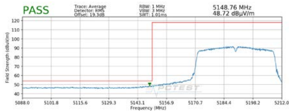
Plot 7-8. Radiated Lower Band Edge Plot SISO ANT1 (Average – UNII Band 1)
