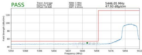
Plot 7-5. Radiated Lower Band Edge Plot SISO ANT1 (Average – UNII Band 2C)
