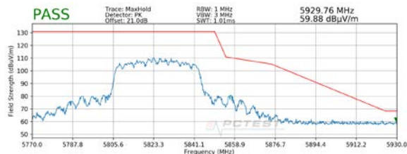
Plot 7-37. Radiated Upper Band Edge Plot MIMO (Peak – UNII Band 3)
