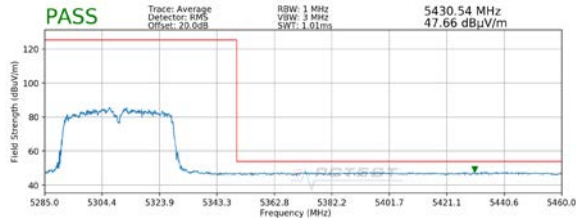
Plot 7-33. Radiated Upper Band Edge Plot MIMO (Average – UNII Band 2A)
