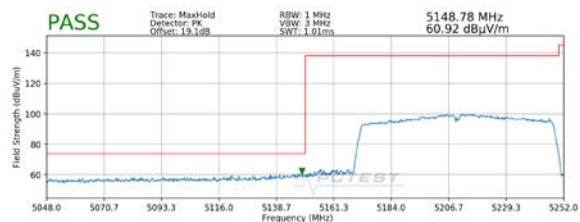
Plot 7-16. Radiated Lower Band Edge Plot SISO ANT1 (Peak – UNII Band 1)
