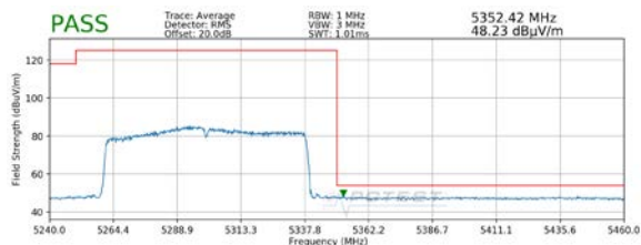
Plot 7-17. Radiated Upper Band Edge Plot SISO ANT1 (Average – UNII Band 2A)
