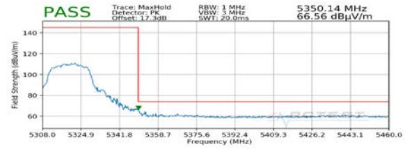
Plot 7-30. Radiated Upper Band Edge Plot MIMO (Peak – UNII Band 2A) with Dual Display
