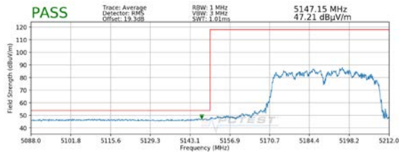
Plot 7-31. Radiated Lower Band Edge Plot MIMO (Average – UNII Band 1)
