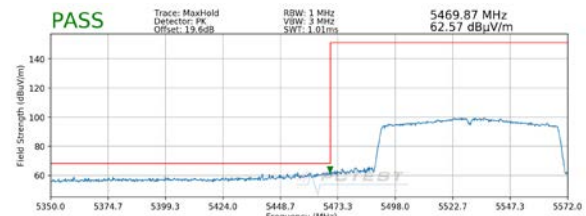
Plot 7-20. Radiated Lower Band Edge Plot SISO ANT1 (Peak – UNII Band 2C)
