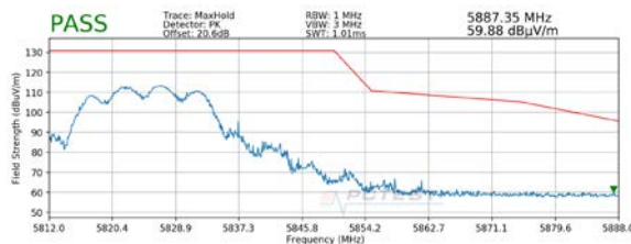
Plot 7-28. Radiated Upper Band Edge Plot MIMO (Peak – UNII Band 3)
