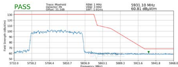
Plot 7-46. Radiated Upper Band Edge Plot MIMO (Peak – UNII Band 3)
