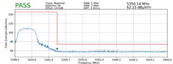
Plot 7-25. Radiated Upper Band Edge Plot MIMO (Peak – UNII Band 2A)
