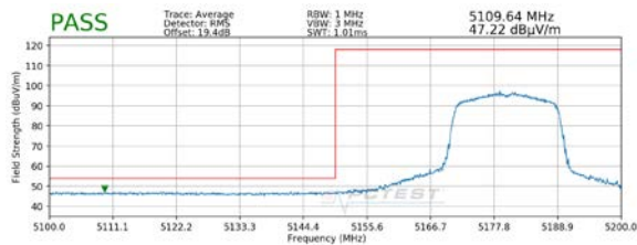
Plot 7-1. Radiated Lower Band Edge Plot SISO ANT1 (Average – UNII Band 1)
