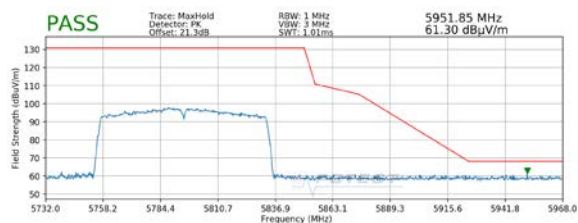
Plot 7-21. Radiated Upper Band Edge Plot SISO ANT1 (Peak – UNII Band 3)
