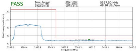
Plot 7-10. Radiated Upper Band Edge Plot SISO ANT1 (Average – UNII Band 2A)
