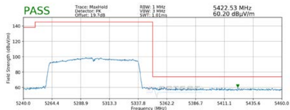
Plot 7-18. Radiated Upper Band Edge Plot SISO ANT1 (Peak – UNII Band 2A)
