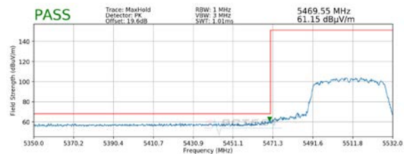
Plot 7-36. Radiated Lower Band Edge Plot MIMO (Peak – UNII Band 2C)
