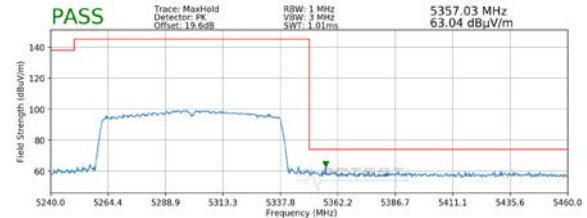
Plot 7-43. Radiated Upper Band Edge Plot MIMO (Peak – UNII Band 2A)
