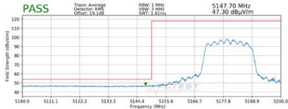
Plot 7-22. Radiated Lower Band Edge Plot MIMO (Average – UNII Band 1)
