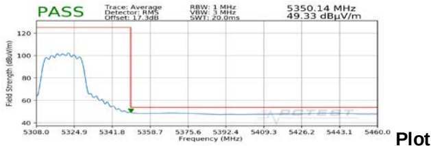
Plot 7-29. Radiated Upper Band Edge Plot MIMO (Average – UNII Band 2A) with Dual Display
