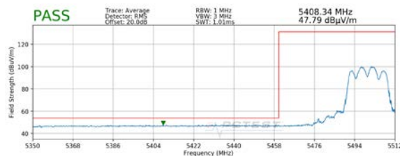
Plot 7-26. Radiated Lower Band Edge Plot MIMO (Average – UNII Band 2C)
