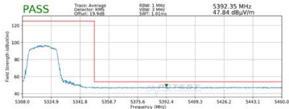
Plot 7-24. Radiated Upper Band Edge Plot MIMO (Average – UNII Band 2A)
