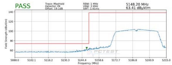
Plot 7-9. Radiated Lower Band Edge Plot SISO ANT1 (Peak – UNII Band 1)
