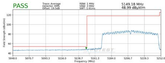
Plot 7-40. Radiated Lower Band Edge Plot MIMO (Average – UNII Band 1)
