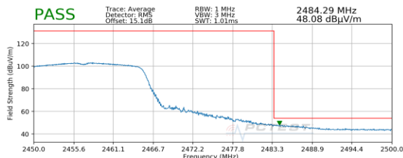
Plot 7-79. Radiated Restricted Upper Band Edge Measurement SISO ANT1 (Average)
