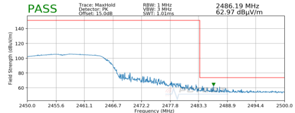
Plot 7-90. Radiated Restricted Upper Band Edge Measurement SISO ANT2 (Peak)
