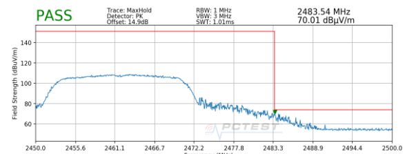
Plot 7-102. Radiated Restricted Upper Band Edge Measurement MIMO (Peak)
