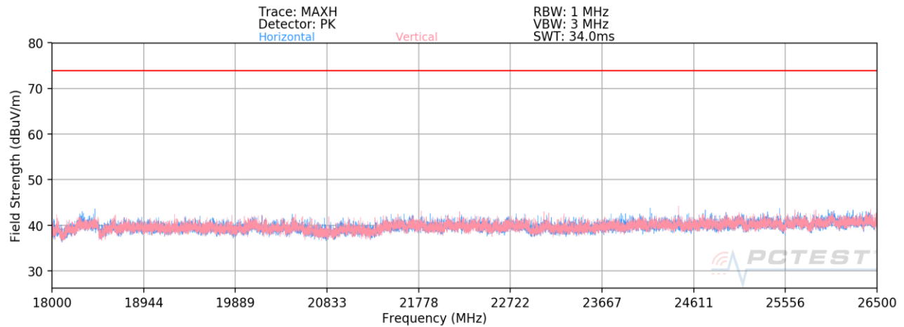
Plot 7-72. Radiated Spurious Plot above 18GHz MIMO/CDD
