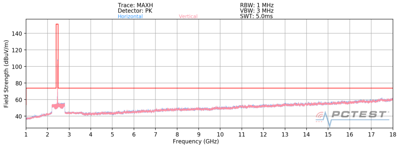
Plot 7-71. Radiated Spurious Plot above 1GHz MIMO/CDD (802.11g – Ch. 11)
