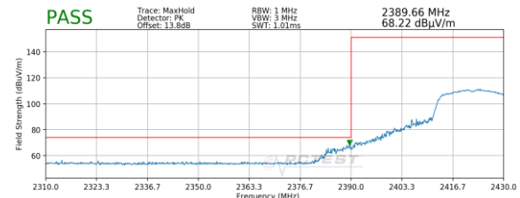
Plot 7-96. Radiated Restricted Lower Band Edge Measurement MIMO (Peak)
