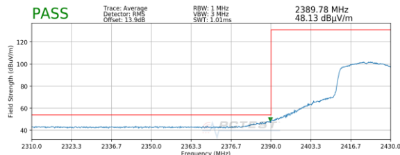
Plot 7-95. Radiated Restricted Lower Band Edge Measurement MIMO (Average)
