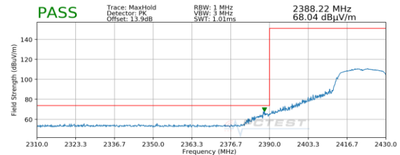
Plot 7-76. Radiated Restricted Lower Band Edge Measurement SISO ANT1 (Peak)
