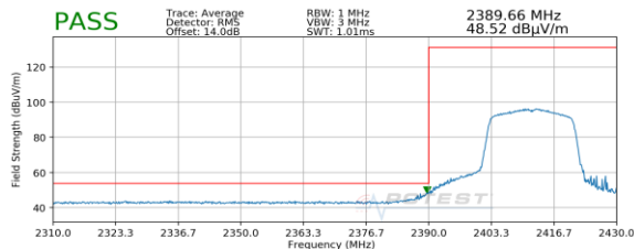
Plot 7-83. Radiated Restricted Lower Band Edge Measurement SISO ANT2 (Average)
