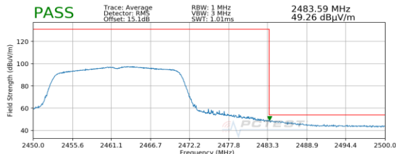
Plot 7-91. Radiated Restricted Upper Band Edge Measurement SISO ANT2 (Average)
