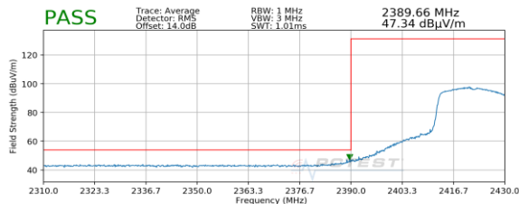
Plot 7-85. Radiated Restricted Lower Band Edge Measurement SISO ANT2 (Average)
