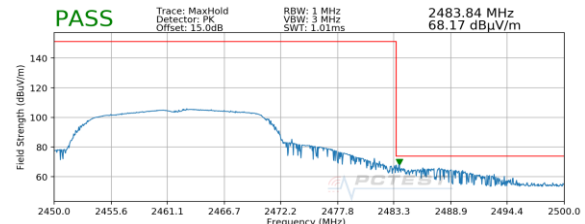
Plot 7-92. Radiated Restricted Upper Band Edge Measurement SISO ANT2 (Peak)
