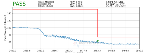
Plot 7-98. Radiated Restricted Upper Band Edge Measurement MIMO (Peak)
