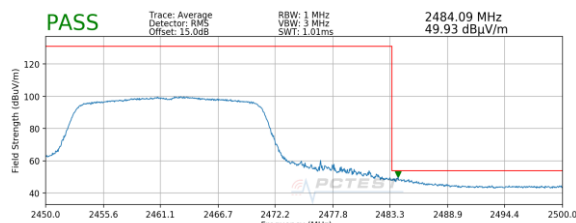
Plot 7-101. Radiated Restricted Upper Band Edge Measurement MIMO (Average)
