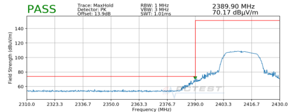
Plot 7-74. Radiated Restricted Lower Band Edge Measurement SISO ANT1 (Peak)
