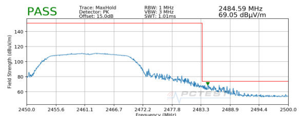
Plot 7-82. Radiated Restricted Upper Band Edge Measurement SISO ANT1 (Peak)
