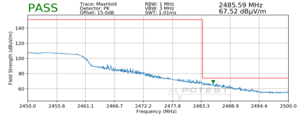
Plot 7-88. Radiated Restricted Upper Band Edge Measurement SISO ANT2 (Peak)
