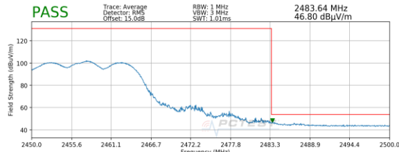
Plot 7-99. Radiated Restricted Upper Band Edge Measurement MIMO (Average)
