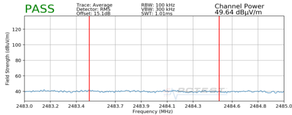
Plot 7-77. Radiated Restricted Upper Band Edge Measurement SISO ANT1 (Average)
