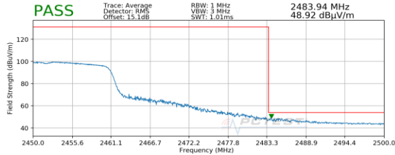
Plot 7-87. Radiated Restricted Upper Band Edge Measurement SISO ANT2 (Average)
