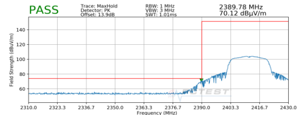
Plot 7-84. Radiated Restricted Lower Band Edge Measurement SISO ANT2 (Peak)
