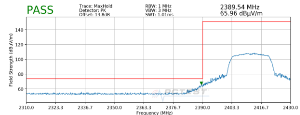
Plot 7-94. Radiated Restricted Lower Band Edge Measurement MIMO (Peak)
