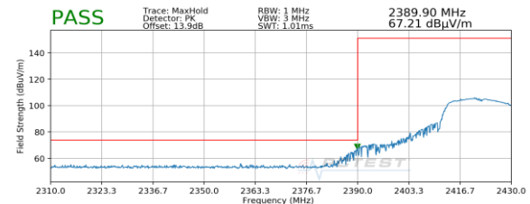
Plot 7-86. Radiated Restricted Lower Band Edge Measurement SISO ANT2 (Peak)
