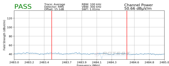
Plot 7-81. Radiated Restricted Upper Band Edge Measurement SISO ANT1 (Average)
