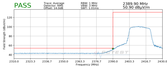
Plot 7-73. Radiated Restricted Lower Band Edge Measurement SISO ANT1 (Average)
