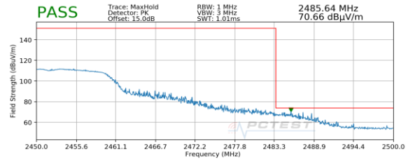
Plot 7-78. Radiated Restricted Upper Band Edge Measurement SISO ANT1 (Peak)
