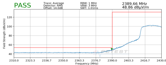
Plot 7-75. Radiated Restricted Lower Band Edge Measurement SISO ANT1 (Average)
