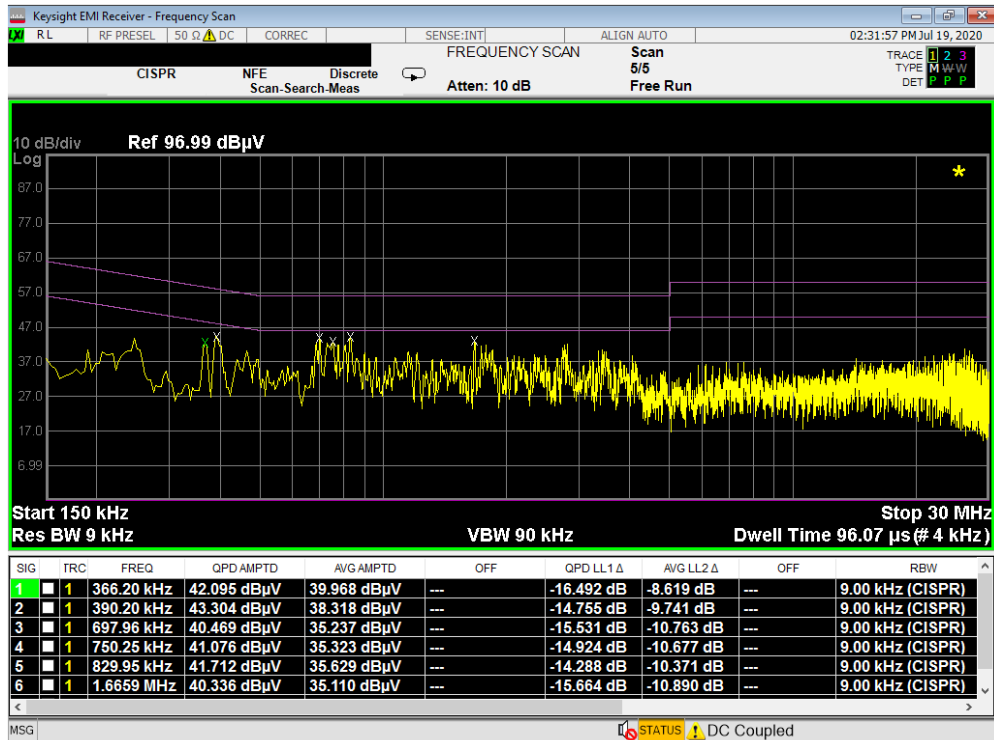
Plot 7-108. Line Conducted Plot with 802.11b (N) with WCP
