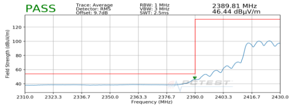
Plot 7-103. Radiated Restricted Lower Band Edge Measurement MIMO with WCP (Average)
