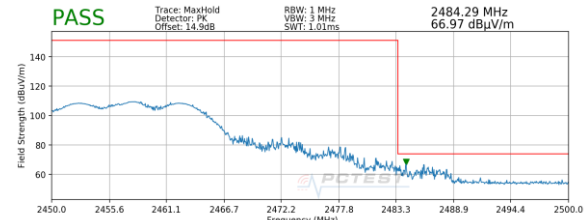
Plot 7-100. Radiated Restricted Upper Band Edge Measurement MIMO (Peak)
