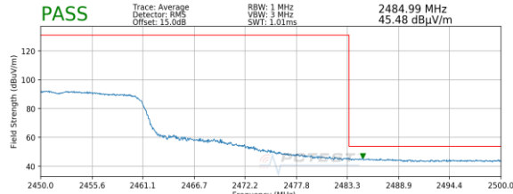
Plot 7-97. Radiated Restricted Upper Band Edge Measurement MIMO (Average)
