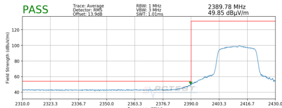
Plot 7-93. Radiated Restricted Lower Band Edge Measurement MIMO (Average)
