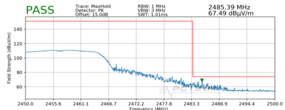
Plot 7-80. Radiated Restricted Upper Band Edge Measurement SISO ANT1 (Peak)
