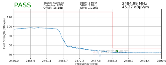
Plot 7-89. Radiated Restricted Upper Band Edge Measurement SISO ANT2 (Average)
