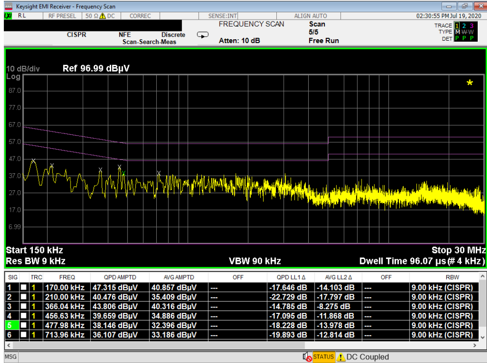
Plot 7-107. Line Conducted Plot with 802.11b (L1) with WCP
