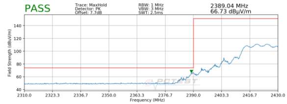
Plot 7-104. Radiated Restricted Lower Band Edge Measurement MIMO with WCP (Peak)
