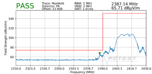
Plot 7-14. Radiated Restricted Lower Band Edge Measurement MIMO (Peak)
