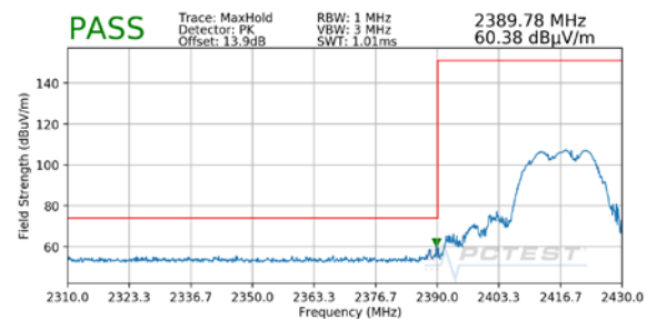
Plot 7-16. Radiated Restricted Lower Band Edge Measurement MIMO (Peak)
