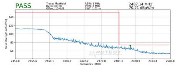
Plot 7-8. Radiated Restricted Upper Band Edge Measurement SISO ANT1 (Peak)
