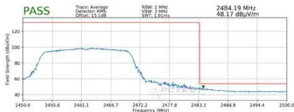
Plot 7-11. Radiated Restricted Upper Band Edge Measurement SISO ANT1 (Average)
