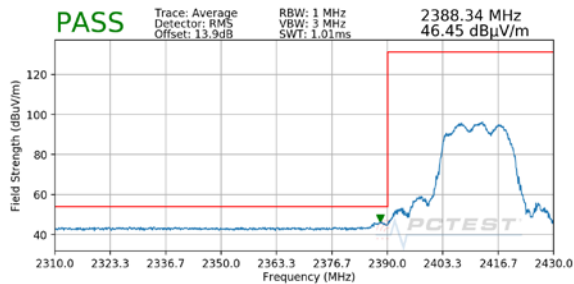
Plot 7-13. Radiated Restricted Lower Band Edge Measurement MIMO (Average)
