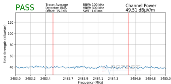
Plot 7-19. Radiated Restricted Upper Band Edge Measurement MIMO (Average)
