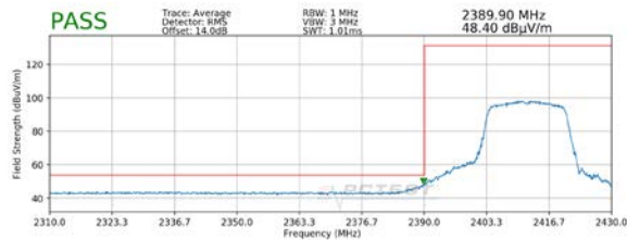
Plot 7-1. Radiated Restricted Lower Band Edge Measurement SISO ANT1 (Average)
