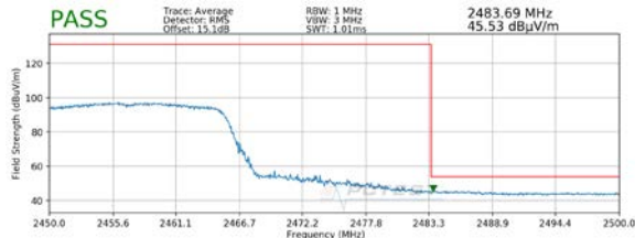
Plot 7-9. Radiated Restricted Upper Band Edge Measurement SISO ANT1 (Average)
