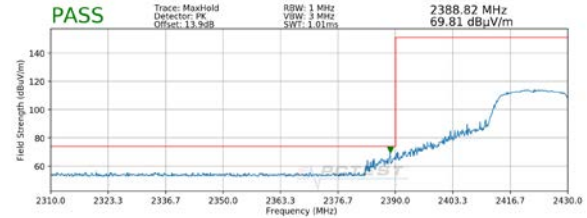
Plot 7-6. Radiated Restricted Lower Band Edge Measurement SISO ANT1 (Peak)
