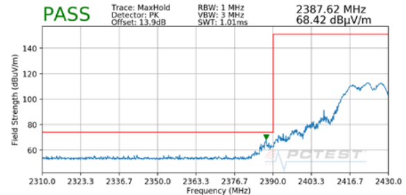
Plot 7-18. Radiated Restricted Lower Band Edge Measurement MIMO (Peak)
