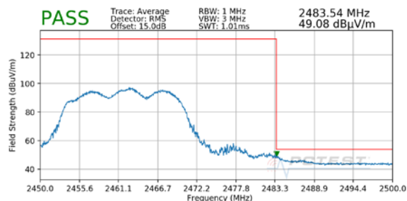
Plot 7-23. Radiated Restricted Upper Band Edge Measurement MIMO (Average)
