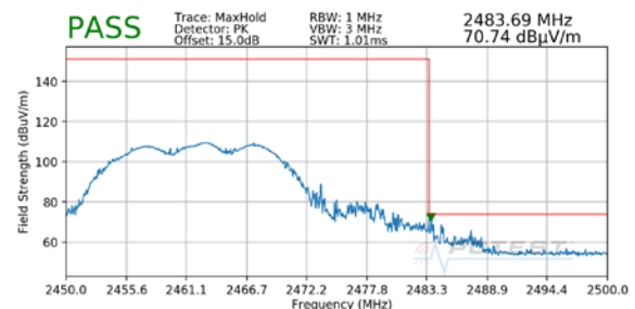
Plot 7-24. Radiated Restricted Upper Band Edge Measurement MIMO (Peak)
