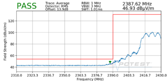
Plot 7-17. Radiated Restricted Lower Band Edge Measurement MIMO (Average)
