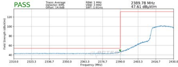
Plot 7-5. Radiated Restricted Lower Band Edge Measurement SISO ANT1 (Average)
