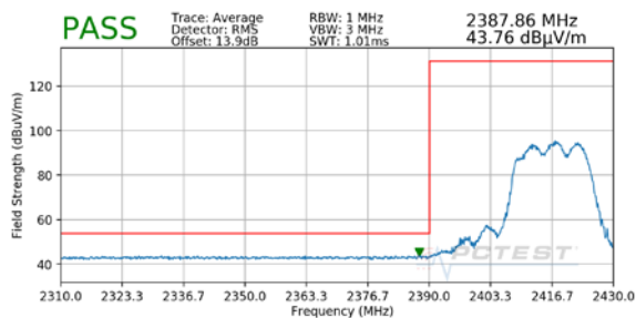
Plot 7-15. Radiated Restricted Lower Band Edge Measurement MIMO (Average)
