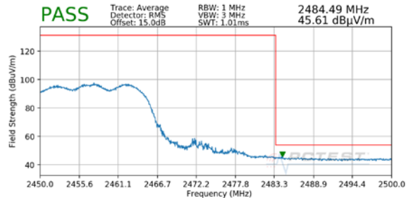
Plot 7-21. Radiated Restricted Upper Band Edge Measurement MIMO (Average)
