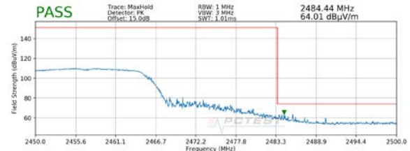
Plot 7-10. Radiated Restricted Upper Band Edge Measurement SISO ANT1 (Peak)
