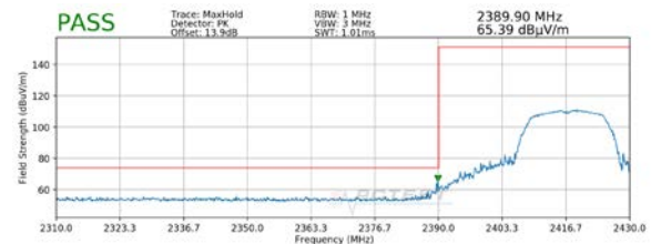
Plot 7-4. Radiated Restricted Lower Band Edge Measurement SISO ANT1 (Peak)
