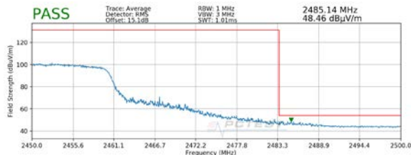
Plot 7-7. Radiated Restricted Upper Band Edge Measurement SISO ANT1 (Average)
