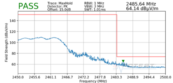
Plot 7-22. Radiated Restricted Upper Band Edge Measurement MIMO(Peak)
