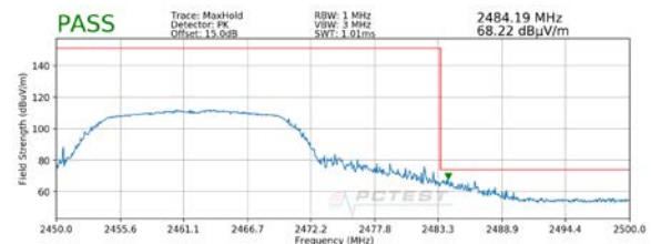
Plot 7-12. Radiated Restricted Upper Band Edge Measurement SISO ANT1 (Peak)
