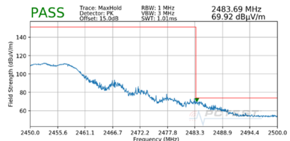
Plot 7-20. Radiated Restricted Upper Band Edge Measurement MIMO (Peak)
