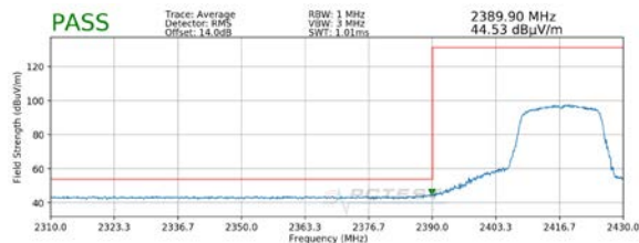
Plot 7-3. Radiated Restricted Lower Band Edge Measurement SISO ANT1 (Average)
