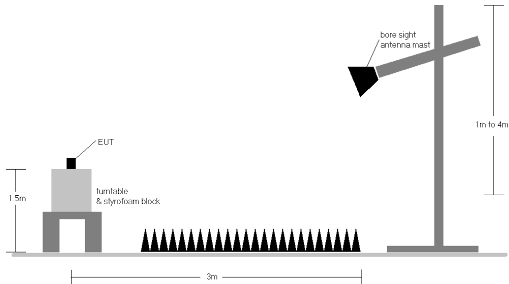
Figure 7-1. Test Instrument & Measurement Setup
