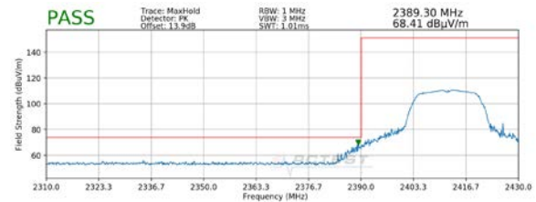
Plot 7-2. Radiated Restricted Lower Band Edge Measurement SISO ANT1 (Peak)
