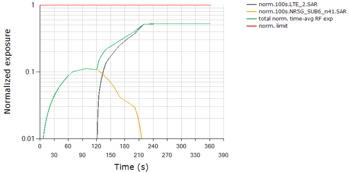
Total Normalized Time-averaged RF Exposure Tech: LTE, Band 2 / Tech: NR5G SUB6, Band n41
