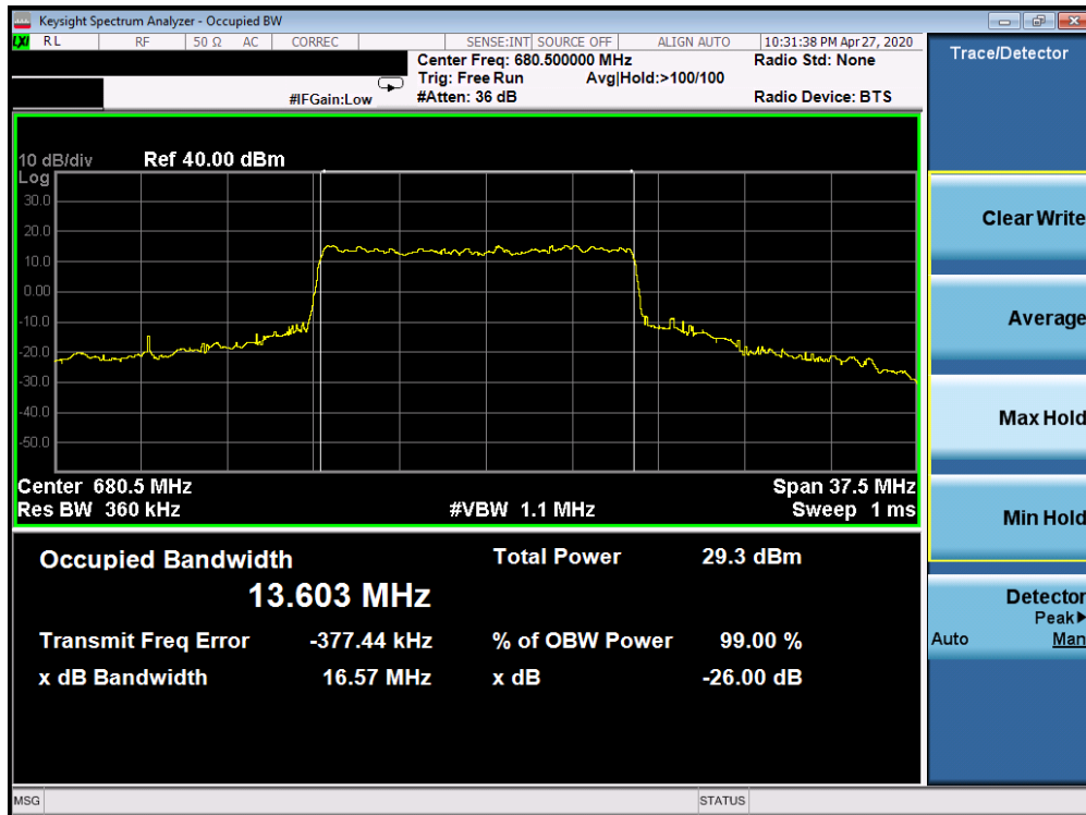
Plot 7-122. Occupied Bandwidth Plot (5G sub6 n71 - 15.0MHz 64-QAM - Full RB Configuration)
