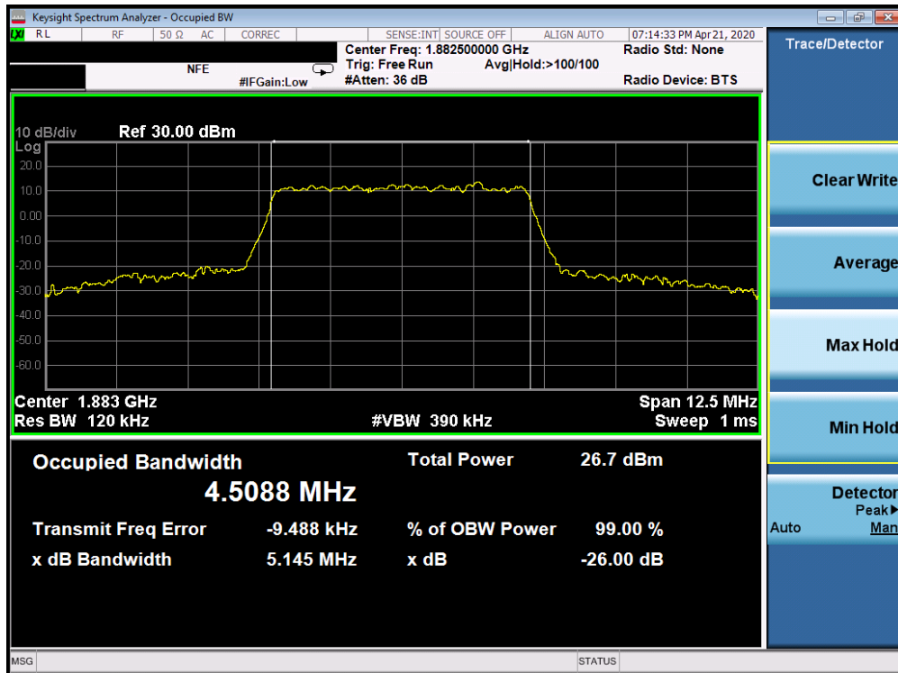
Plot 7-173. Occupied Bandwidth Plot (5G sub6 n25/2 - 5.0MHz 256-QAM - Full RB Configuration)
