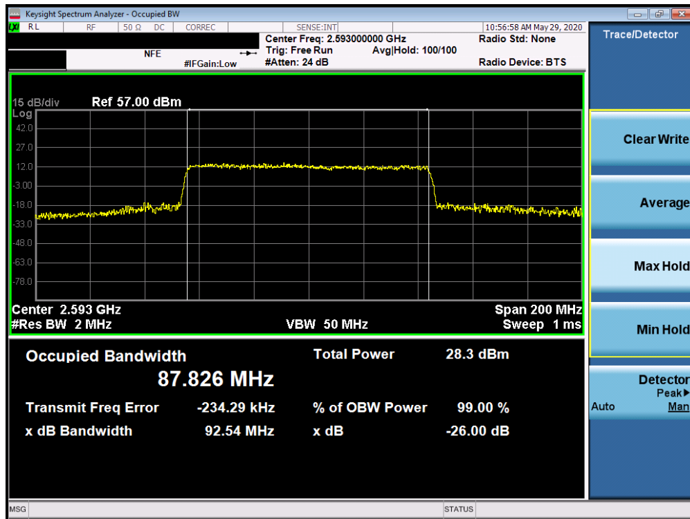
Plot 7-217. Occupied Bandwidth Plot (5G sub6 n41 – 90.0MHz 64-QAM - Full RB Configuration)
