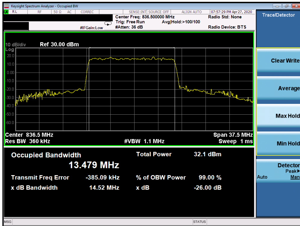
Plot 7-139. Occupied Bandwidth Plot (5G sub6 n5 – 15.0MHz BPSK - Full RB Configuration)
