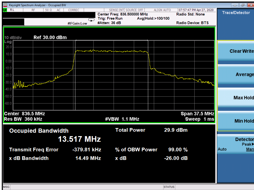
Plot 7-140. Occupied Bandwidth Plot (5G sub6 n5 – 15.0MHz QPSK - Full RB Configuration)
