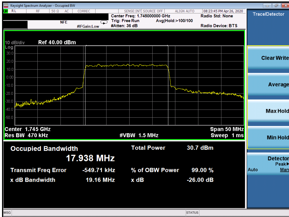
Plot 7-165. Occupied Bandwidth Plot (5G sub6 n66 - 20.0MHz QPSK - Full RB Configuration)
