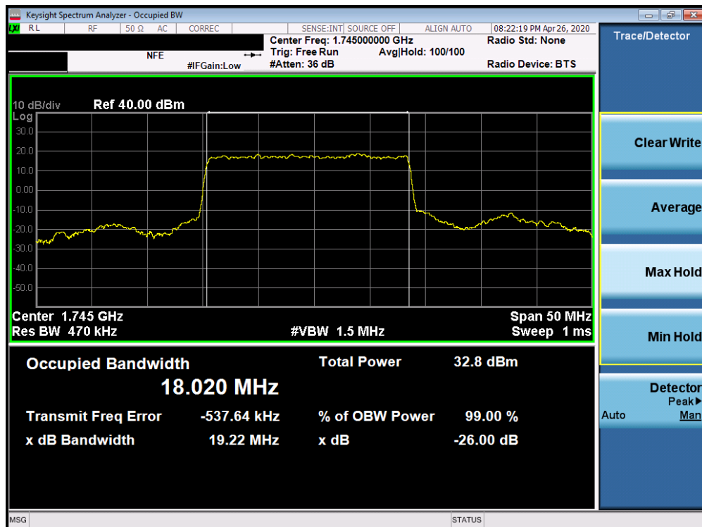
Plot 7-164. Occupied Bandwidth Plot (5G sub6 n66 - 20.0MHz BPSK - Full RB Configuration)
