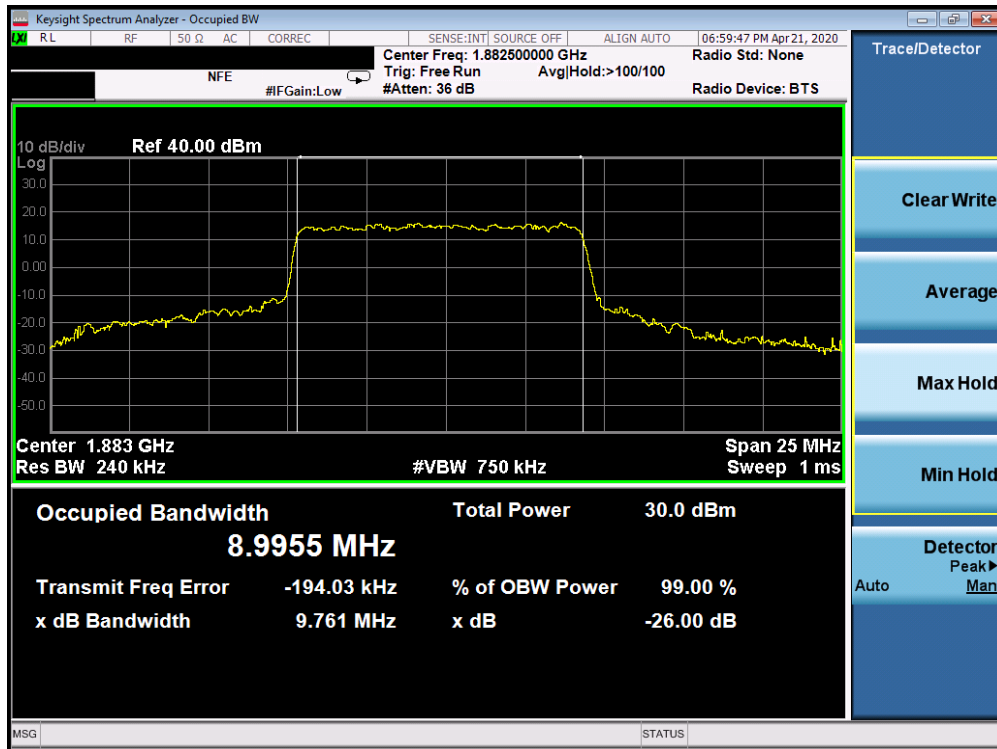
Plot 7-177. Occupied Bandwidth Plot (5G sub6 n25/2 - 10.0MHz 64-QAM - Full RB Configuration)
