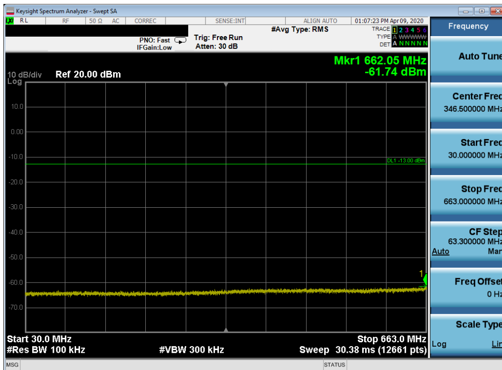
Plot 7-227. Conducted Spurious Plot (Band 71 - 10.0MHz QPSK - RB Size 1, RB Offset 0 - Mid Channel)
