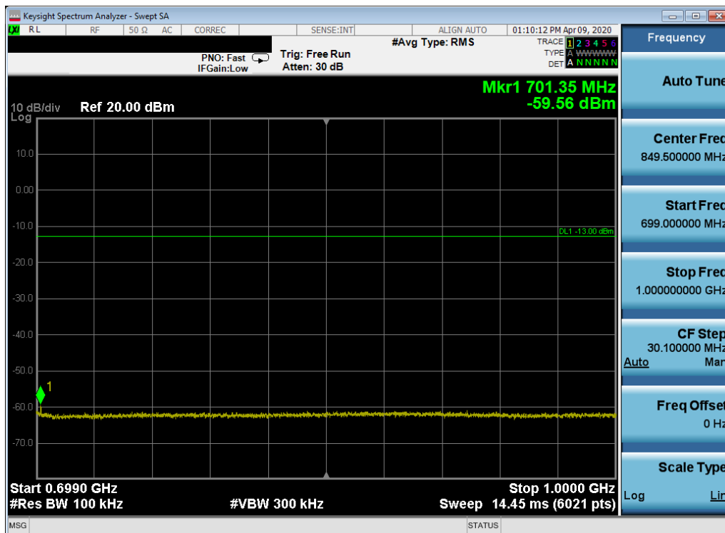
Plot 7-231. Conducted Spurious Plot (Band 71 - 10.0MHz QPSK - RB Size 1, RB Offset 0 - High Channel)
