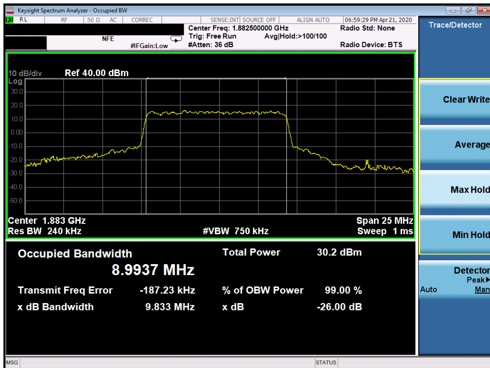
Plot 7-176. Occupied Bandwidth Plot (5G sub6 n25/2 - 10.0MHz 16-QAM - Full RB Configuration)
