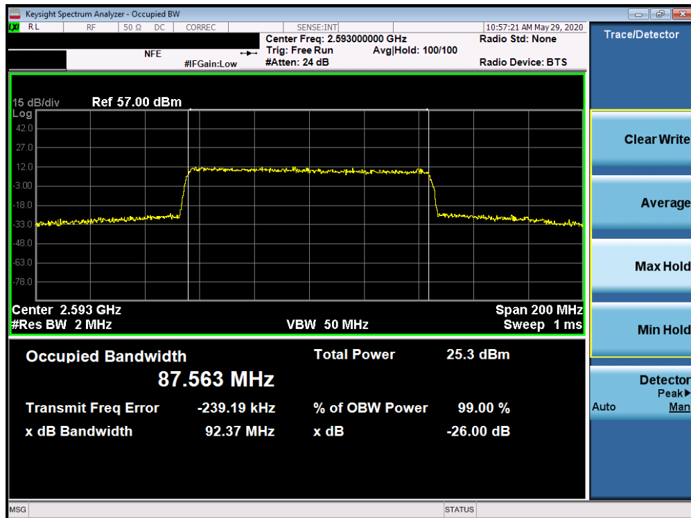
Plot 7-218. Occupied Bandwidth Plot (5G sub6 n41 – 90.0MHz 256-QAM - Full RB Configuration)
