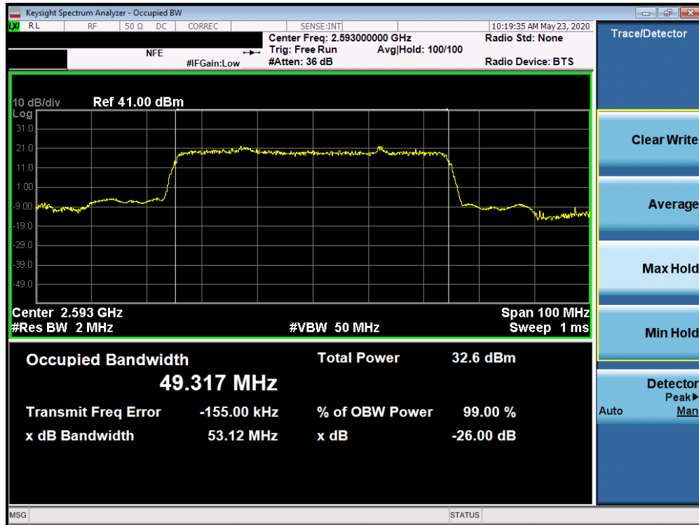
Plot 7-199. Occupied Bandwidth Plot (5G sub6 n41 - 50.0MHz BPSK - Full RB Configuration)
