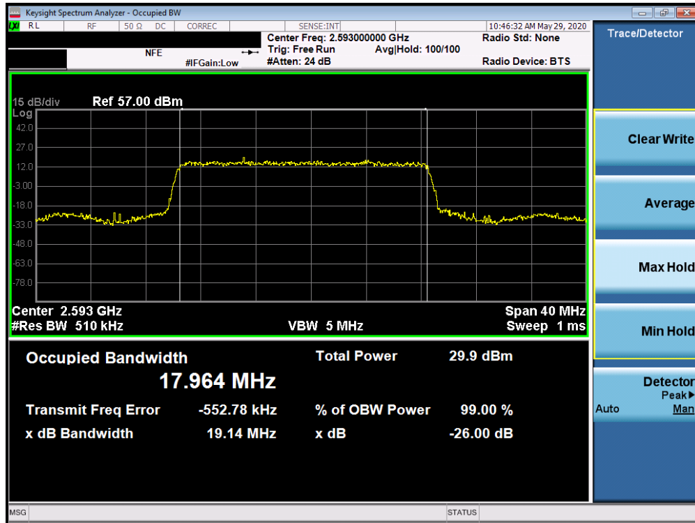
Plot 7-189. Occupied Bandwidth Plot (5G sub6 n41 - 20.0MHz BPSK - Full RB Configuration)
