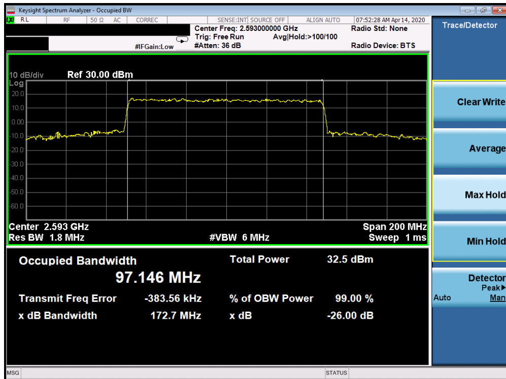
Plot 7-220. Occupied Bandwidth Plot (5G sub6 n41 - 100.0MHz QPSK - Full RB Configuration)
