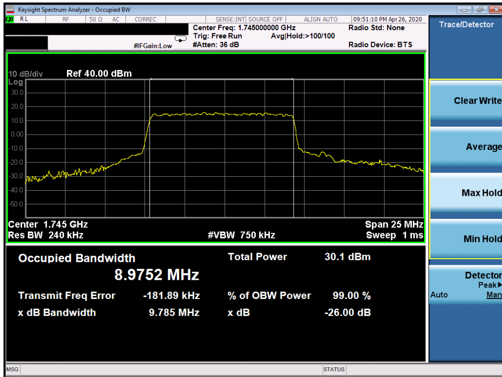
Plot 7-155. Occupied Bandwidth Plot (5G sub6 n66 - 10.0MHz QPSK - Full RB Configuration)
