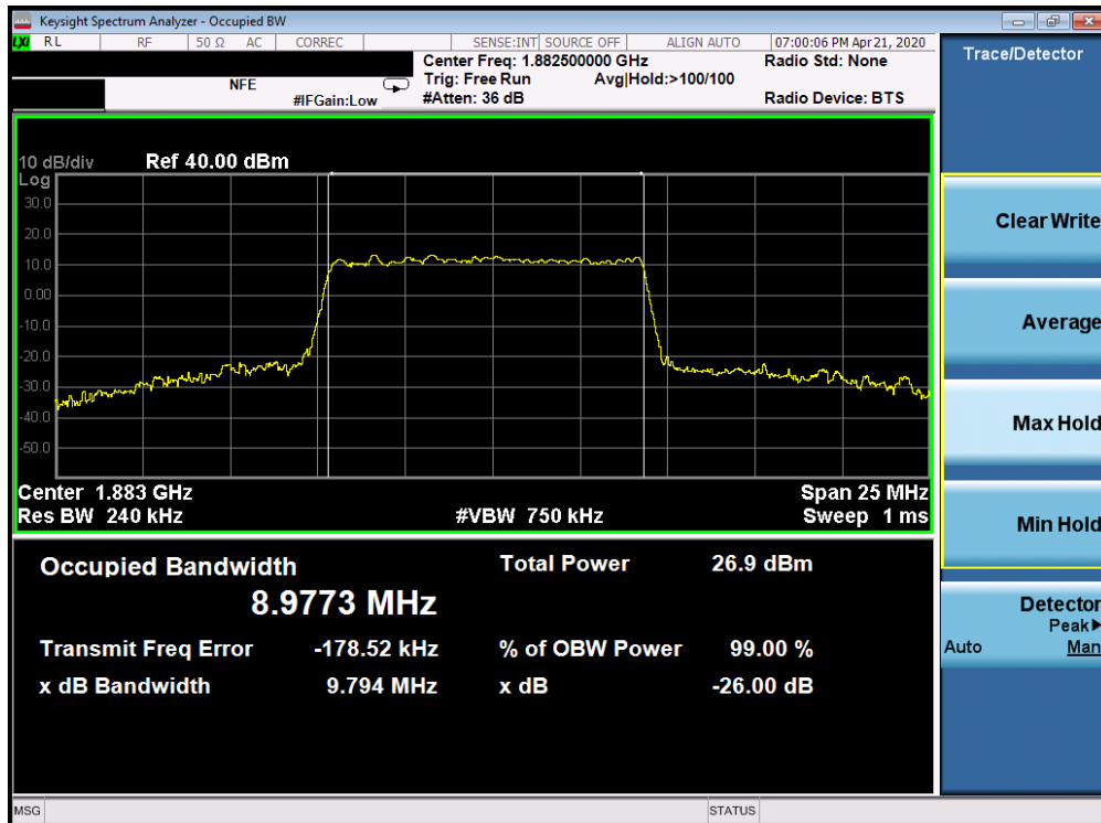
Plot 7-178. Occupied Bandwidth Plot (5G sub6 n25/2 - 10.0MHz 256-QAM - Full RB Configuration)
