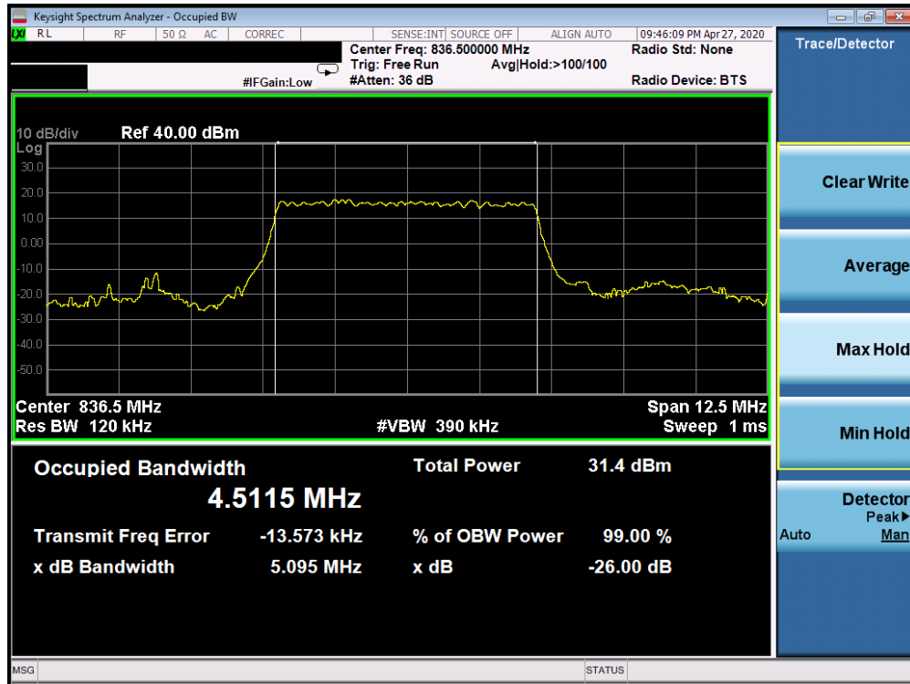
Plot 7-129. Occupied Bandwidth Plot (5G sub6 n5 - 5.0MHz BPSK - Full RB Configuration)
