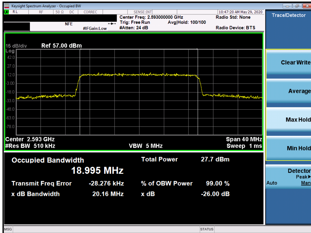
Plot 7-190. Occupied Bandwidth Plot (5G sub6 n41 - 20.0MHz QPSK - Full RB Configuration)
