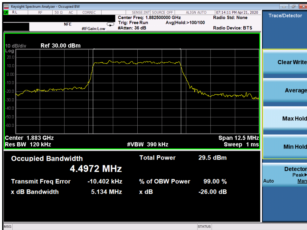
Plot 7-172. Occupied Bandwidth Plot (5G sub6 n25/2 - 5.0MHz 64-QAM - Full RB Configuration)
