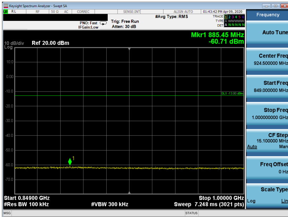
Plot 7-246. Conducted Spurious Plot (Band 5 - 10.0MHz QPSK - RB Size 1, RB Offset 0 - Low Channel)
