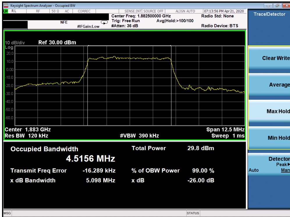
Plot 7-171. Occupied Bandwidth Plot (5G sub6 n25/2 - 5.0MHz 16-QAM - Full RB Configuration)
