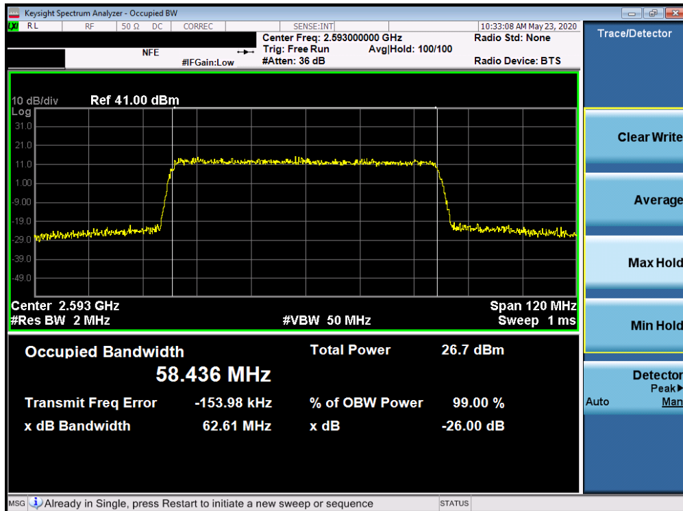
Plot 7-208. Occupied Bandwidth Plot (5G sub6 n41 - 60.0MHz 256-QAM - Full RB Configuration)
