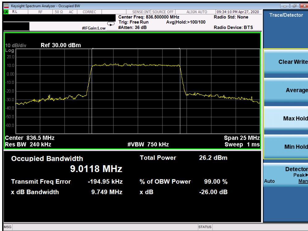
Plot 7-138. Occupied Bandwidth Plot (5G sub6 n5 - 10.0MHz 256-QAM - Full RB Configuration)
