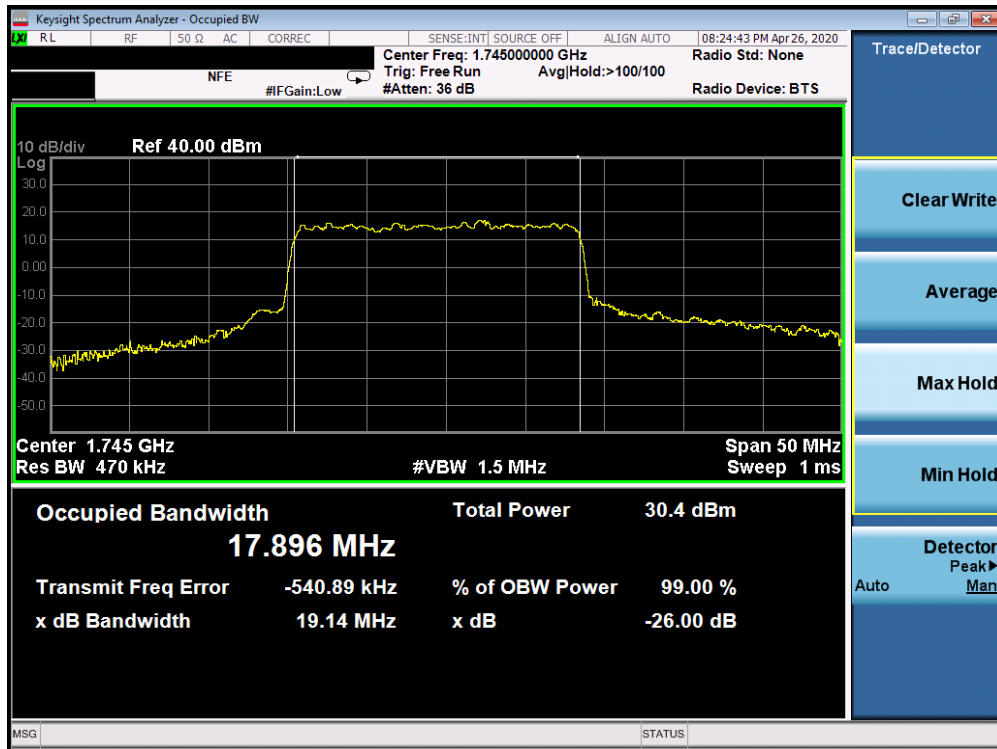
Plot 7-167. Occupied Bandwidth Plot (5G sub6 n66 - 20.0MHz 64-QAM - Full RB Configuration)
