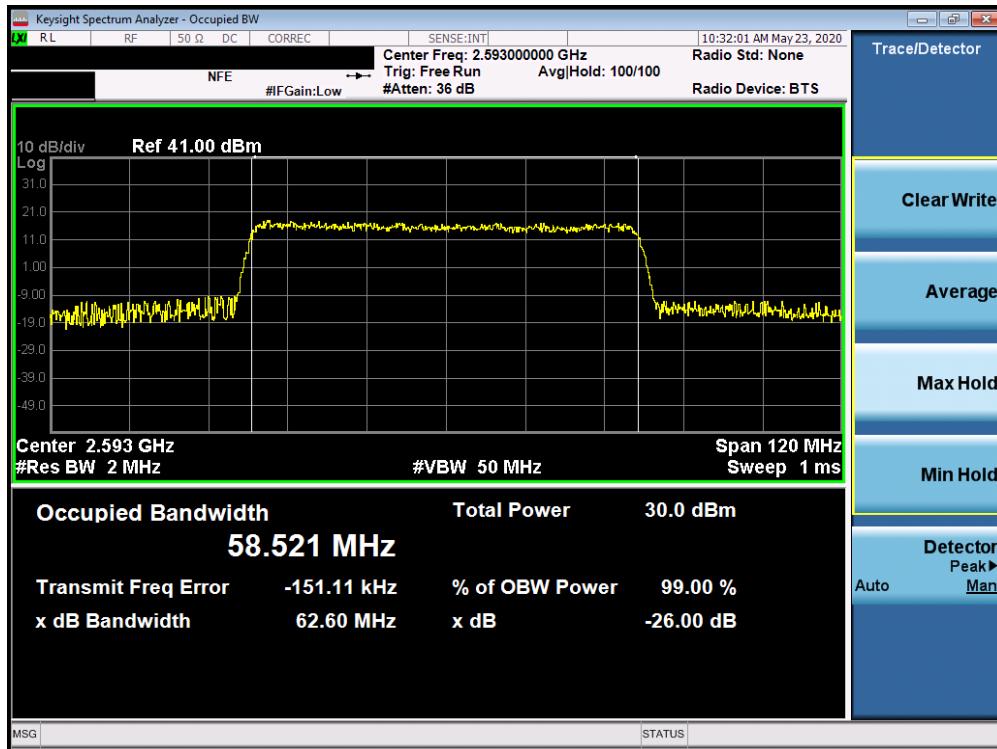
Plot 7-205. Occupied Bandwidth Plot (5G sub6 n41 - 60.0MHz QPSK - Full RB Configuration)
