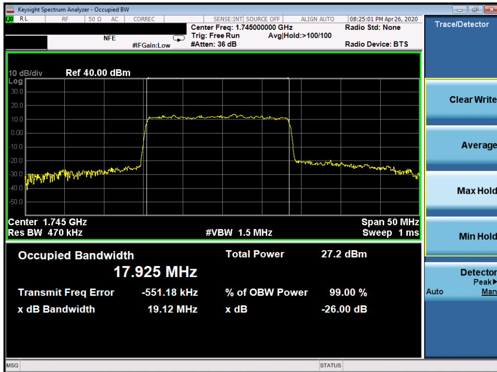
Plot 7-168. Occupied Bandwidth Plot (5G sub6 n66 - 20.0MHz 256-QAM - Full RB Configuration)
