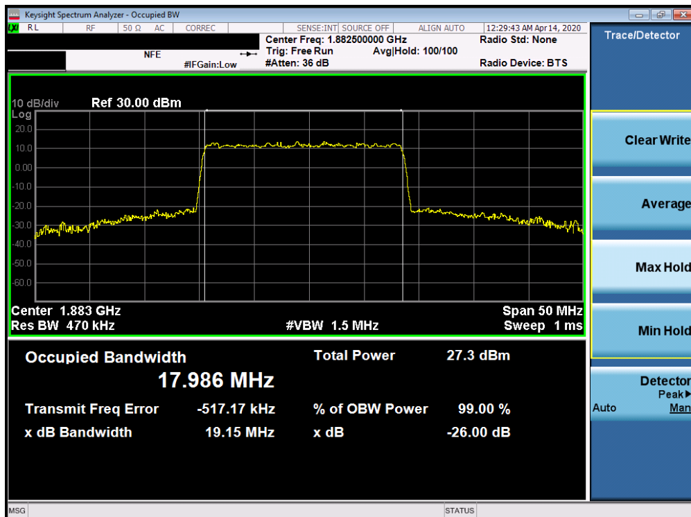
Plot 7-188. Occupied Bandwidth Plot (5G sub6 n25/2 - 20.0MHz 256-QAM - Full RB Configuration)
