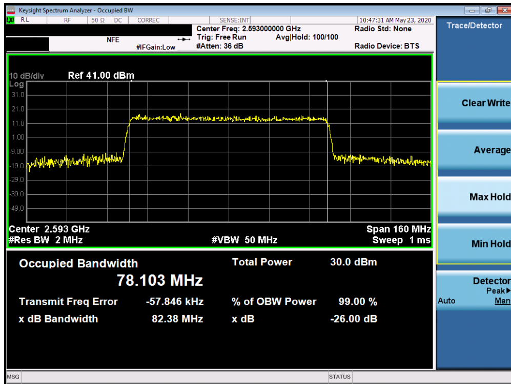
Plot 7-211. Occupied Bandwidth Plot (5G sub6 n41 - 80.0MHz 16-QAM - Full RB Configuration)
