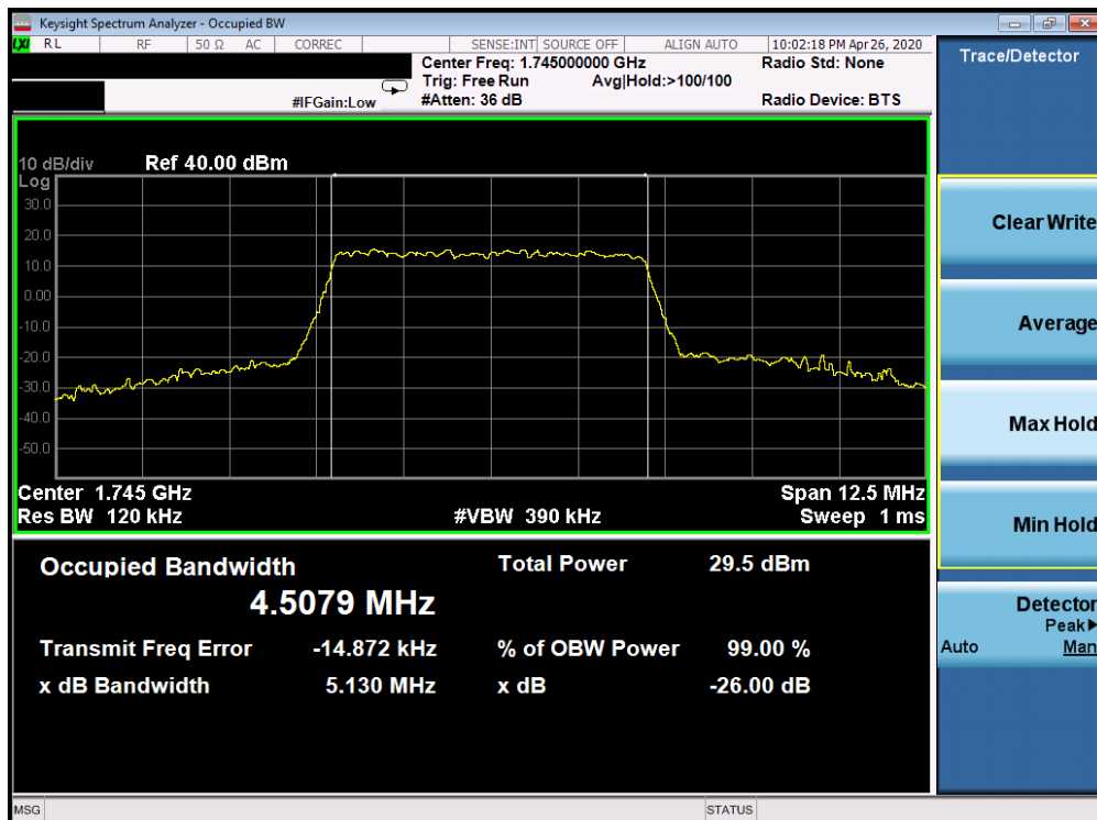
Plot 7-152. Occupied Bandwidth Plot (5G sub6 n66 - 5.0MHz 64-QAM - Full RB Configuration)
