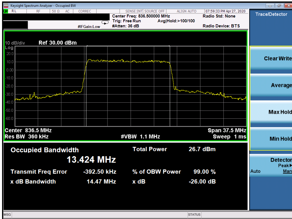
Plot 7-143. Occupied Bandwidth Plot (5G sub6 n5 – 15.0MHz 256-QAM - Full RB Configuration)
