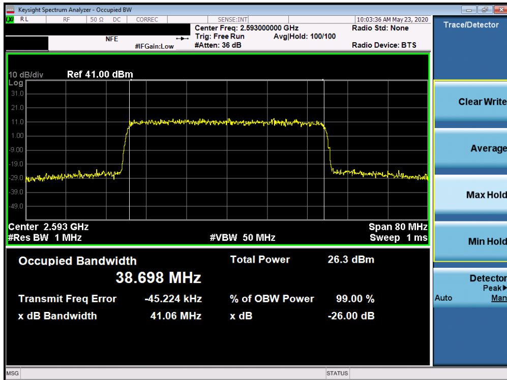
Plot 7-198. Occupied Bandwidth Plot (5G sub6 n41 - 40.0MHz 256-QAM - Full RB Configuration)
