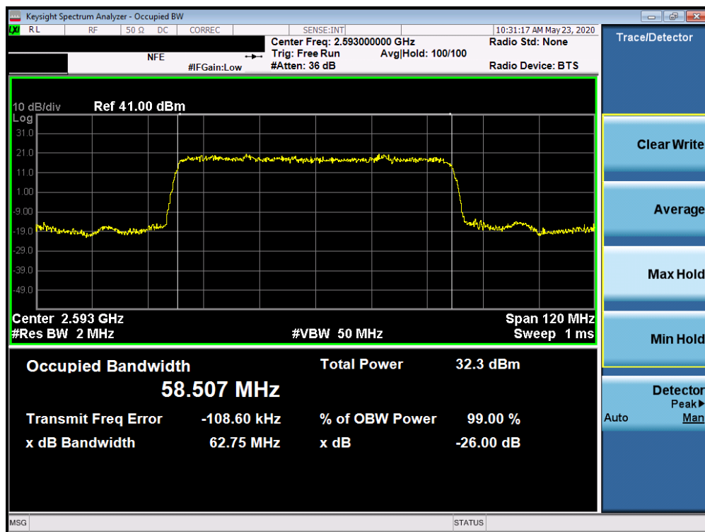
Plot 7-204. Occupied Bandwidth Plot (5G sub6 n41 – 60.0MHz BPSK - Full RB Configuration)
