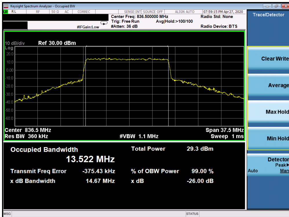
Plot 7-142. Occupied Bandwidth Plot (5G sub6 n5 – 15.0MHz 64-QAM - Full RB Configuration)
