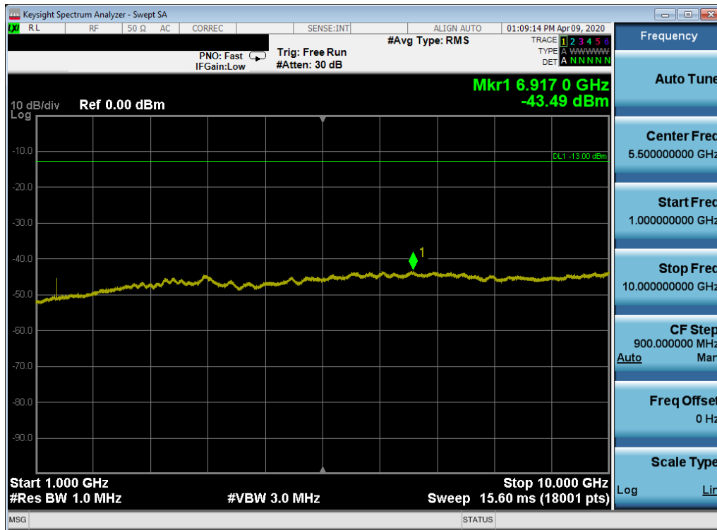
Plot 7-226. Conducted Spurious Plot (Band 71 - 10.0MHz QPSK - RB Size 1, RB Offset 0 - Low Channel)
