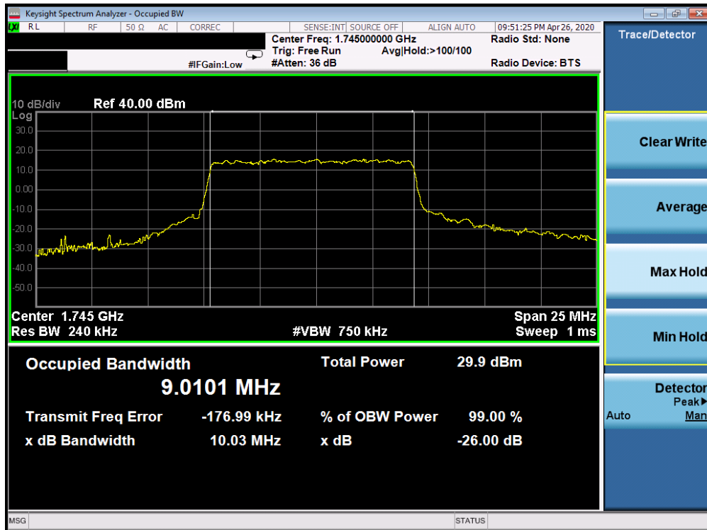
Plot 7-156. Occupied Bandwidth Plot (5G sub6 n66 - 10.0MHz 16-QAM - Full RB Configuration)
