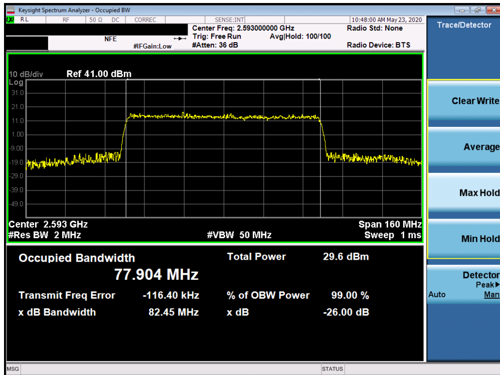
Plot 7-212. Occupied Bandwidth Plot (5G sub6 n41 - 80.0MHz 64-QAM - Full RB Configuration)
