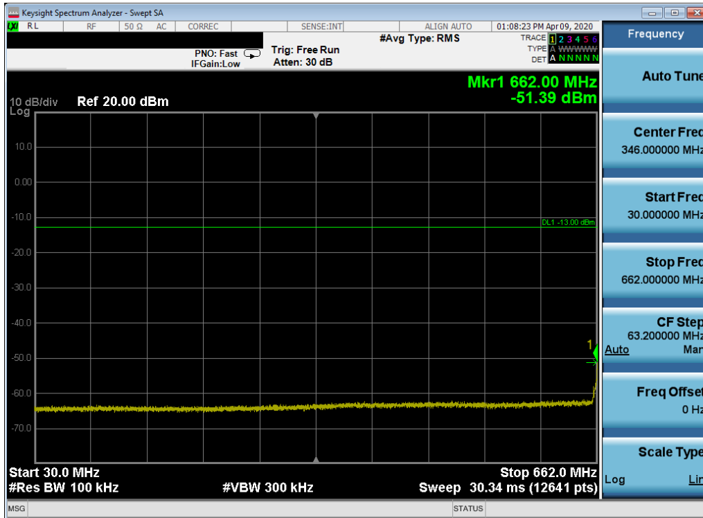
Plot 7-224. Conducted Spurious Plot (Band 71 - 10.0MHz QPSK - RB Size 1, RB Offset 0 - Low Channel)
