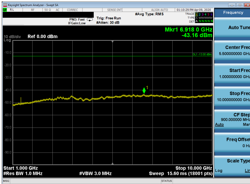
Plot 7-232. Conducted Spurious Plot (Band 71 - 10.0MHz QPSK - RB Size 1, RB Offset 0 - High Channel)
