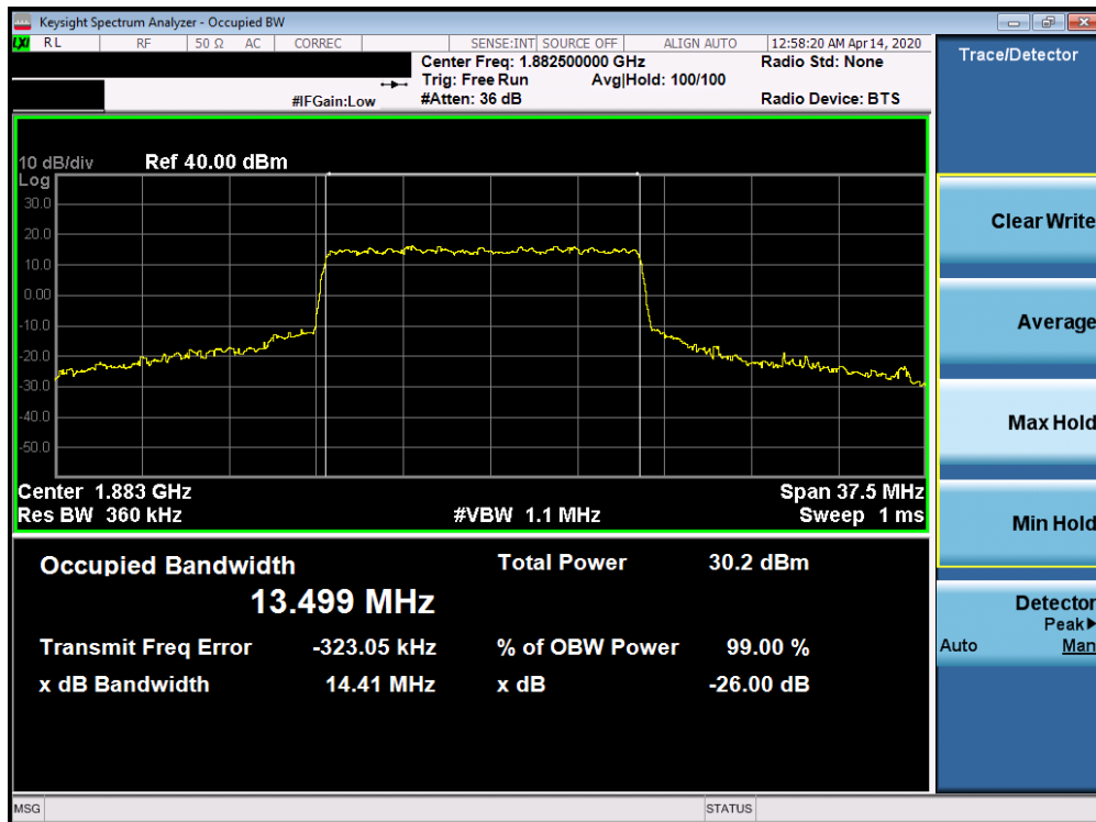
Plot 7-180. Occupied Bandwidth Plot (5G sub6 n25/2 - 15.0MHz QPSK - Full RB Configuration)
