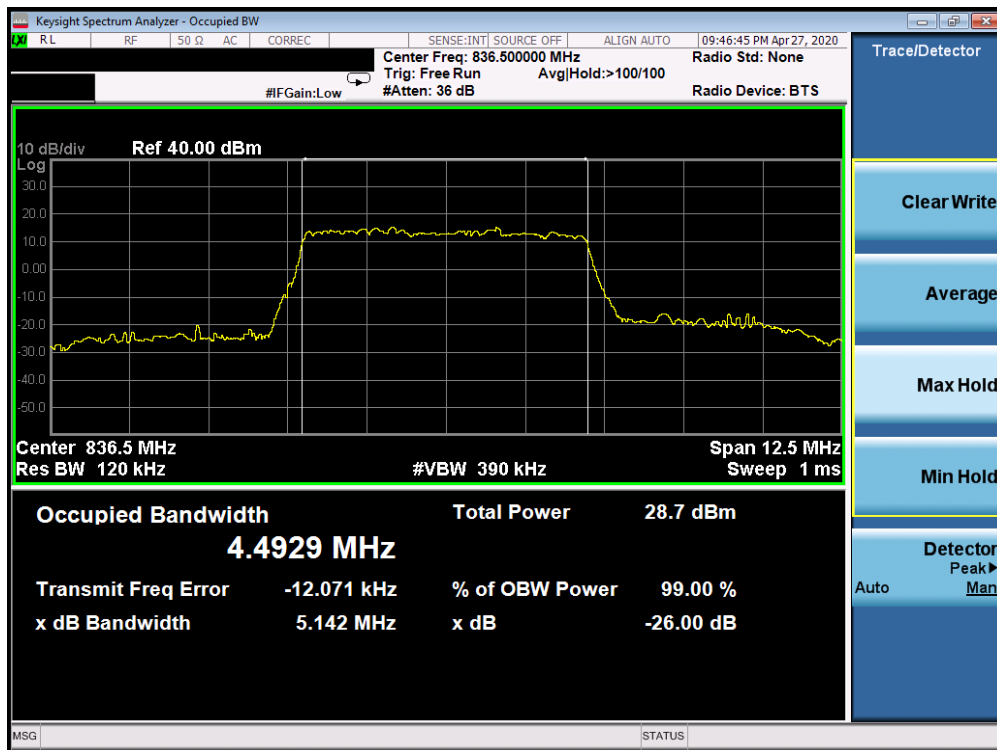
Plot 7-132. Occupied Bandwidth Plot (5G sub6 n5 - 5.0MHz 64-QAM - Full RB Configuration)
