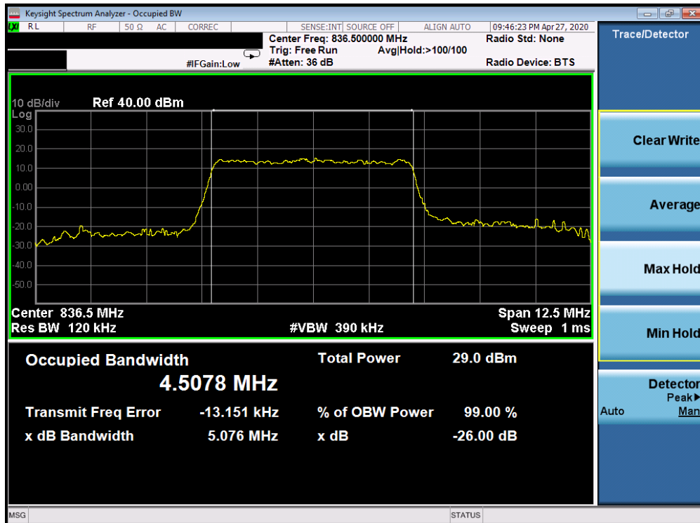
Plot 7-130. Occupied Bandwidth Plot (5G sub6 n5 - 5.0MHz QPSK - Full RB Configuration)
