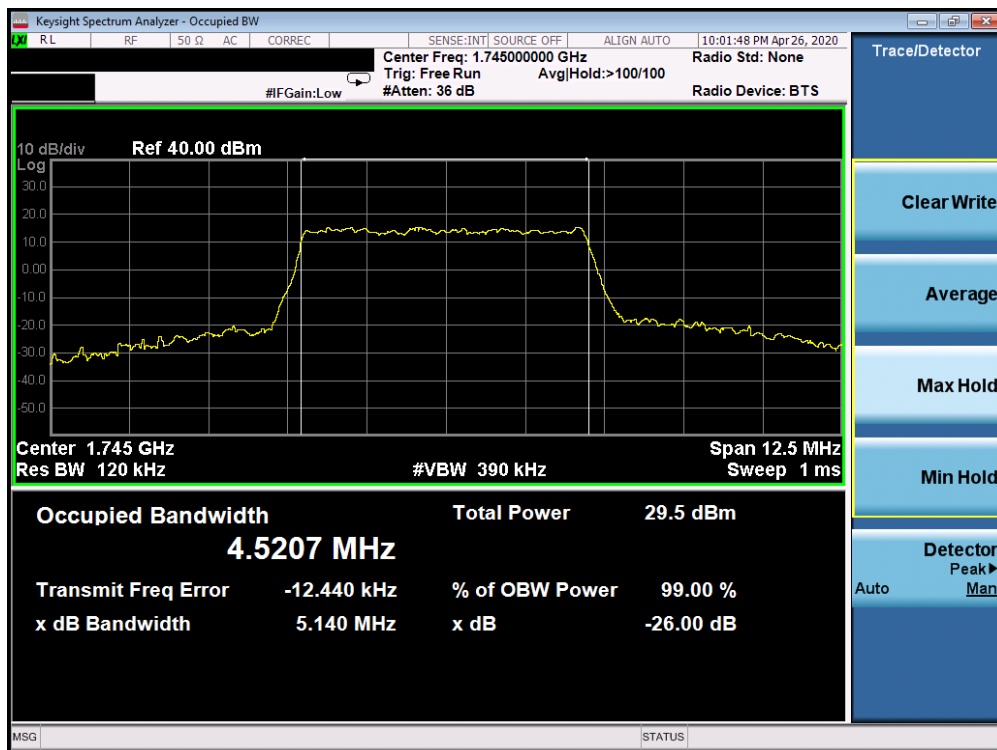
Plot 7-150. Occupied Bandwidth Plot (5G sub6 n66 - 5.0MHz QPSK - Full RB Configuration)
