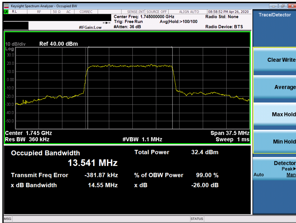
Plot 7-159. Occupied Bandwidth Plot (5G sub6 n66 - 15.0MHz BPSK - Full RB Configuration)
