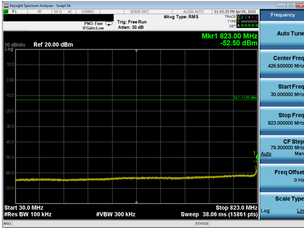
Plot 7-245. Conducted Spurious Plot (Band 5 - 10.0MHz QPSK - RB Size 1, RB Offset 0 - Low Channel)
