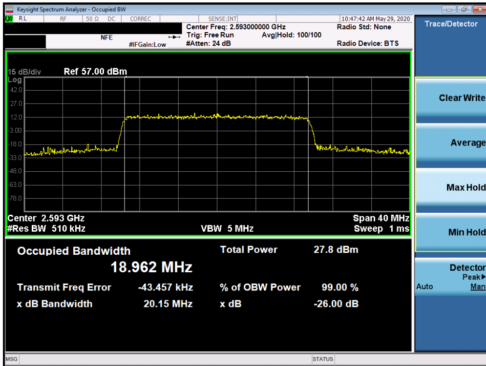
Plot 7-191. Occupied Bandwidth Plot (5G sub6 n41 - 20.0MHz 16-QAM - Full RB Configuration)
