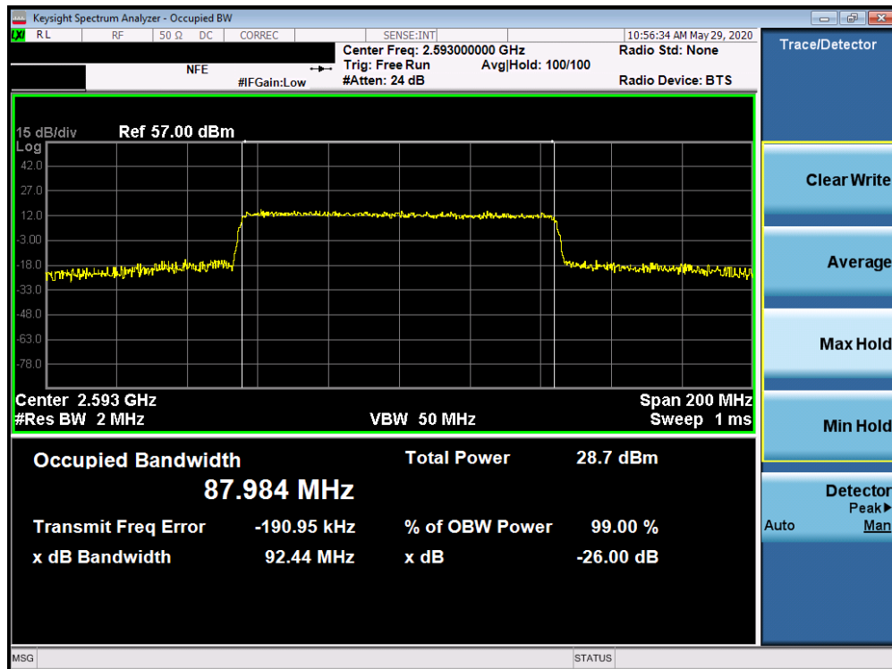
Plot 7-216. Occupied Bandwidth Plot (5G sub6 n41 – 90.0MHz 16-QAM - Full RB Configuration)
