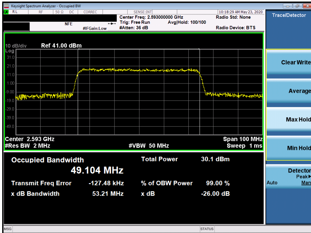
Plot 7-202. Occupied Bandwidth Plot (5G sub6 n41 - 50.0MHz 64-QAM - Full RB Configuration)
