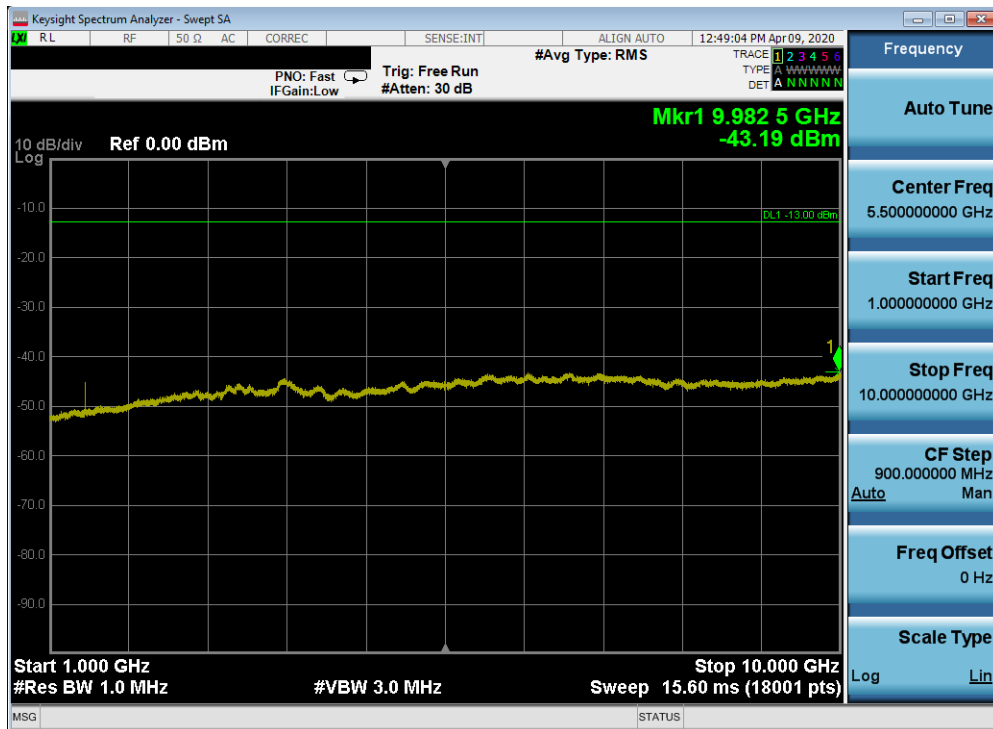
Plot 7-238. Conducted Spurious Plot (Band 12/17 - 10.0MHz QPSK - RB Size 1, RB Offset 0 - Mid Channel)
