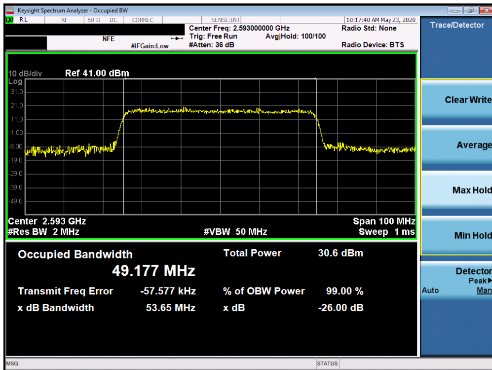
Plot 7-200. Occupied Bandwidth Plot (5G sub6 n41 - 50.0MHz QPSK - Full RB Configuration)
