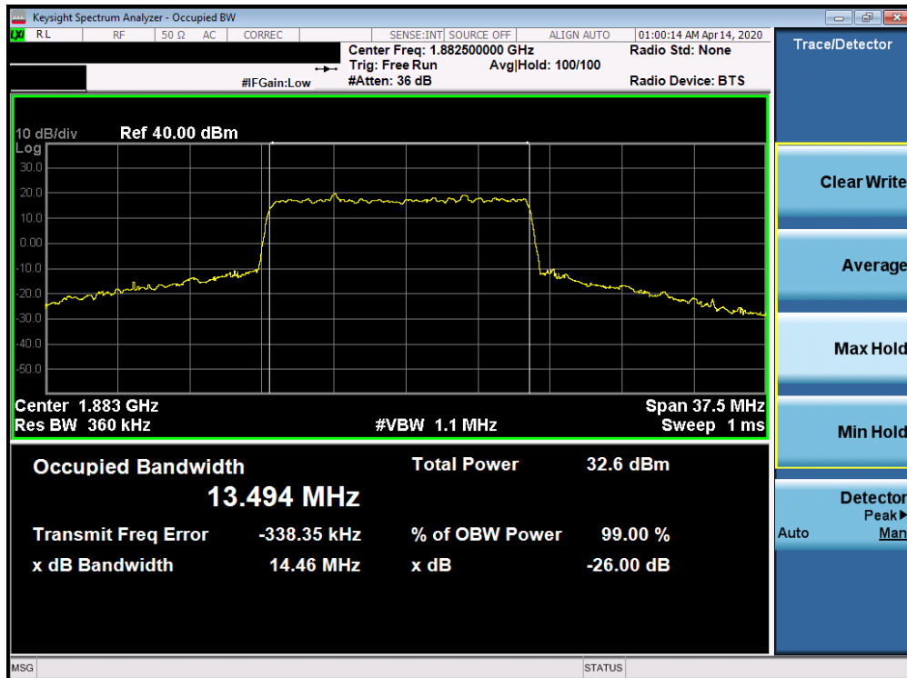
Plot 7-182. Occupied Bandwidth Plot (5G sub6 n25/2 - 15.0MHz 64-QAM - Full RB Configuration)
