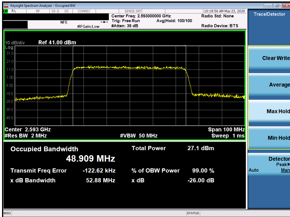
Plot 7-203. Occupied Bandwidth Plot (5G sub6 n41 - 50.0MHz 256-QAM - Full RB Configuration)
