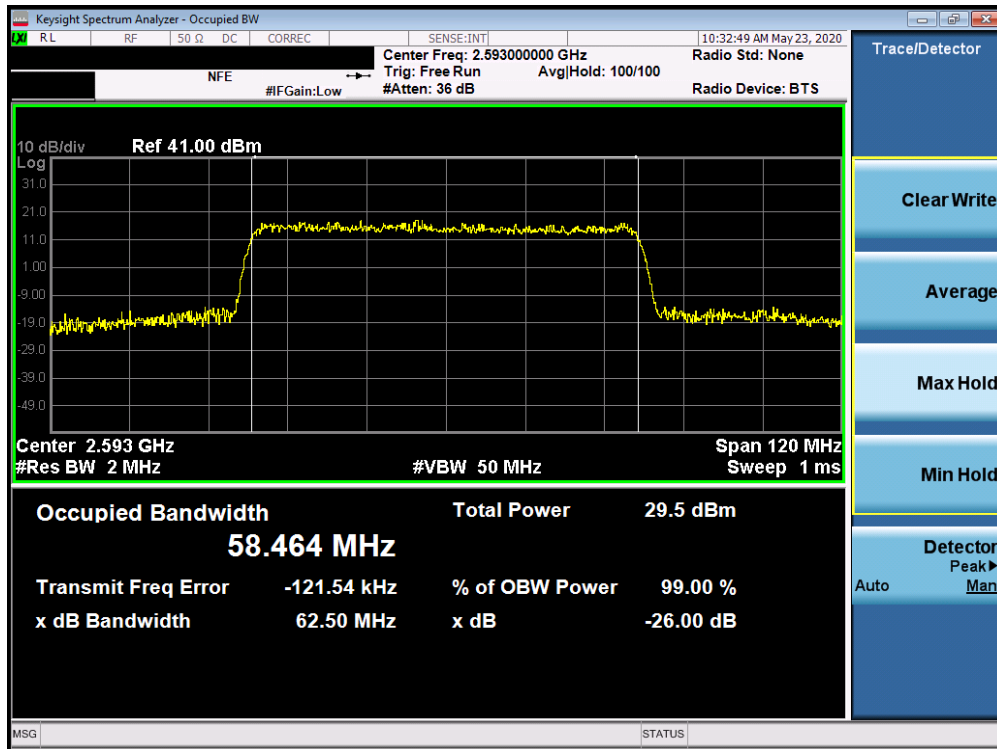
Plot 7-207. Occupied Bandwidth Plot (5G sub6 n41 - 60.0MHz 64-QAM - Full RB Configuration)
