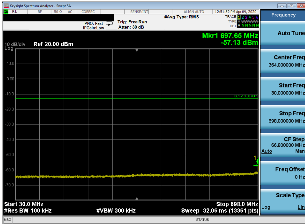
Plot 7-239. Conducted Spurious Plot (Band 12/17 - 10.0MHz QPSK - RB Size 1, RB Offset 0 - High Channel)
