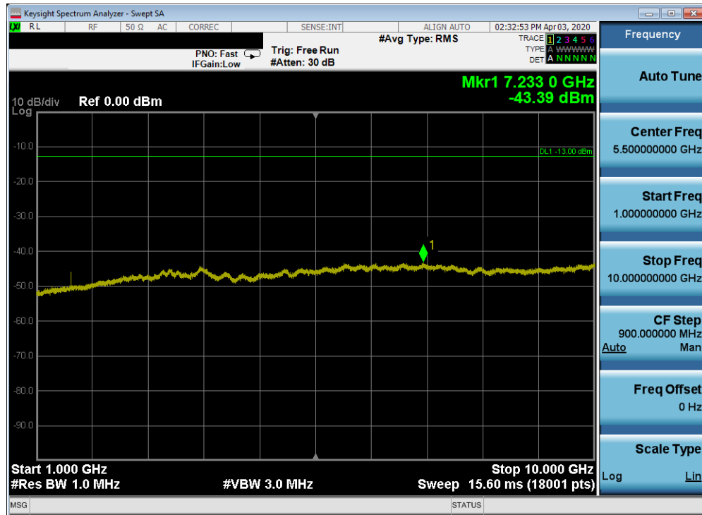
Plot 7-244. Conducted Spurious Plot (Band 13 - 10.0MHz QPSK - RB Size 1, RB Offset 0 - Mid Channel)
