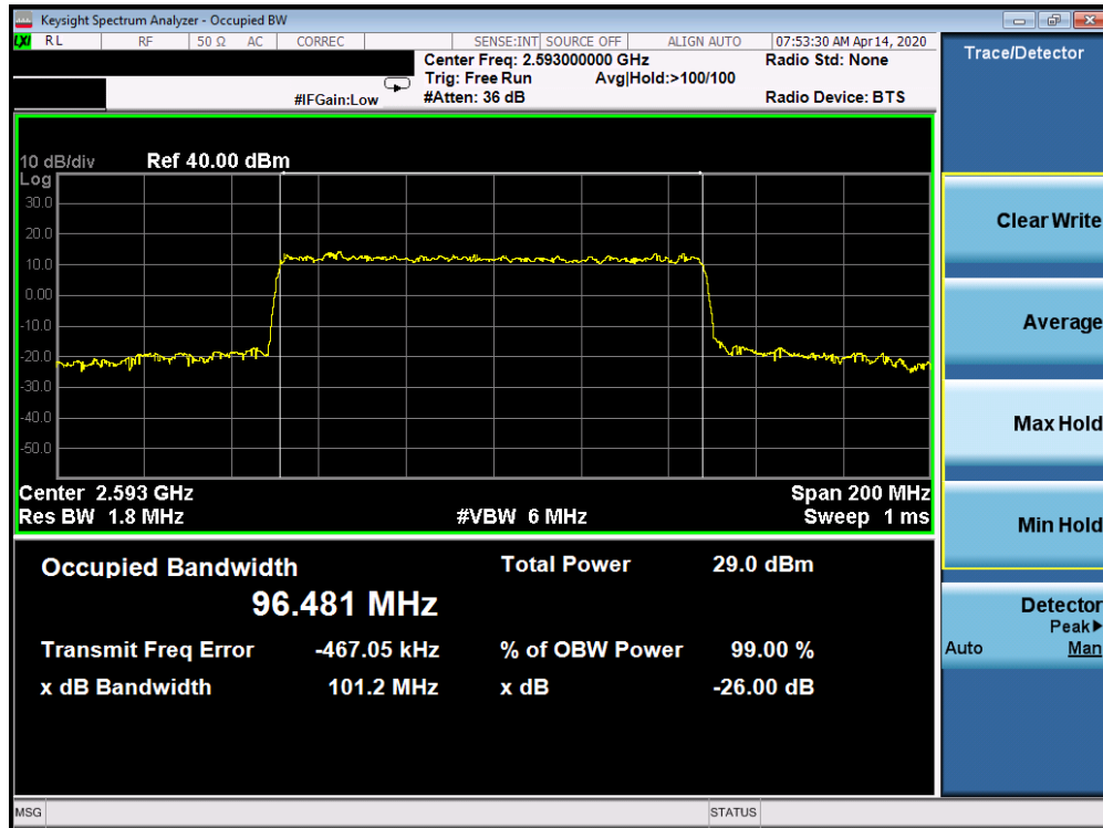
Plot 7-223. Occupied Bandwidth Plot (5G sub6 n41 - 100.0MHz 256-QAM - Full RB Configuration)
