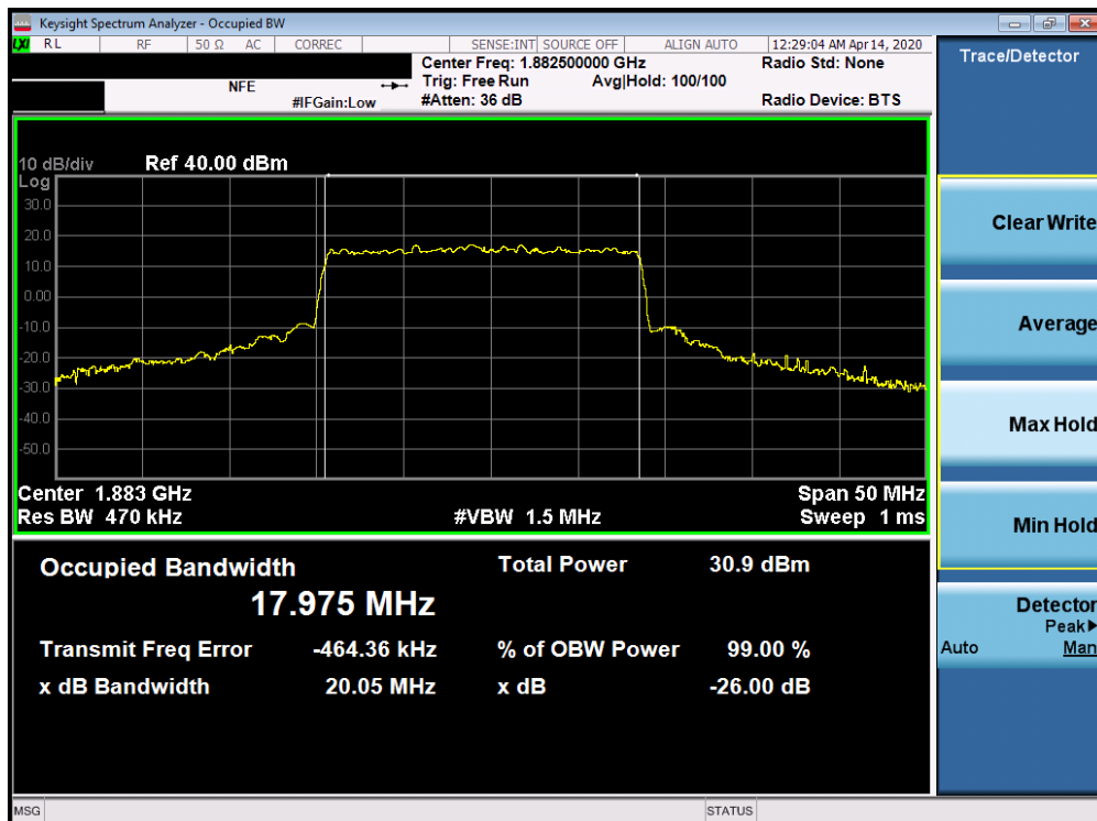
Plot 7-186. Occupied Bandwidth Plot (5G sub6 n25/2 - 20.0MHz 16-QAM - Full RB Configuration)
