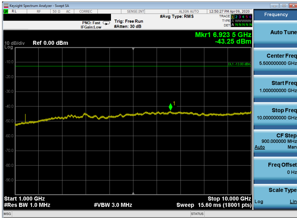
Plot 7-235. Conducted Spurious Plot (Band 12/17 - 10.0MHz QPSK - RB Size 1, RB Offset 0 - Low Channel)
