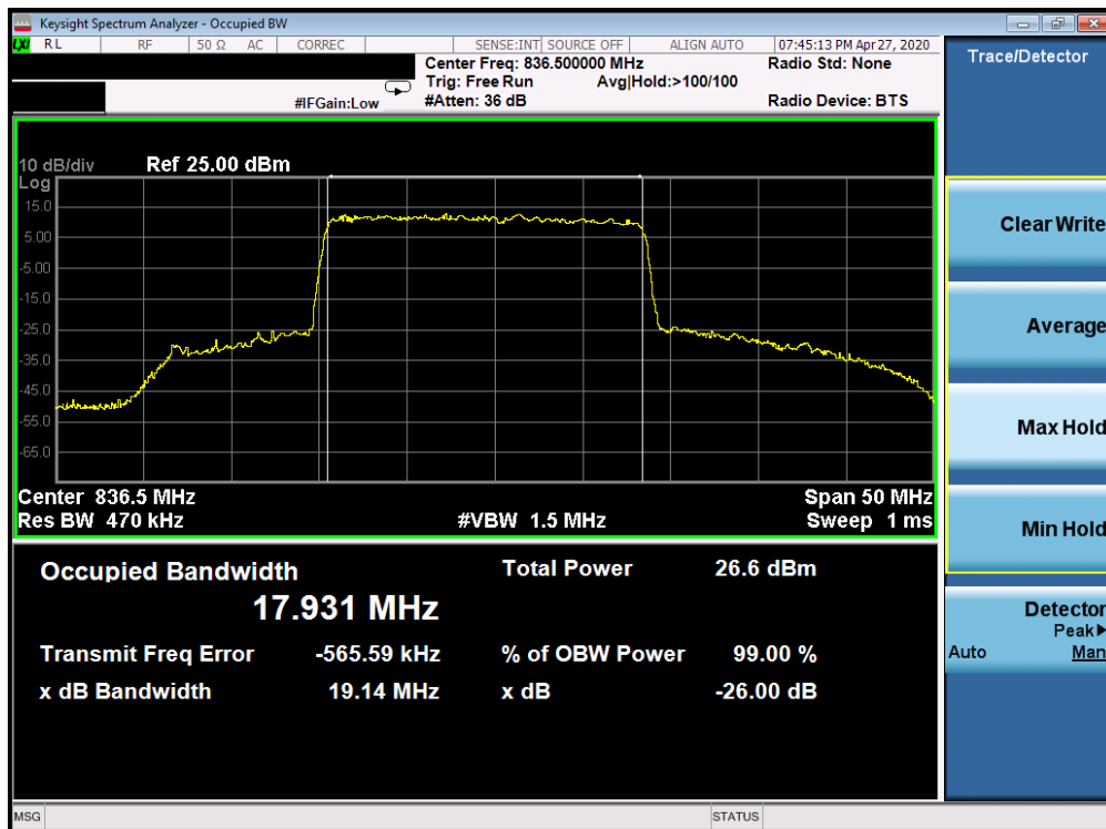
Plot 7-148. Occupied Bandwidth Plot (5G sub6 n5 - 20.0MHz 256-QAM - Full RB Configuration)
