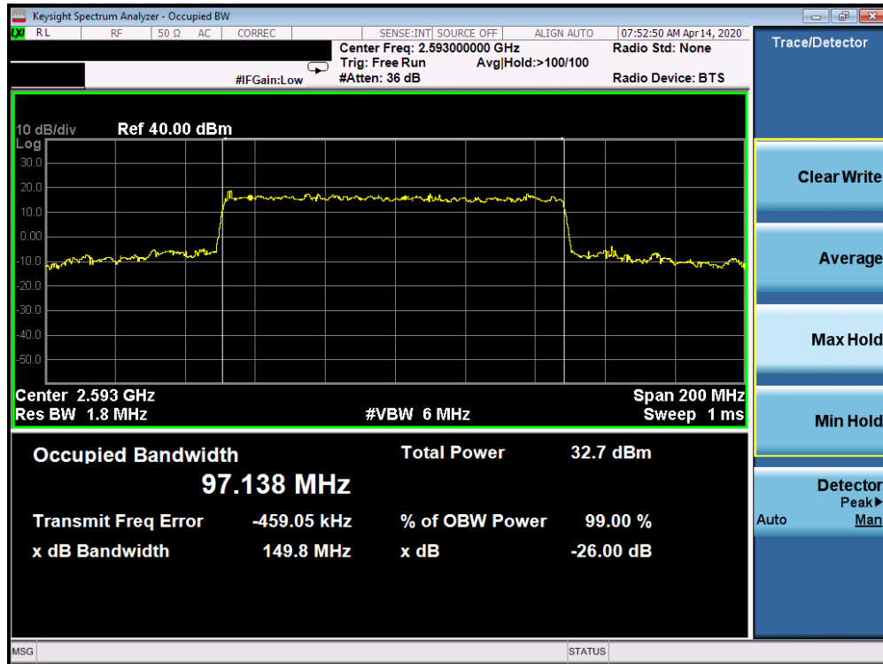
Plot 7-221. Occupied Bandwidth Plot (5G sub6 n41 - 100.0MHz 16-QAM - Full RB Configuration)
