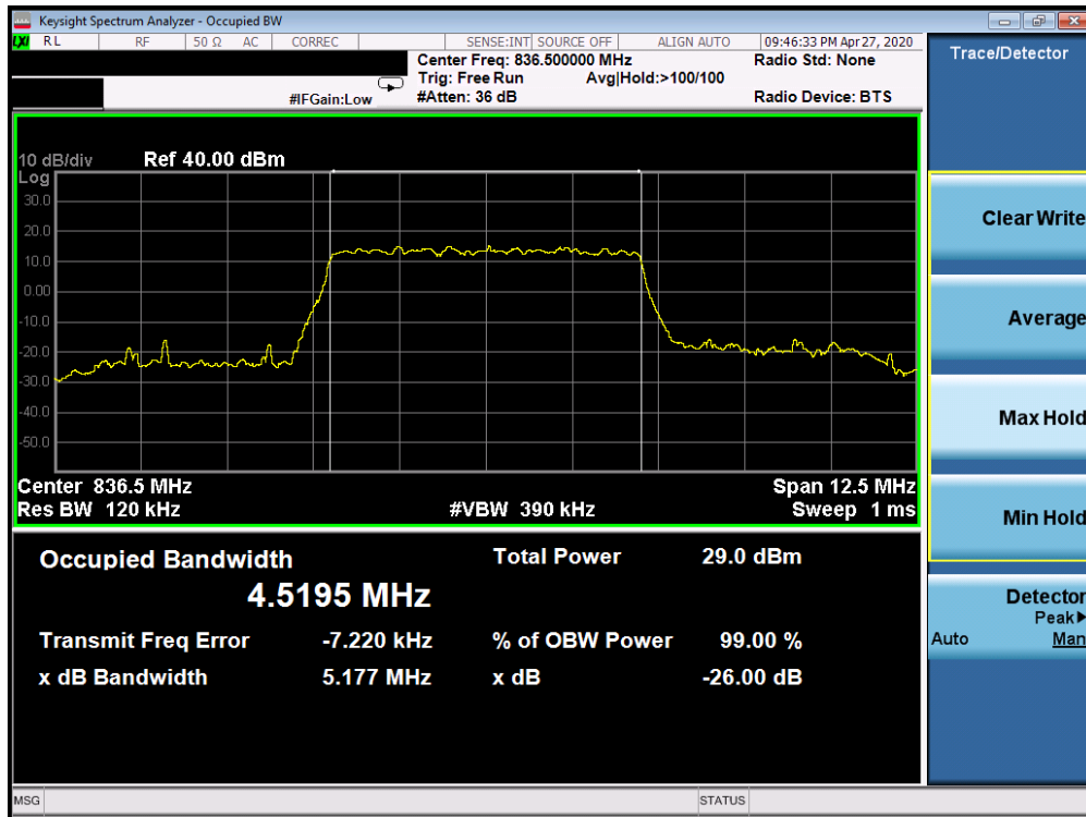
Plot 7-131. Occupied Bandwidth Plot (5G sub6 n5 - 5.0MHz 16-QAM - Full RB Configuration)
