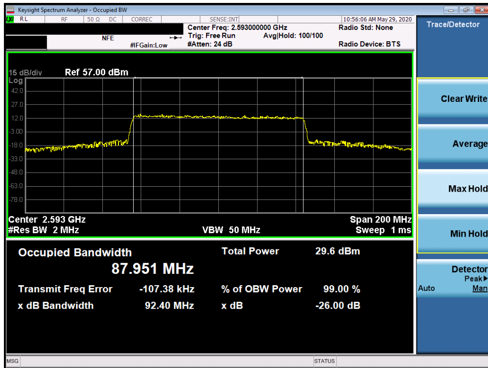
Plot 7-215. Occupied Bandwidth Plot (5G sub6 n41 – 90.0MHz QPSK - Full RB Configuration)
