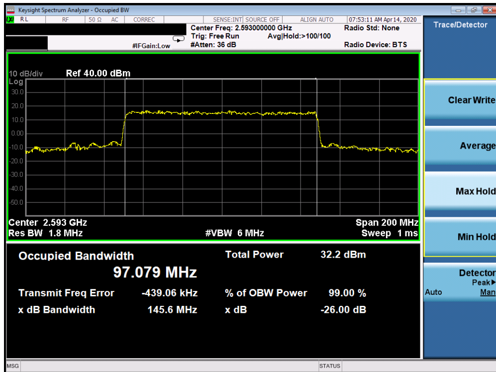
Plot 7-222. Occupied Bandwidth Plot (5G sub6 n41 - 100.0MHz 64-QAM - Full RB Configuration)
