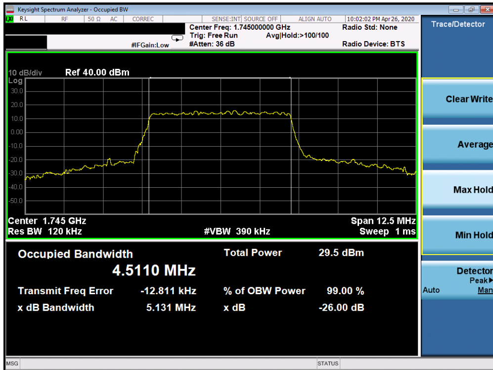
Plot 7-151. Occupied Bandwidth Plot (5G sub6 n66 - 5.0MHz 16-QAM - Full RB Configuration)
