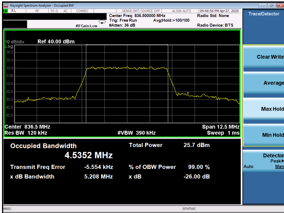
Plot 7-133. Occupied Bandwidth Plot (5G sub6 n5 - 5.0MHz 256-QAM - Full RB Configuration)
