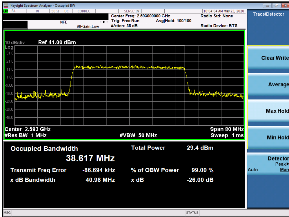
Plot 7-197. Occupied Bandwidth Plot (5G sub6 n41 - 40.0MHz 64-QAM - Full RB Configuration)
