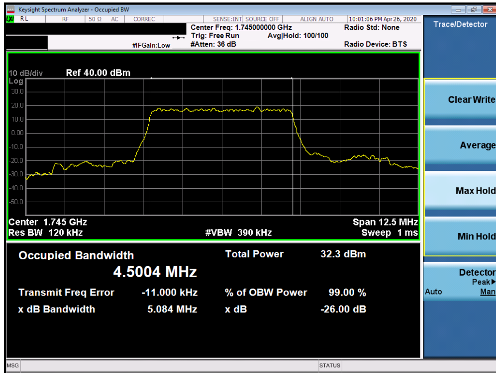
Plot 7-149. Occupied Bandwidth Plot (5G sub6 n66 - 5.0MHz BPSK - Full RB Configuration)
