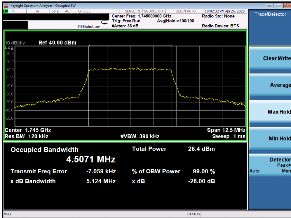
Plot 7-153. Occupied Bandwidth Plot (5G sub6 n66 - 5.0MHz 256-QAM - Full RB Configuration)
