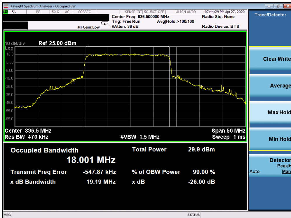
Plot 7-146. Occupied Bandwidth Plot (5G sub6 n5 – 20.0MHz 16-QAM - Full RB Configuration)
