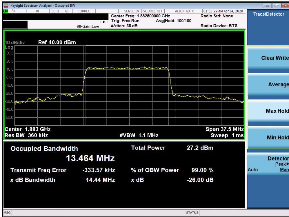
Plot 7-183. Occupied Bandwidth Plot (5G sub6 n25/2 - 15.0MHz 256-QAM - Full RB Configuration)
