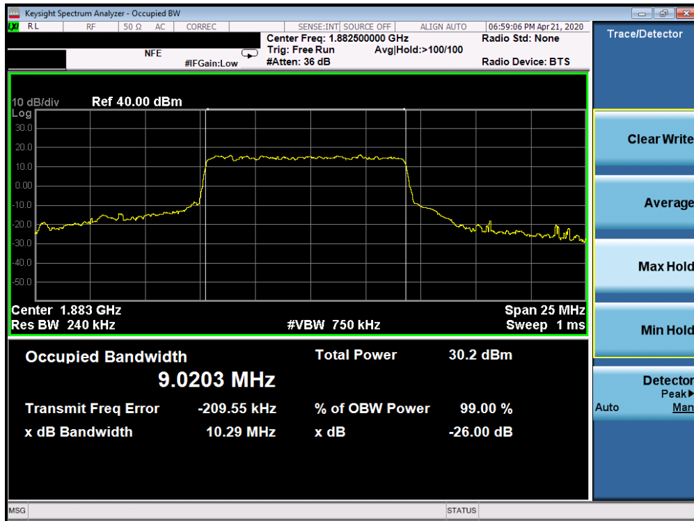
Plot 7-175. Occupied Bandwidth Plot (5G sub6 n25/2 - 10.0MHz QPSK - Full RB Configuration)
