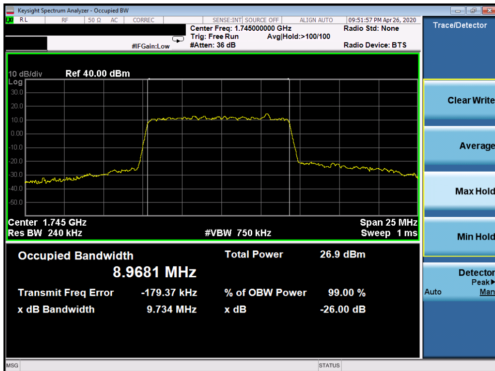
Plot 7-158. Occupied Bandwidth Plot (5G sub6 n66 - 10.0MHz 256-QAM - Full RB Configuration)
