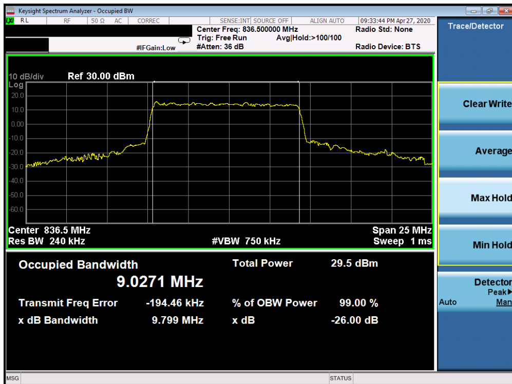
Plot 7-136. Occupied Bandwidth Plot (5G sub6 n5 - 10.0MHz 16-QAM - Full RB Configuration)
