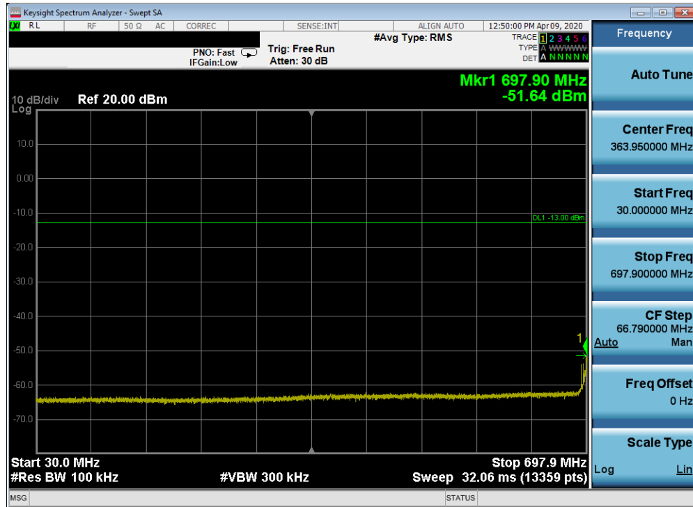
Plot 7-233. Conducted Spurious Plot (Band 12/17 - 10.0MHz QPSK - RB Size 1, RB Offset 0 - Low Channel)
