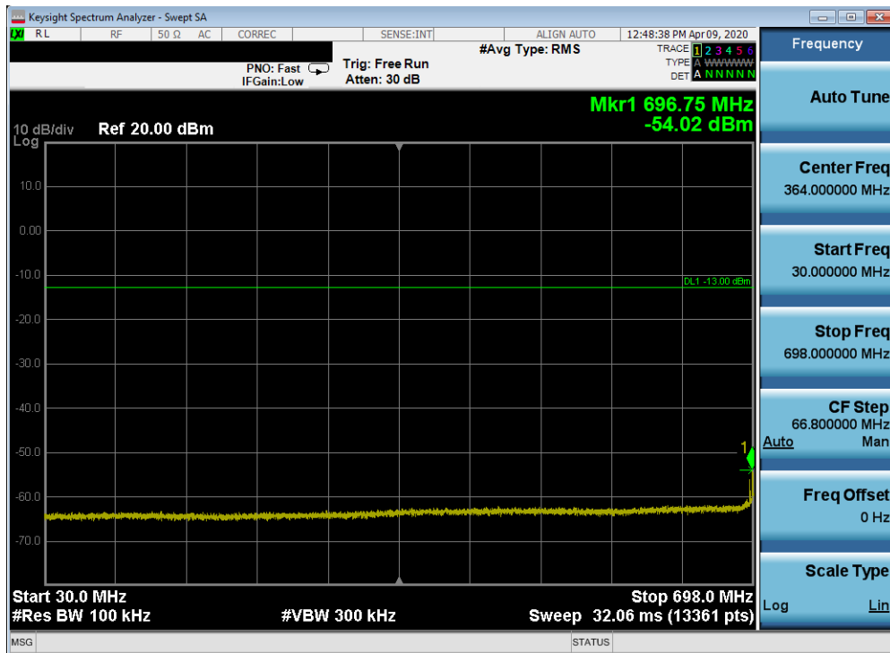
Plot 7-236. Conducted Spurious Plot (Band 12/17 - 10.0MHz QPSK - RB Size 1, RB Offset 0 - Mid Channel)
