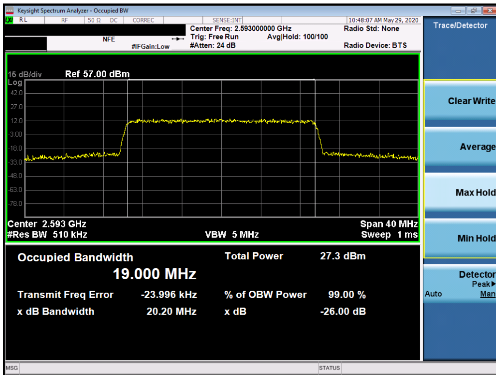
Plot 7-192. Occupied Bandwidth Plot (5G sub6 n41 - 20.0MHz 64-QAM - Full RB Configuration)
