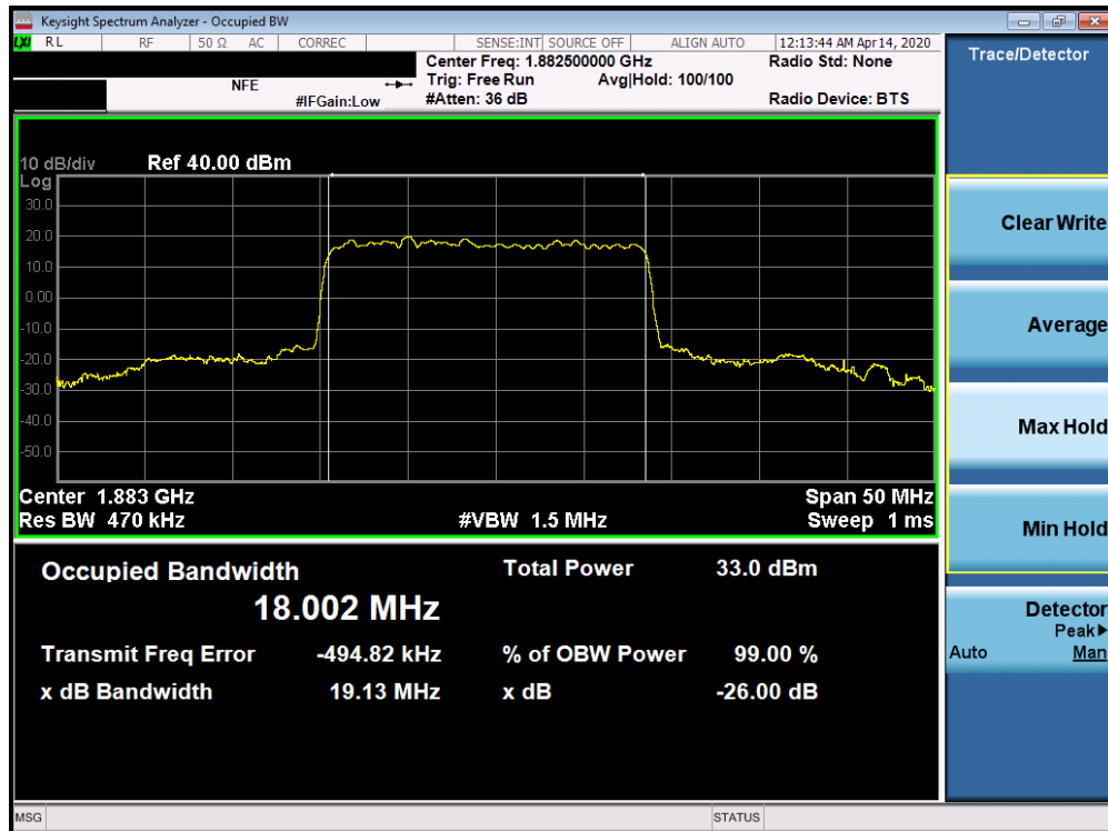
Plot 7-184. Occupied Bandwidth Plot (5G sub6 n25/2 - 20.0MHz BPSK - Full RB Configuration)
