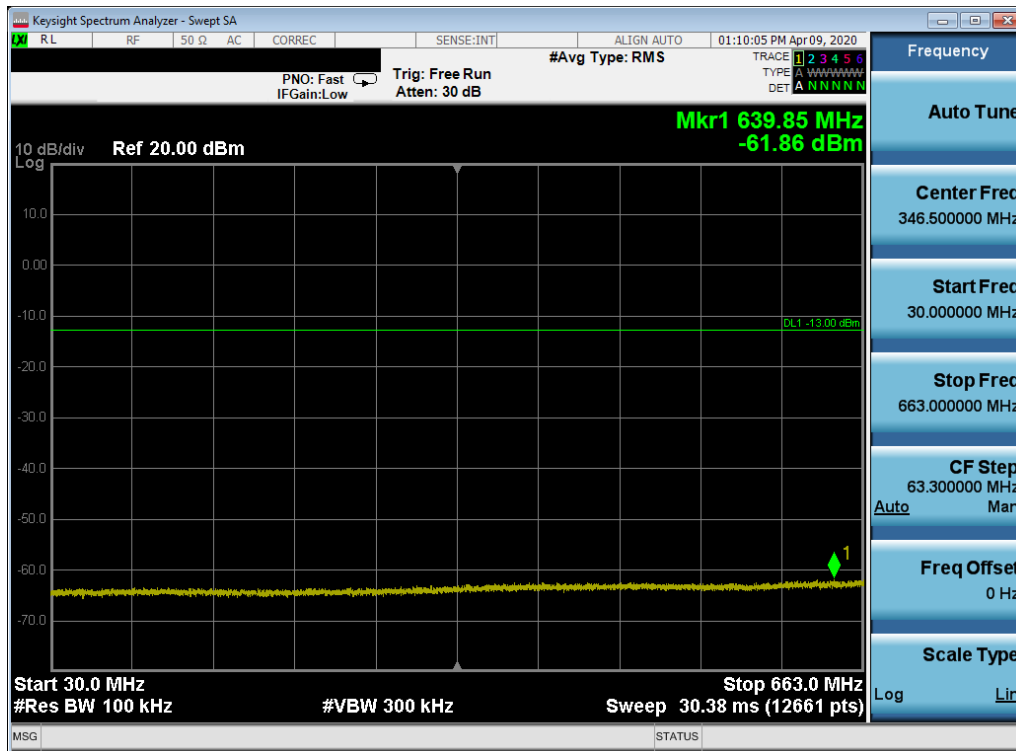
Plot 7-230. Conducted Spurious Plot (Band 71 - 10.0MHz QPSK - RB Size 1, RB Offset 0 - High Channel)
