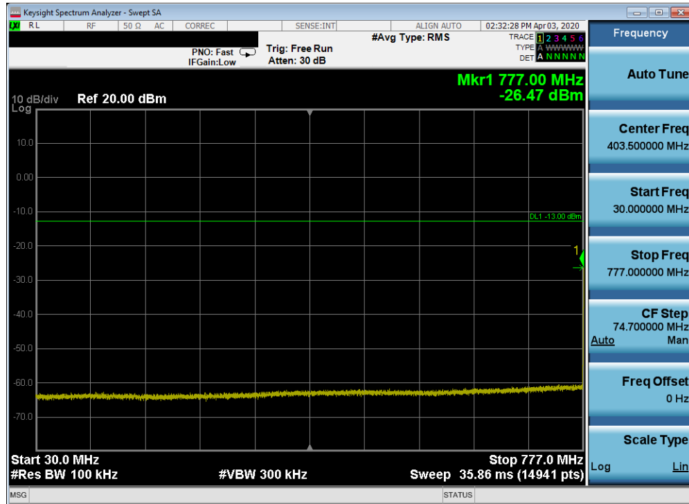
Plot 7-242. Conducted Spurious Plot (Band 13 - 10.0MHz QPSK - RB Size 1, RB Offset 0 - Mid Channel)
