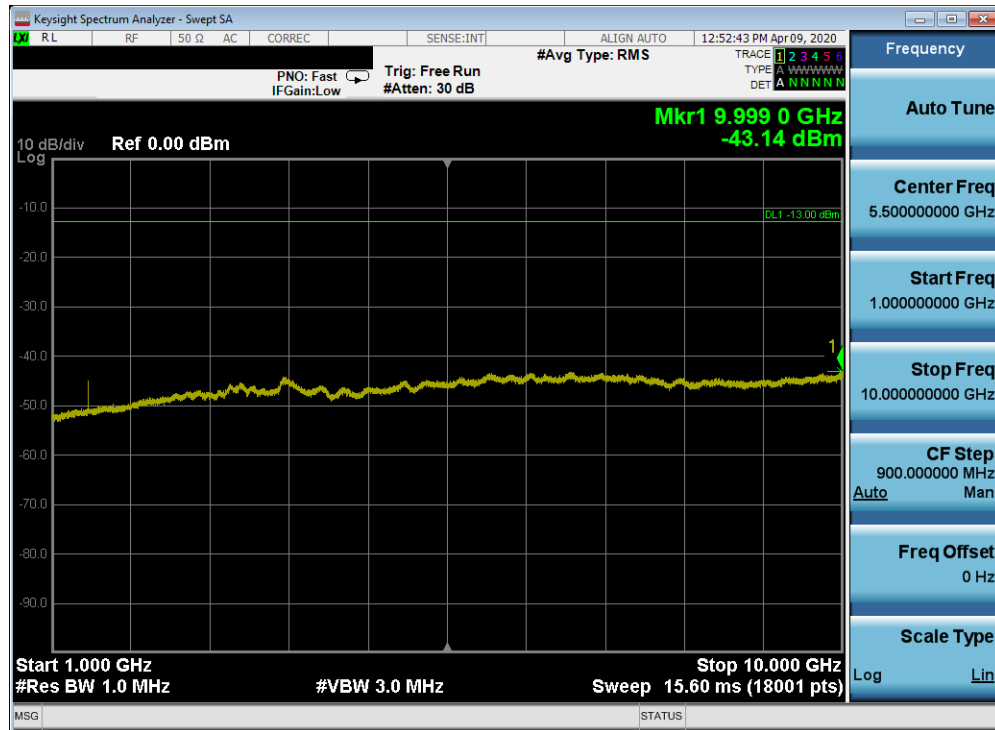
Plot 7-241. Conducted Spurious Plot (Band 12/17 - 10.0MHz QPSK - RB Size 1, RB Offset 0 - High Channel)
