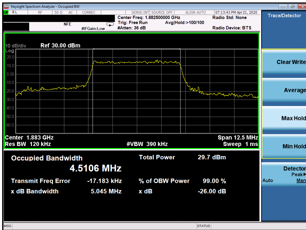
Plot 7-170. Occupied Bandwidth Plot (5G sub6 n25/2 - 5.0MHz QPSK - Full RB Configuration)
