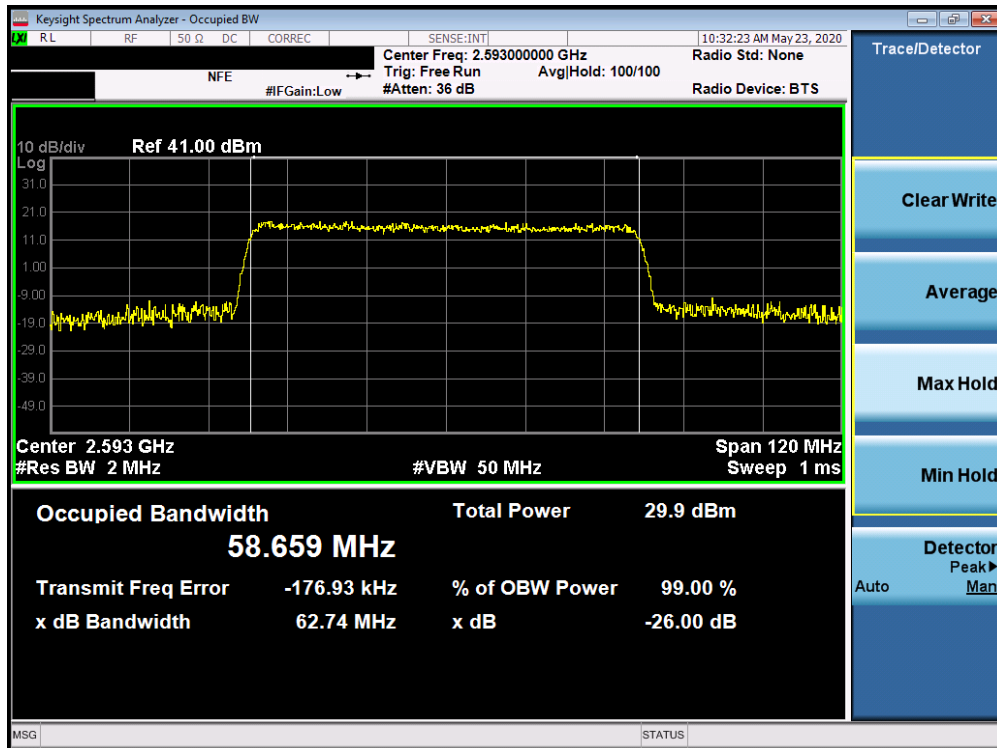
Plot 7-206. Occupied Bandwidth Plot (5G sub6 n41 - 60.0MHz 16-QAM - Full RB Configuration)
