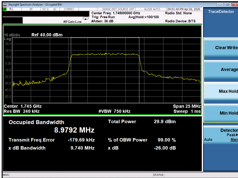
Plot 7-157. Occupied Bandwidth Plot (5G sub6 n66 - 10.0MHz 64-QAM - Full RB Configuration)
