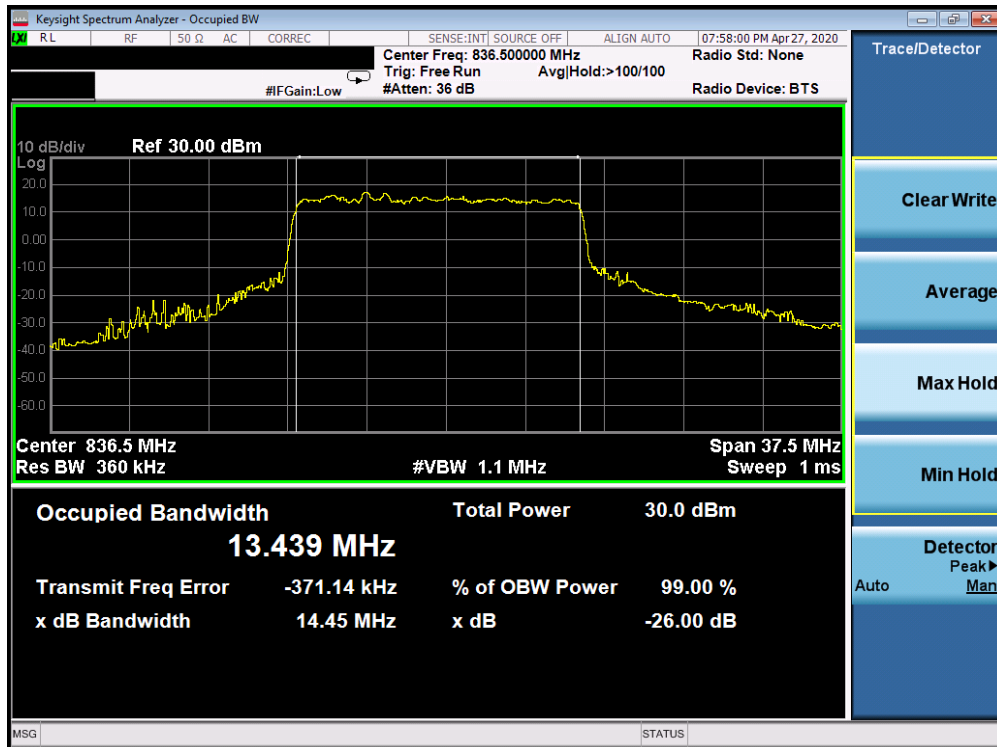
Plot 7-141. Occupied Bandwidth Plot (5G sub6 n5 – 15.0MHz 16-QAM - Full RB Configuration)
