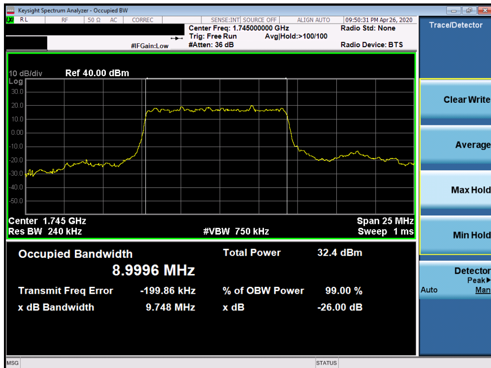
Plot 7-154. Occupied Bandwidth Plot (5G sub6 n66 - 10.0MHz BPSK - Full RB Configuration)
