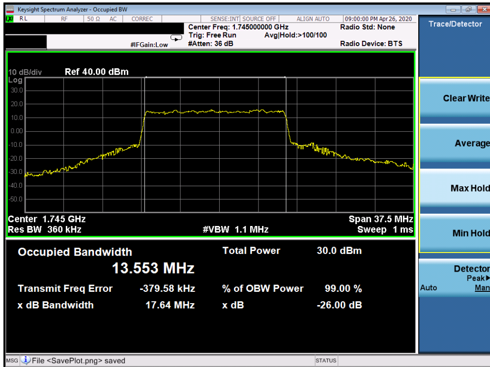
Plot 7-163. Occupied Bandwidth Plot (5G sub6 n66 - 15.0MHz 256-QAM - Full RB Configuration)
