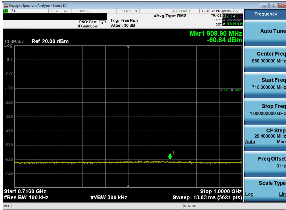
Plot 7-237. Conducted Spurious Plot (Band 12/17 - 10.0MHz QPSK - RB Size 1, RB Offset 0 - Mid Channel)
