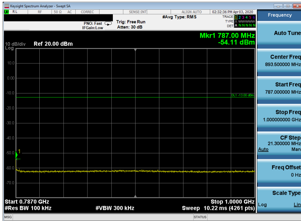
Plot 7-243. Conducted Spurious Plot (Band 13 - 10.0MHz QPSK - RB Size 1, RB Offset 0 - Mid Channel)
