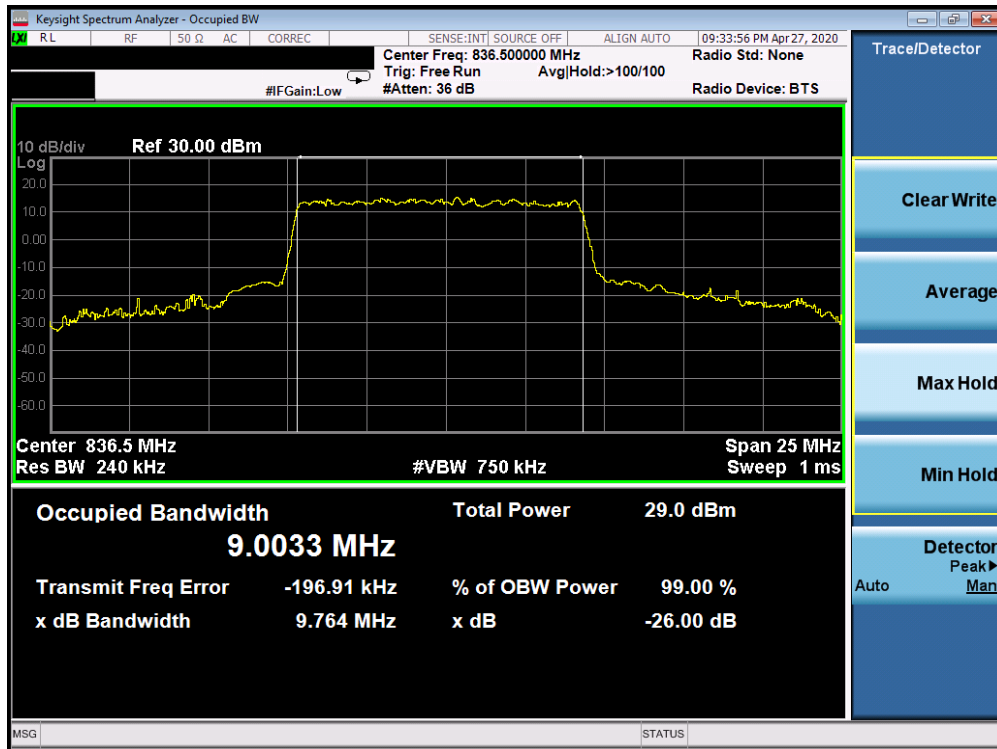
Plot 7-137. Occupied Bandwidth Plot (5G sub6 n5 - 10.0MHz 64-QAM - Full RB Configuration)
