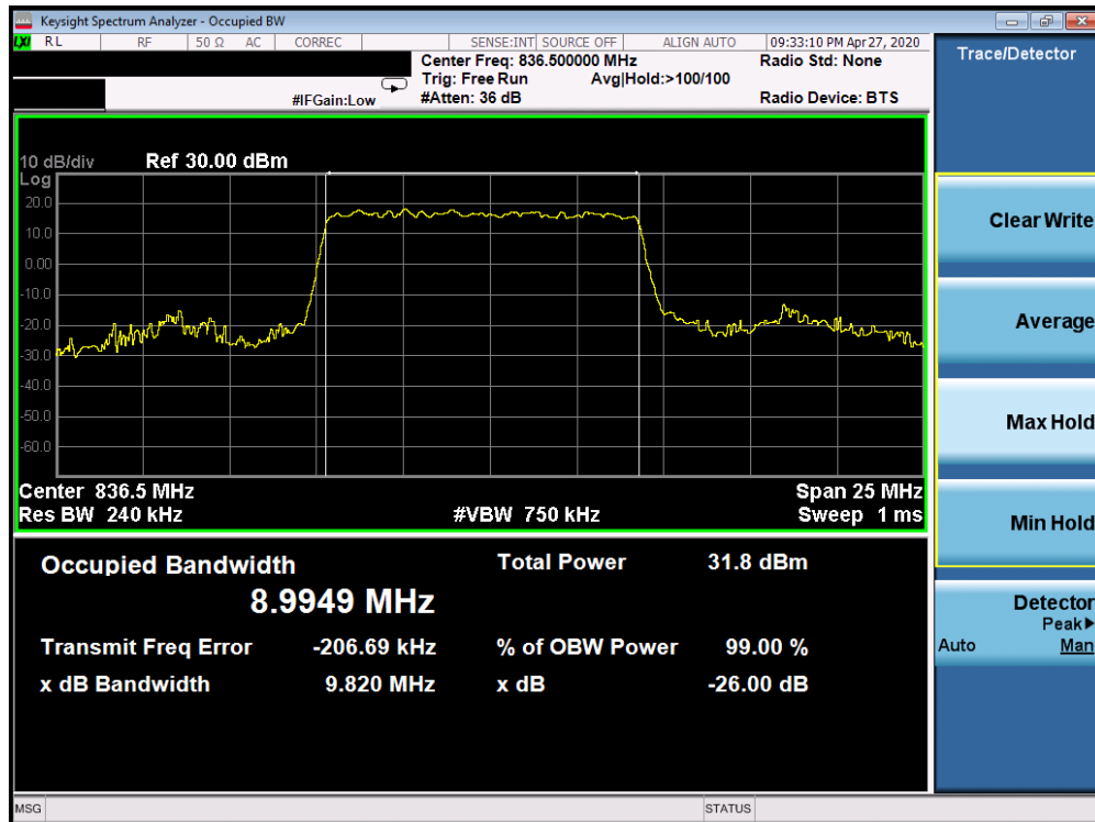
Plot 7-134. Occupied Bandwidth Plot (5G sub6 n5 - 10.0MHz BPSK - Full RB Configuration)
