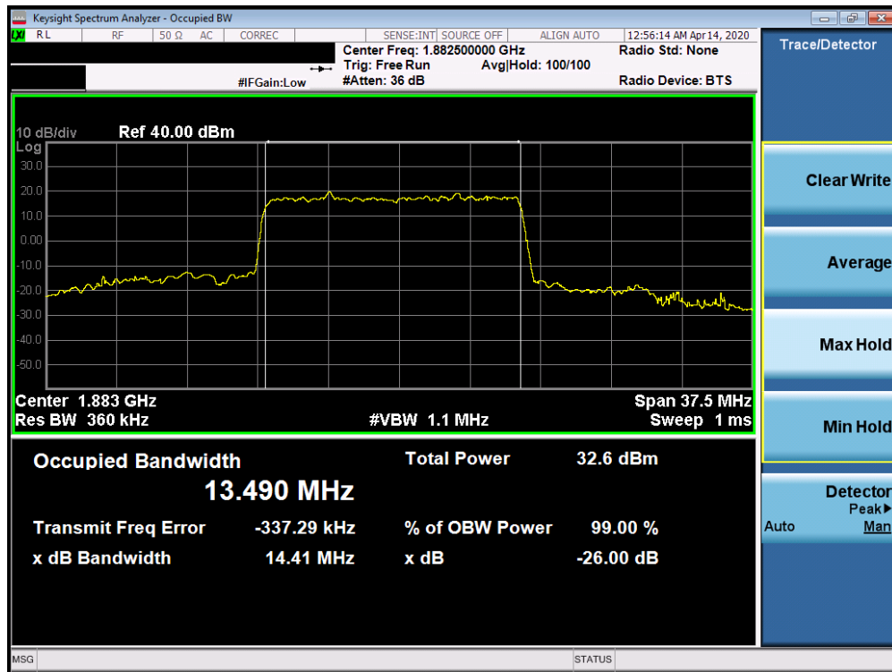
Plot 7-179. Occupied Bandwidth Plot (5G sub6 n25/2 - 15.0MHz BPSK - Full RB Configuration)
