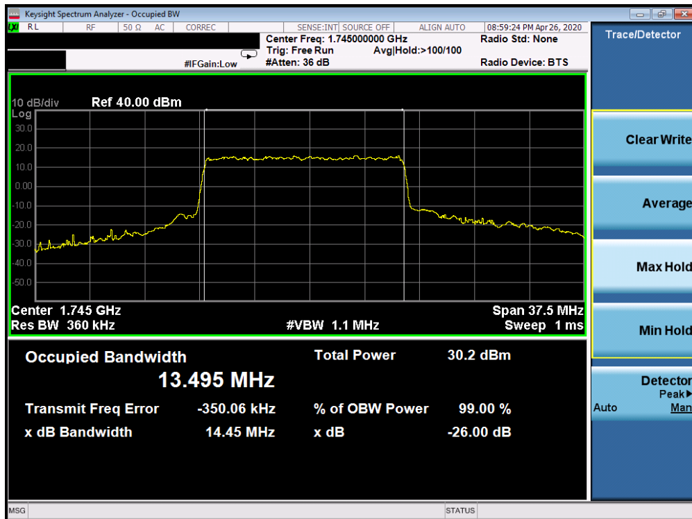
Plot 7-160. Occupied Bandwidth Plot (5G sub6 n66 - 15.0MHz QPSK - Full RB Configuration)
