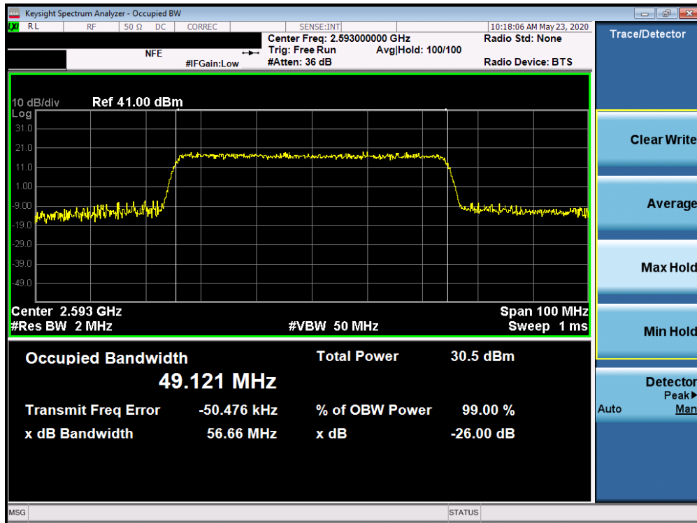
Plot 7-201. Occupied Bandwidth Plot (5G sub6 n41 - 50.0MHz 16-QAM - Full RB Configuration)
