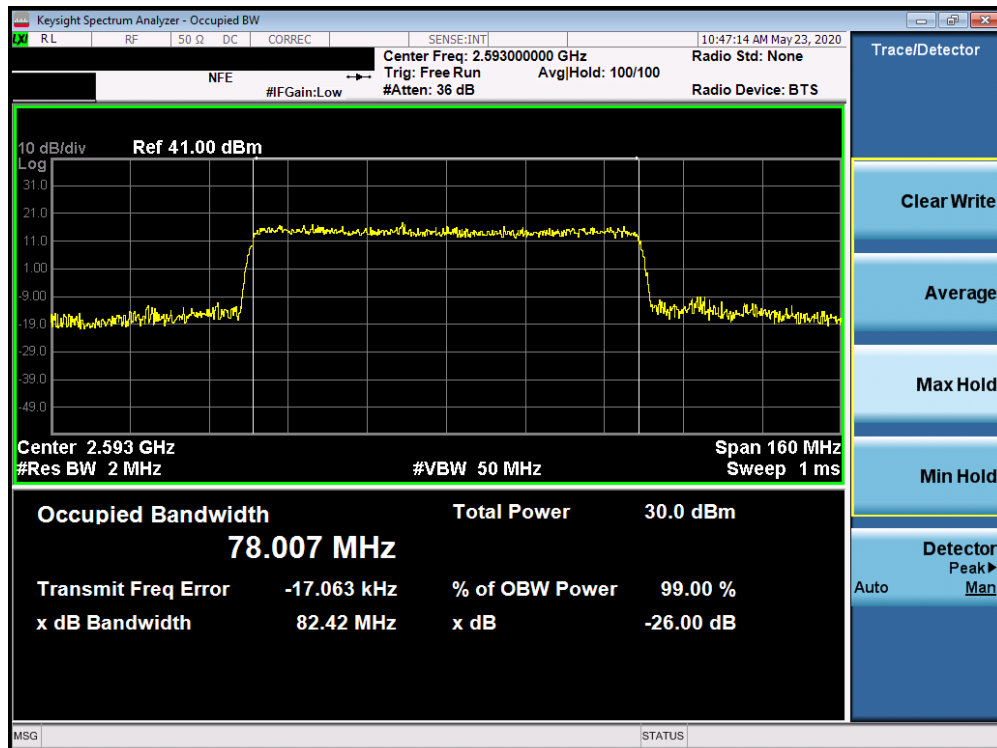
Plot 7-210. Occupied Bandwidth Plot (5G sub6 n41 - 80.0MHz QPSK - Full RB Configuration)
