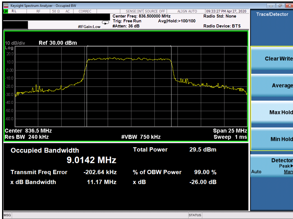
Plot 7-135. Occupied Bandwidth Plot (5G sub6 n5 - 10.0MHz QPSK - Full RB Configuration)
