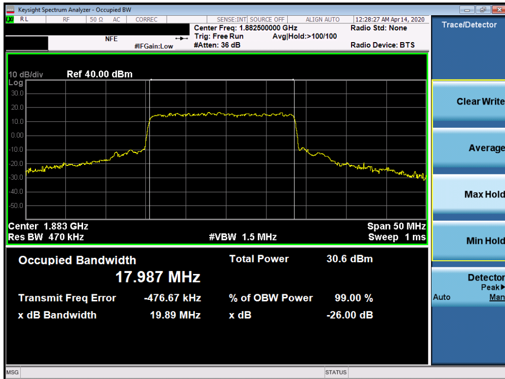
Plot 7-185. Occupied Bandwidth Plot (5G sub6 n25/2 - 20.0MHz QPSK - Full RB Configuration)
