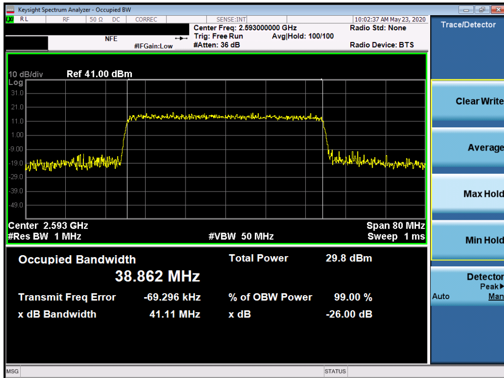
Plot 7-196. Occupied Bandwidth Plot (5G sub6 n41 - 40.0MHz 16-QAM - Full RB Configuration)
