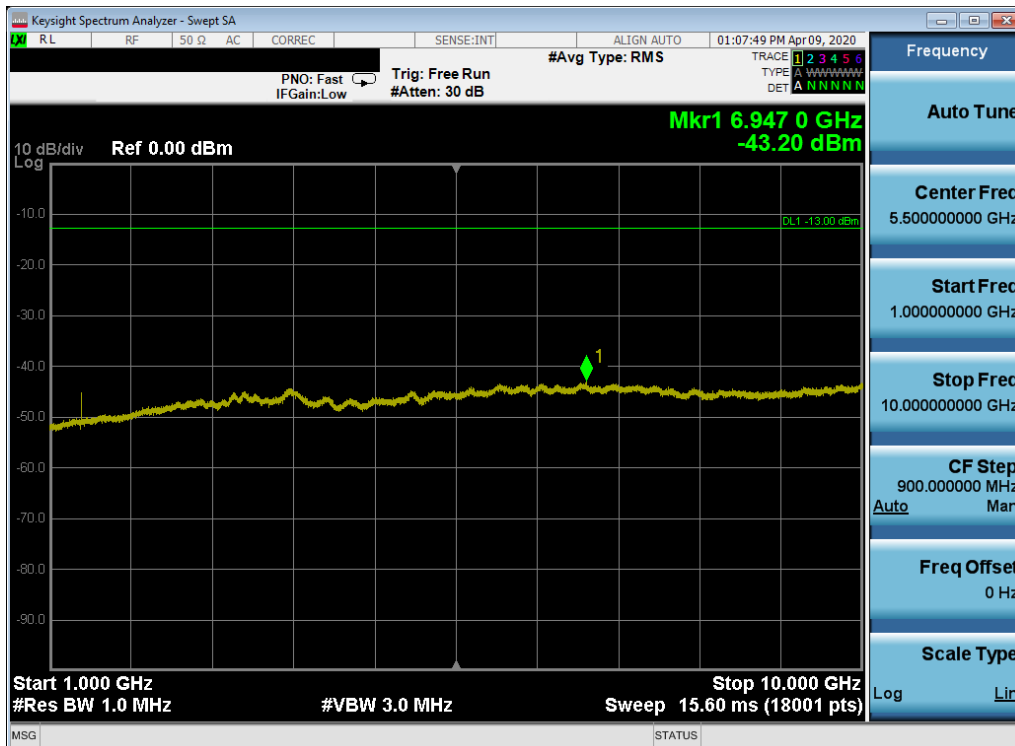
Plot 7-229. Conducted Spurious Plot (Band 71 - 10.0MHz QPSK - RB Size 1, RB Offset 0 - Mid Channel)
