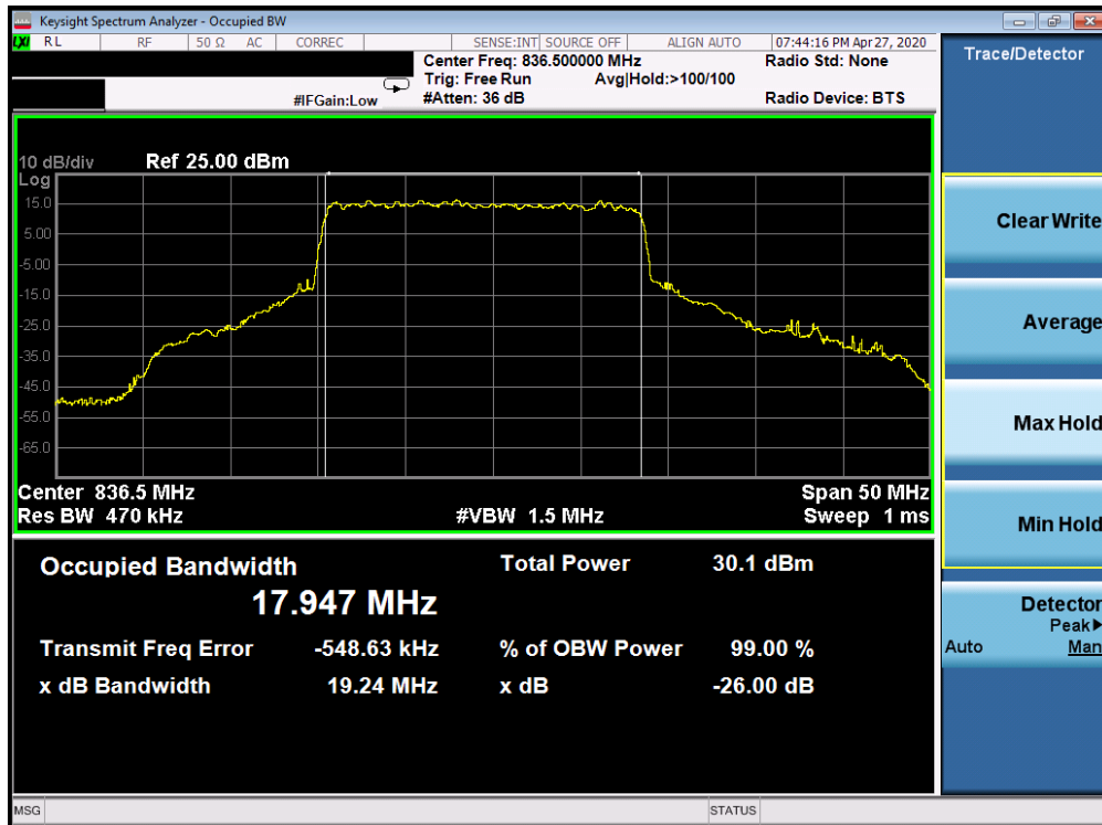
Plot 7-145. Occupied Bandwidth Plot (5G sub6 n5 – 20.0MHz QPSK - Full RB Configuration)
