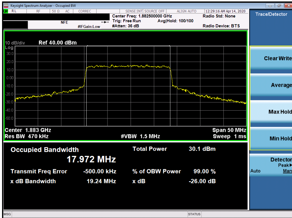
Plot 7-187. Occupied Bandwidth Plot (5G sub6 n25/2 - 20.0MHz 64-QAM - Full RB Configuration)
