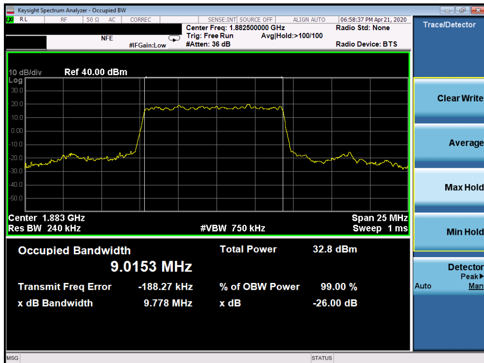
Plot 7-174. Occupied Bandwidth Plot (5G sub6 n25/2 - 10.0MHz BPSK - Full RB Configuration)
