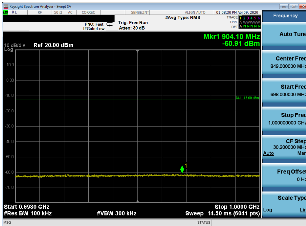
Plot 7-225. Conducted Spurious Plot (Band 71 - 10.0MHz QPSK - RB Size 1, RB Offset 0 - Low Channel)
