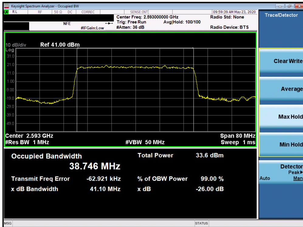
Plot 7-194. Occupied Bandwidth Plot (5G sub6 n41 - 40.0MHz BPSK - Full RB Configuration)
