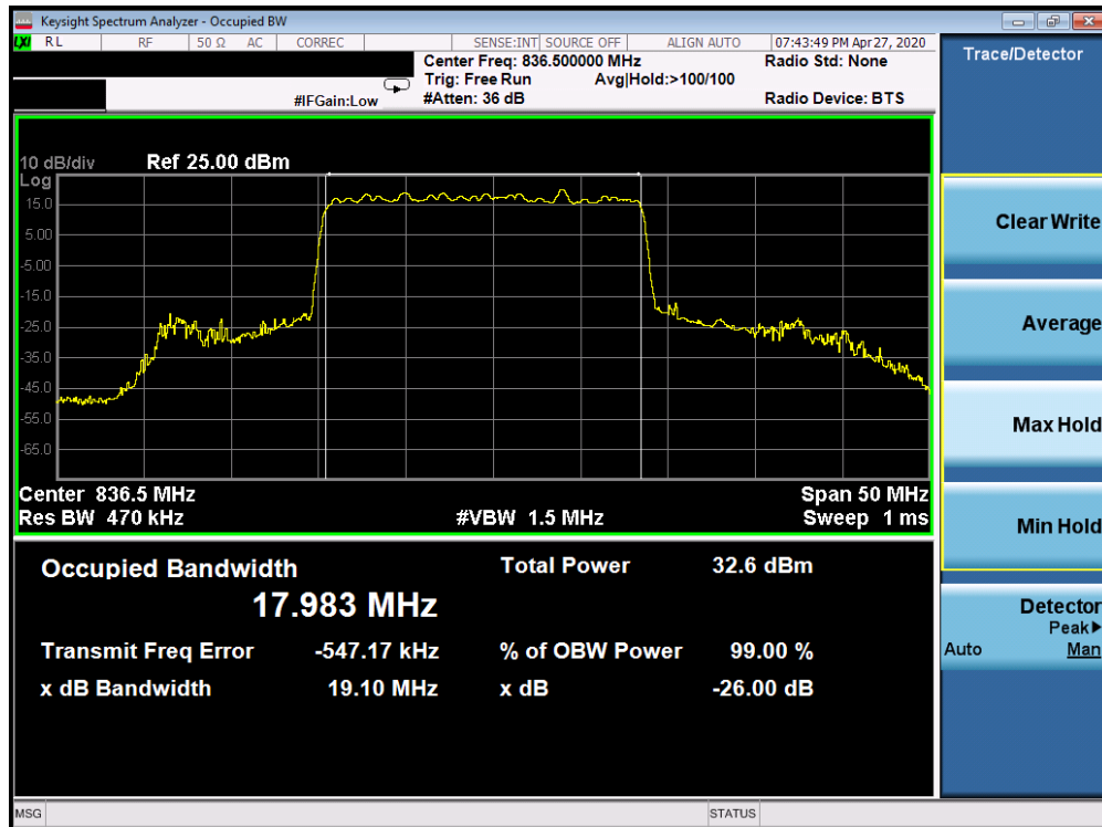
Plot 7-144. Occupied Bandwidth Plot (5G sub6 n5 – 20.0MHz BPSK - Full RB Configuration)
