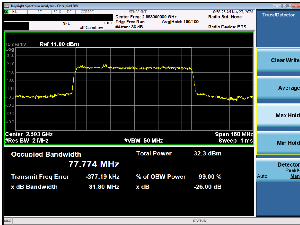
Plot 7-209. Occupied Bandwidth Plot (5G sub6 n41 - 80.0MHz BPSK - Full RB Configuration)
