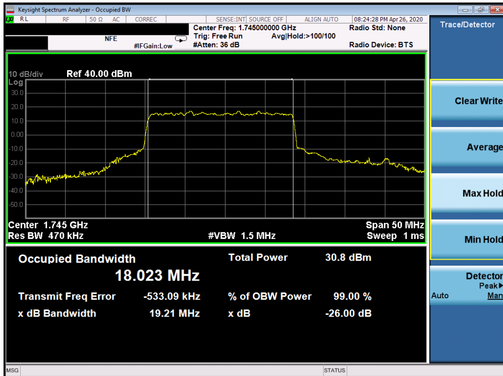
Plot 7-166. Occupied Bandwidth Plot (5G sub6 n66 - 20.0MHz 16-QAM - Full RB Configuration)
