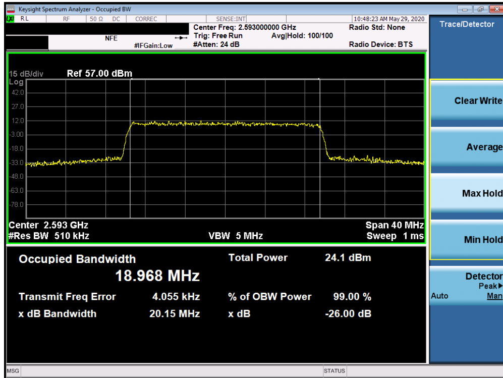
Plot 7-193. Occupied Bandwidth Plot (5G sub6 n41 - 20.0MHz 256-QAM - Full RB Configuration)
