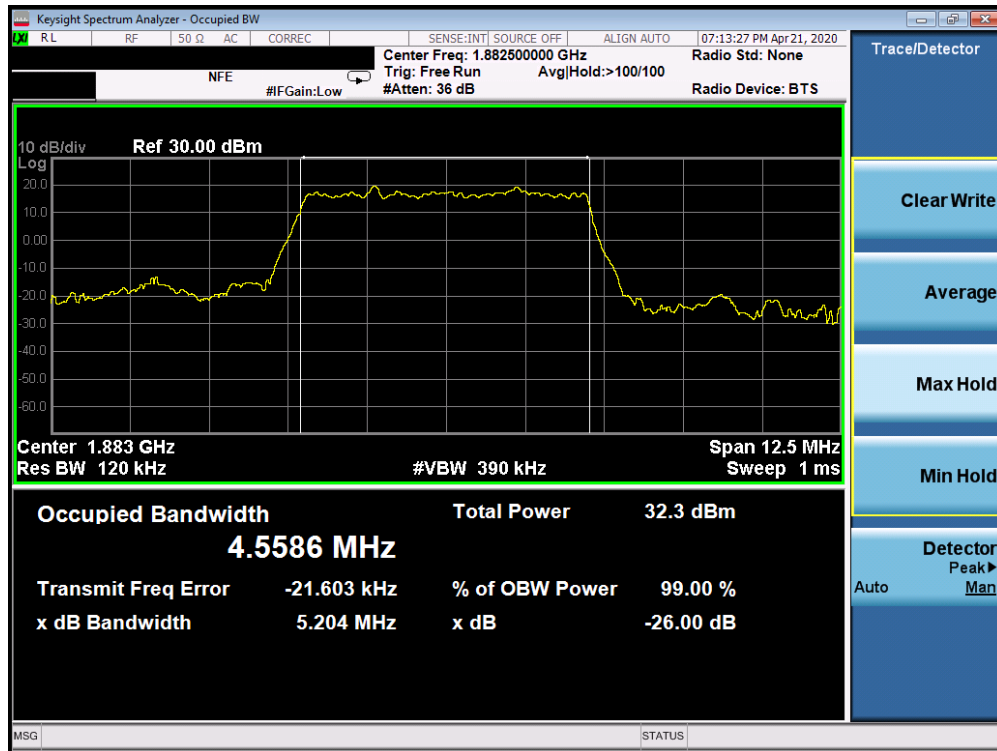
Plot 7-169. Occupied Bandwidth Plot (5G sub6 n25/2 - 5.0MHz BPSK - Full RB Configuration)
