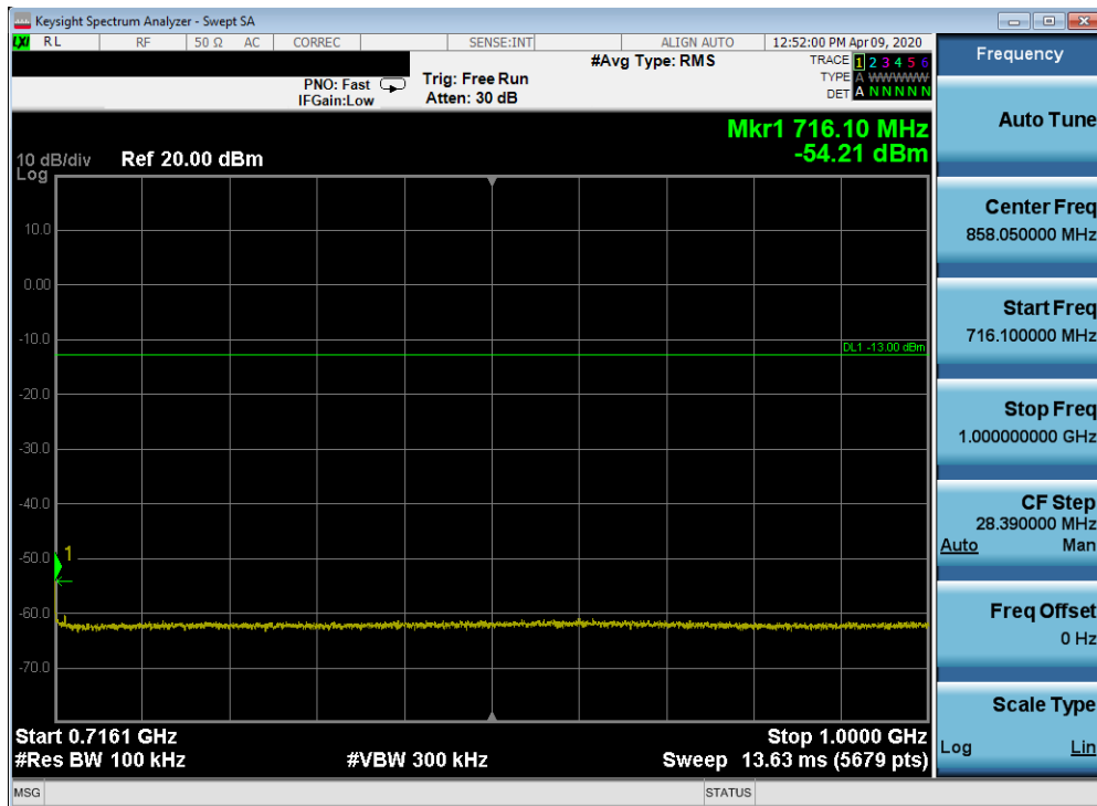
Plot 7-240. Conducted Spurious Plot (Band 12/17 - 10.0MHz QPSK - RB Size 1, RB Offset 0 - High Channel)
