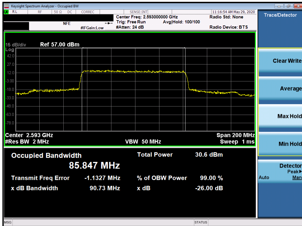
Plot 7-214. Occupied Bandwidth Plot (5G sub6 n41 - 90.0MHz BPSK - Full RB Configuration)
