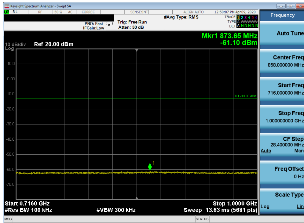
Plot 7-234. Conducted Spurious Plot (Band 12/17 - 10.0MHz QPSK - RB Size 1, RB Offset 0 - Low Channel)
