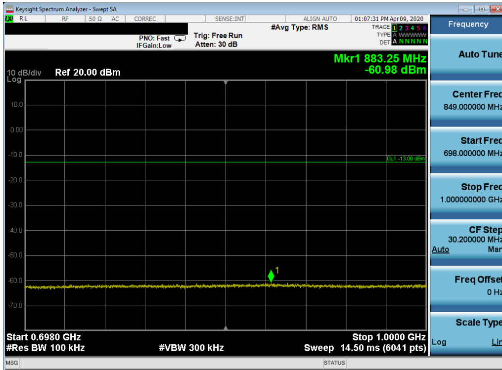
Plot 7-228. Conducted Spurious Plot (Band 71 - 10.0MHz QPSK - RB Size 1, RB Offset 0 - Mid Channel)
