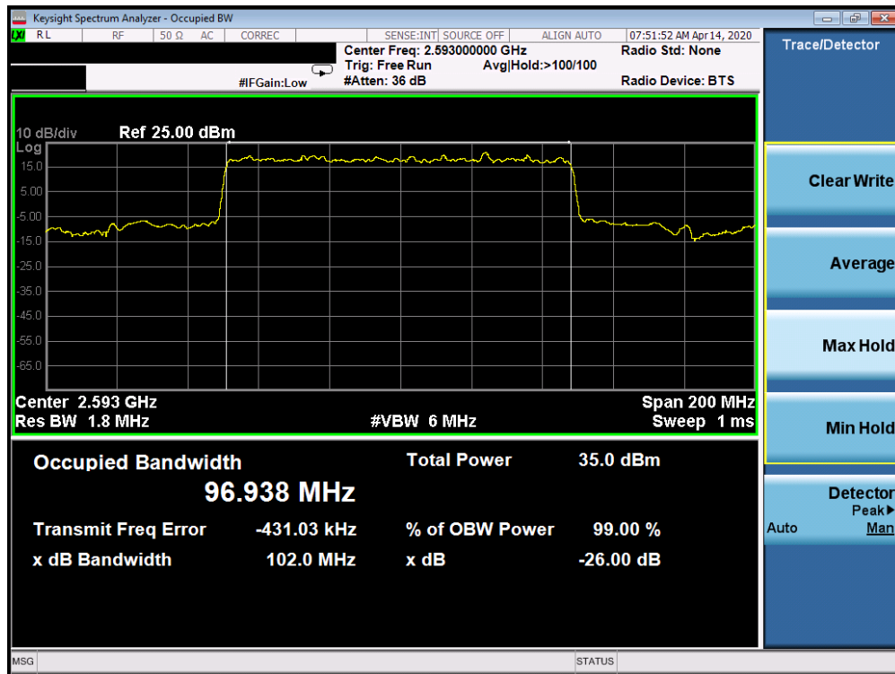
Plot 7-219. Occupied Bandwidth Plot (5G sub6 n41 - 100.0MHz BPSK - Full RB Configuration)
