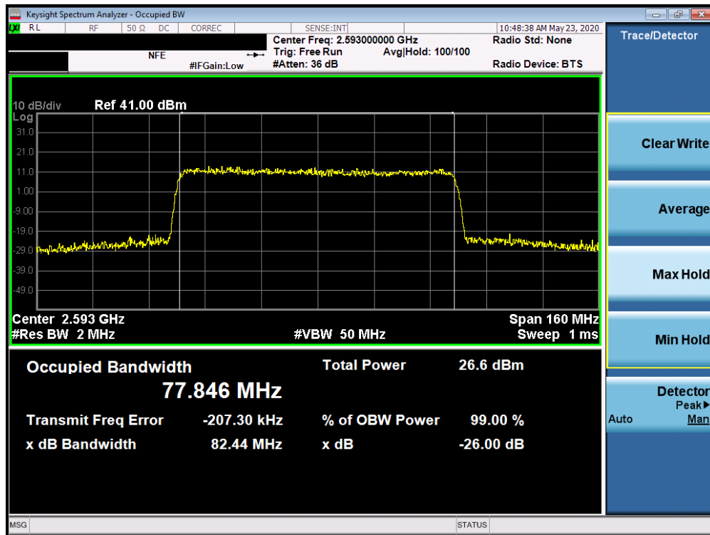
Plot 7-213. Occupied Bandwidth Plot (5G sub6 n41 - 80.0MHz 256-QAM - Full RB Configuration)
