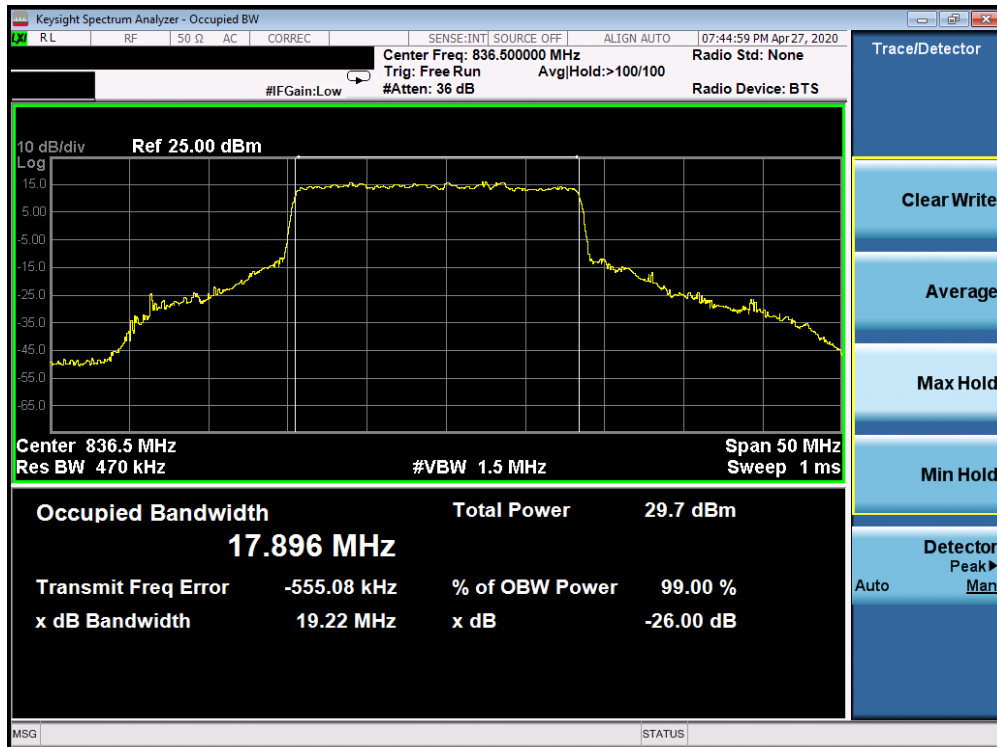
Plot 7-147. Occupied Bandwidth Plot (5G sub6 n5 - 20.0MHz 64-QAM - Full RB Configuration)
