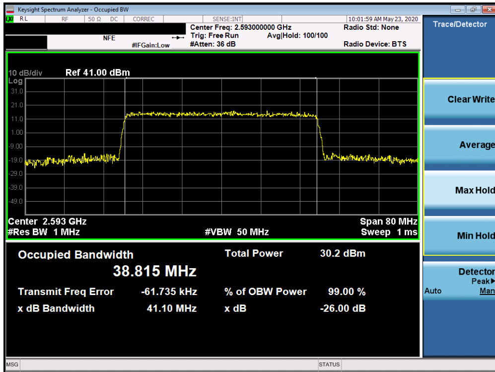
Plot 7-195. Occupied Bandwidth Plot (5G sub6 n41 - 40.0MHz QPSK - Full RB Configuration)
