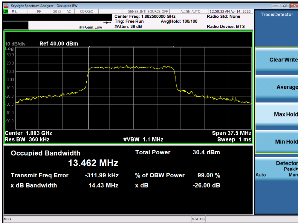
Plot 7-181. Occupied Bandwidth Plot (5G sub6 n25/2 - 15.0MHz 16-QAM - Full RB Configuration)
