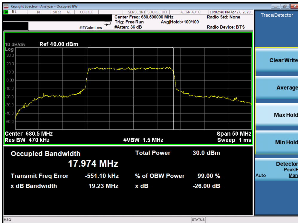
Plot 7-126. Occupied Bandwidth Plot (5G sub6 n71 - 20.0MHz 16-QAM - Full RB Configuration)
