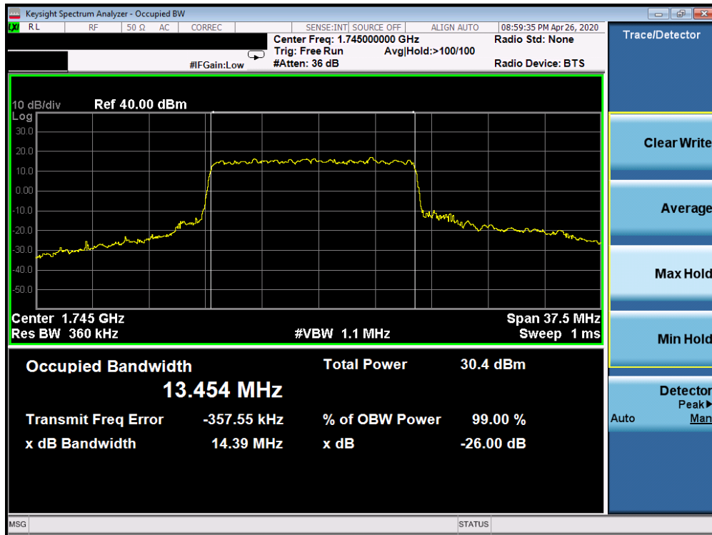
Plot 7-161. Occupied Bandwidth Plot (5G sub6 n66 - 15.0MHz 16-QAM - Full RB Configuration)
