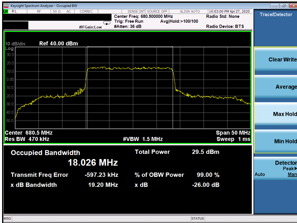
Plot 7-127. Occupied Bandwidth Plot (5G sub6 n71 - 20.0MHz 64-QAM - Full RB Configuration)
