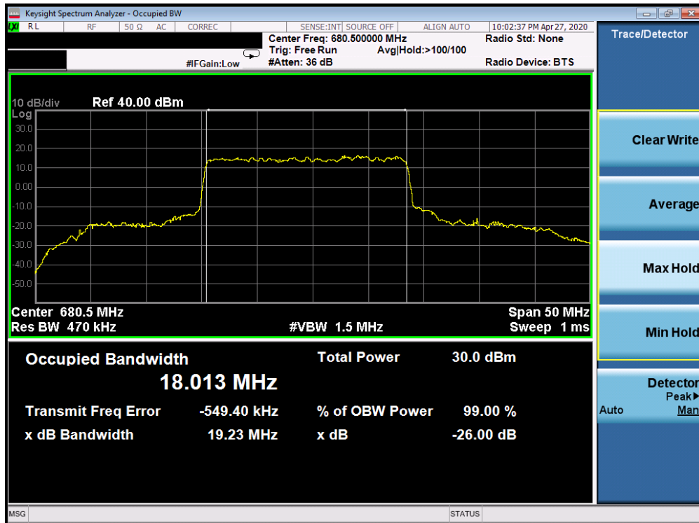
Plot 7-125. Occupied Bandwidth Plot (5G sub6 n71 - 20.0MHz QPSK - Full RB Configuration)
