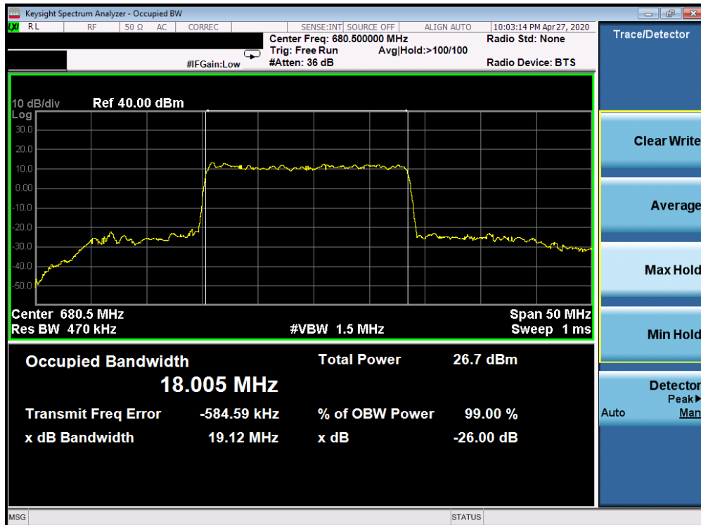
Plot 7-128. Occupied Bandwidth Plot (5G sub6 n71 - 20.0MHz 256-QAM - Full RB Configuration)
