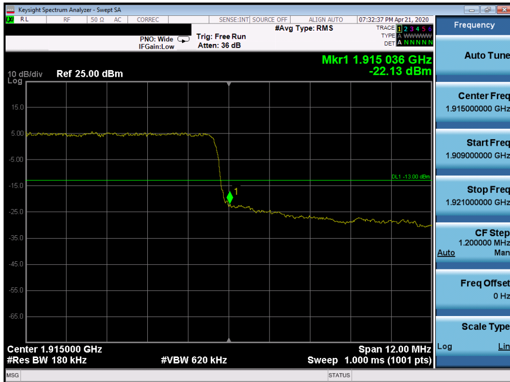
Plot 7-524. Upper 5G sub6 Band Edge Plot (5G sub6 n25 - 15.0MHz QPSK - Full RB Configuration)
