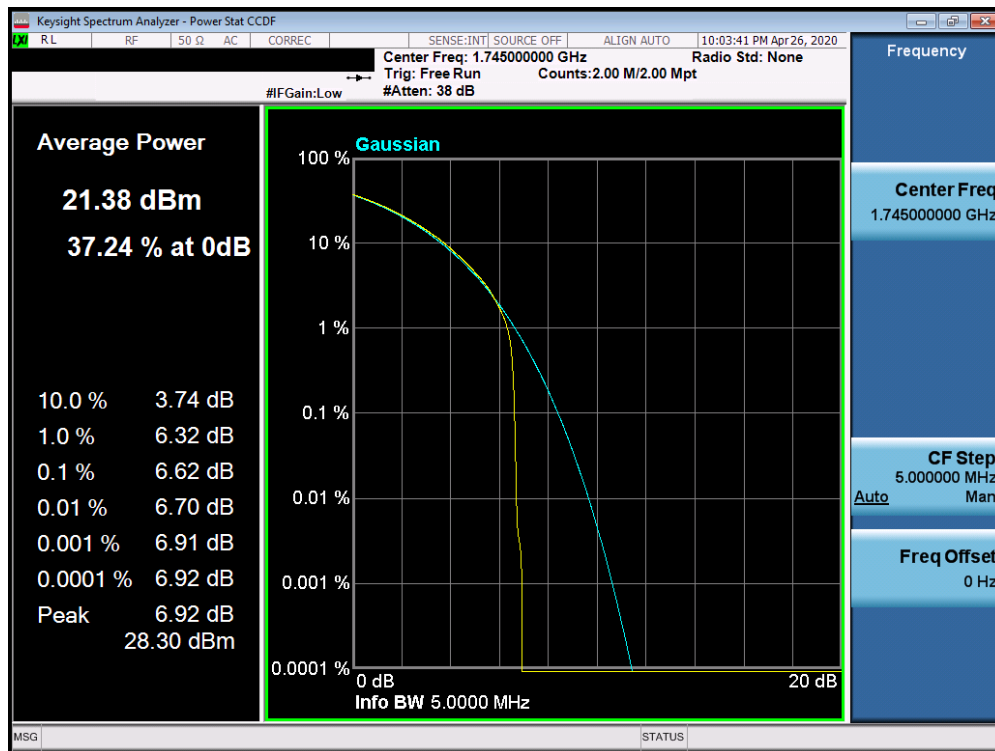
Plot 7-582. PAR Plot (5G sub6 n66/4 - 5.0MHz QPSK - Full RB Configuration)
