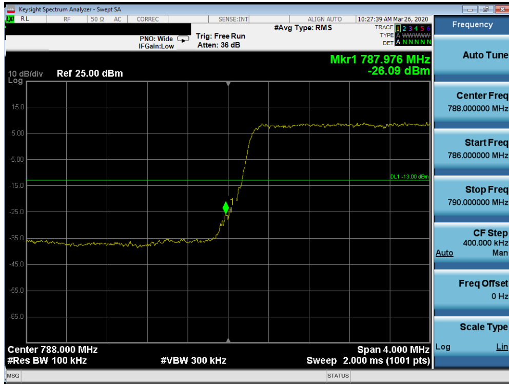
Plot 7-10. Lower Band Edge Plot (LTE Band 14, 5MHz QPSK - RB Size 25)
