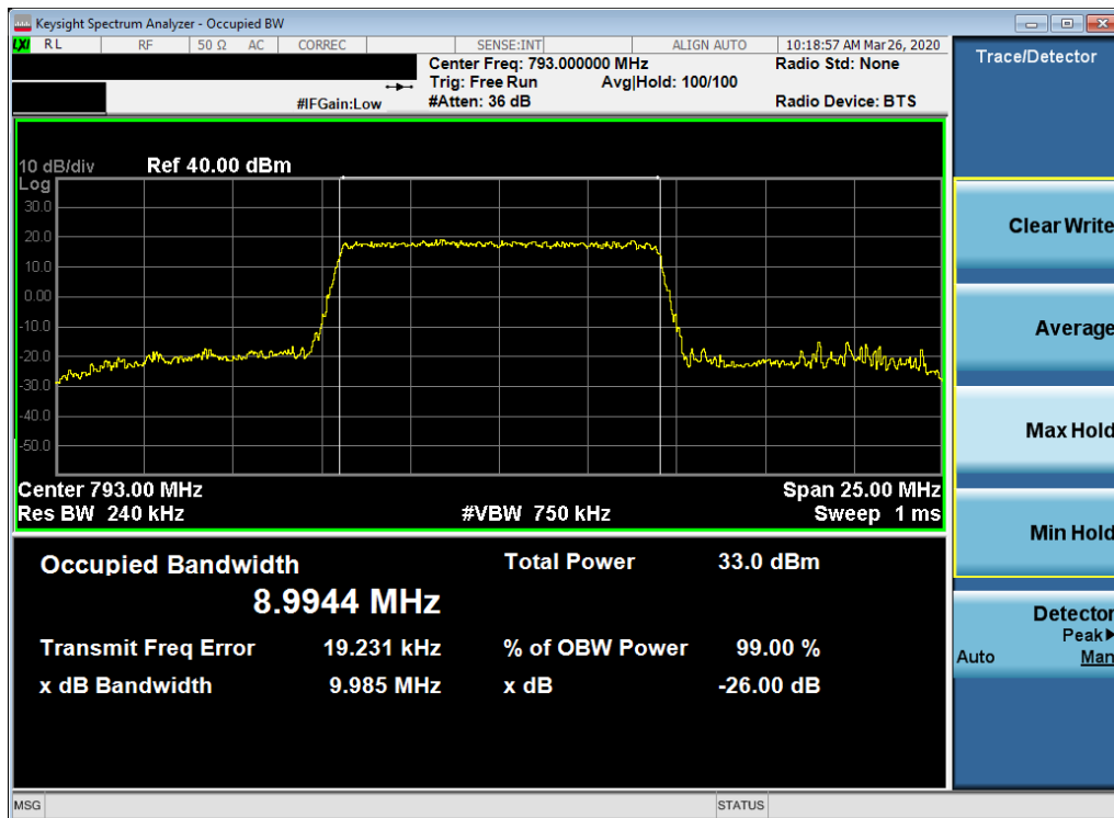
Plot 7-4. Occupied Bandwidth Plot (LTE Band 14 - 10MHz QPSK - Full RB Configuration)
