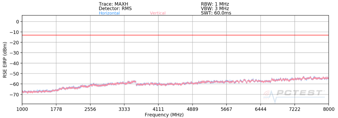
Plot 7-19. Radiated Spurious Plot (Band 14)
