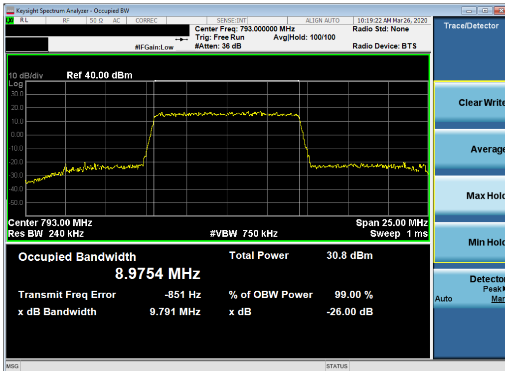
Plot 7-6. Occupied Bandwidth Plot (LTE Band 14 - 10MHz 64-QAM - Full RB Configuration)
