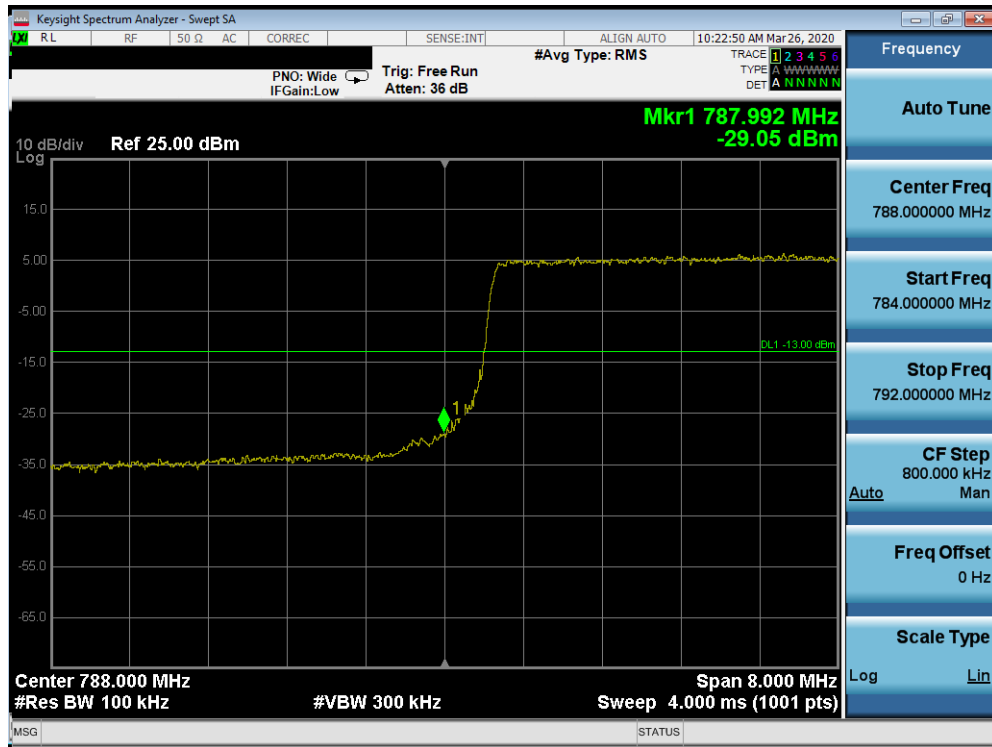
Plot 7-14. Lower Band Edge Plot (LTE Band 14, 10MHz QPSK - RB Size 50)
