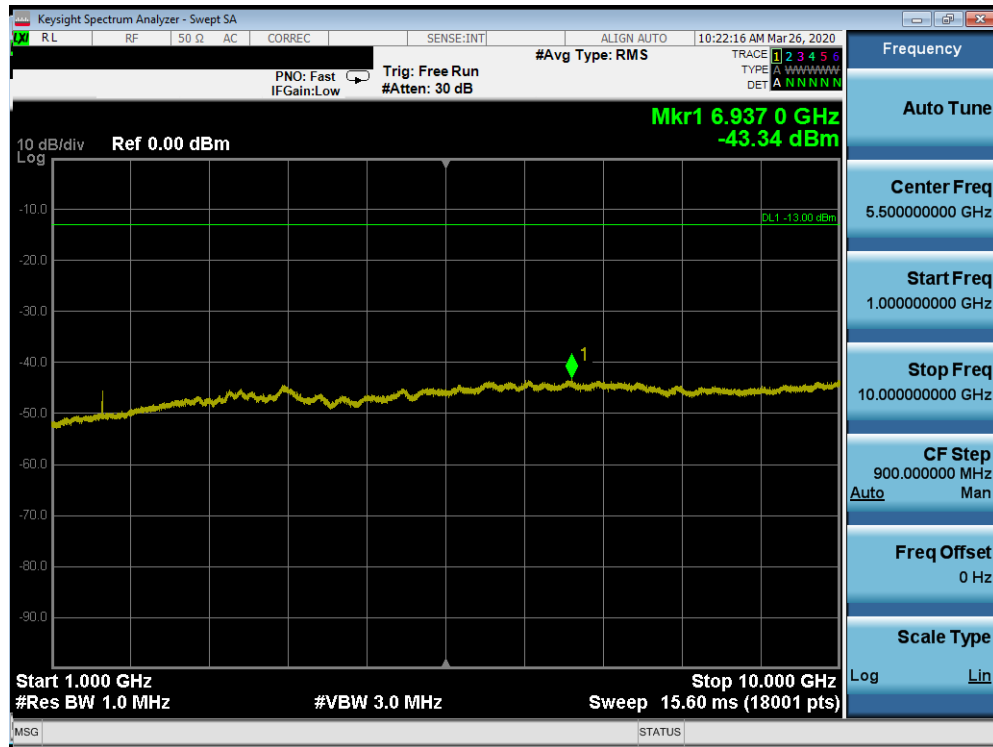
Plot 7-9. Conducted Spurious Plot (LTE Band 14 - 10MHz QPSK - RB Size 1, RB Offset 0)
