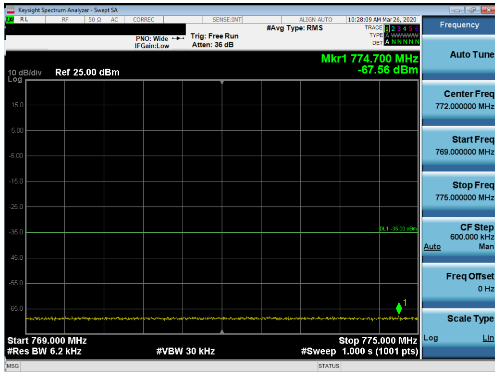
Plot 7-11. Lower Emission Mask Plot (LTE Band 14, 5MHz QPSK - RB Size 25)
