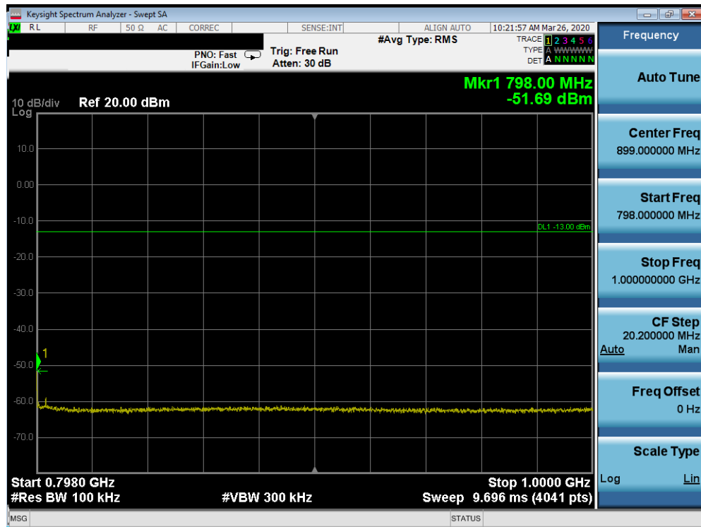
Plot 7-8. Conducted Spurious Plot (LTE Band 14 - 10MHz QPSK - RB Size 1, RB Offset 0)
