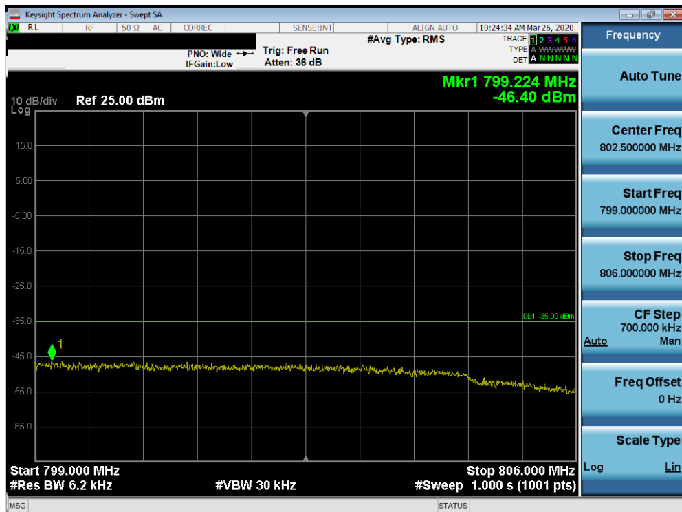
Plot 7-17. Upper Emission Mask Plot (LTE Band 14, 10MHz QPSK - RB Size 50)
