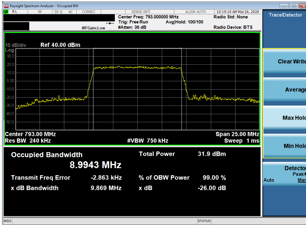
Plot 7-5. Occupied Bandwidth Plot (LTE Band 14 - 10MHz 16-QAM - Full RB Configuration)
