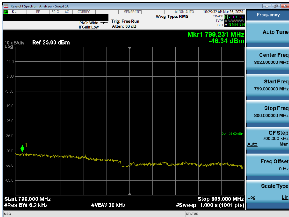
Plot 7-13. Upper Emission Mask Plot (LTE Band 14, 5MHz QPSK - RB Size 25)
