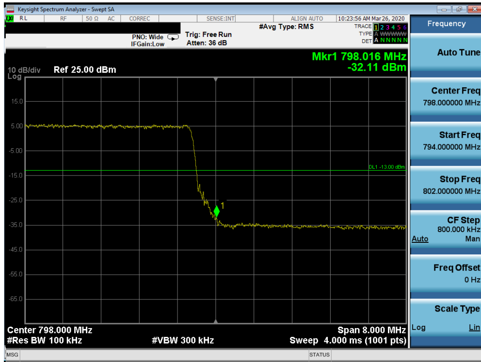
Plot 7-16. Upper Band Edge Plot (LTE Band 14, 10MHz QPSK - RB Size 50)
