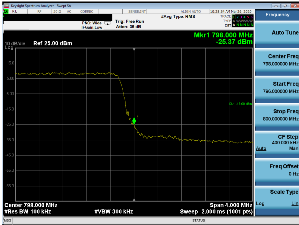
Plot 7-12. Upper Band Edge Plot (LTE Band 14, 5MHz QPSK - RB Size 25)
