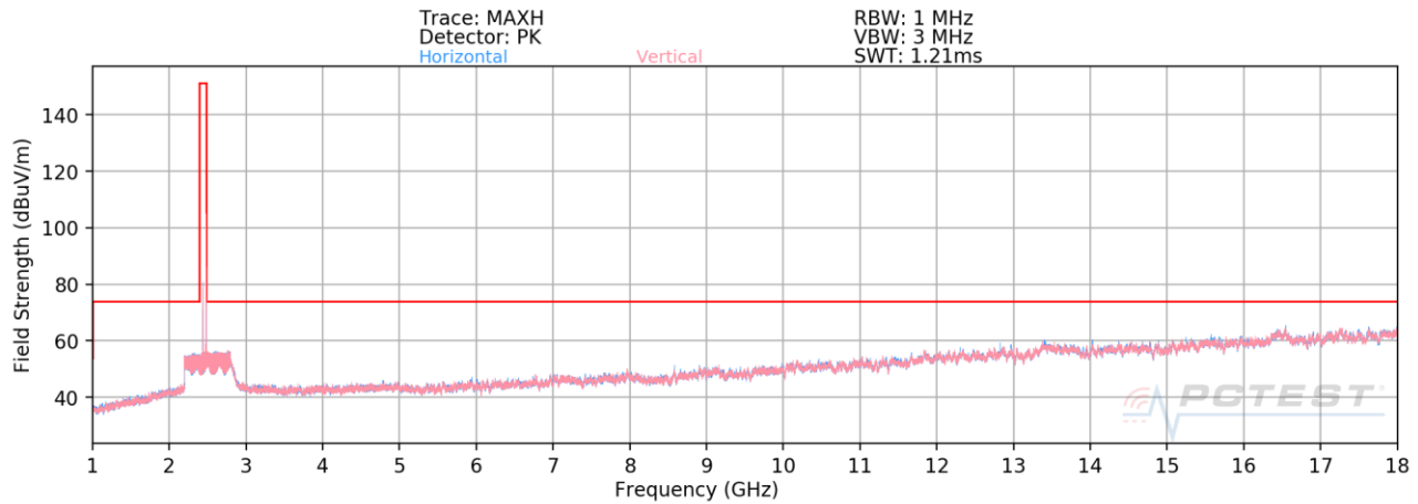
Plot 7-44. Radiated Spurious Plot above 1GHz (BT-Ch. 78)
