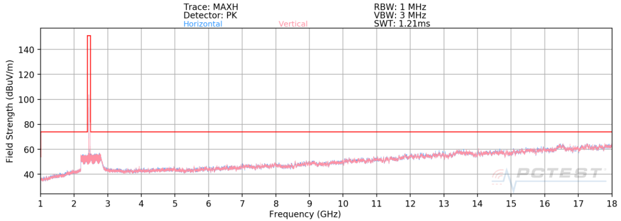
Plot 7-43. Radiated Spurious Plot above 1GHz (BT-Ch. 39)
