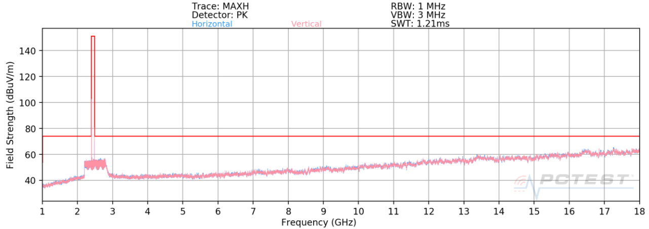
Plot 7-42. Radiated Spurious Plot above 1GHz (BT-Ch. 0)
