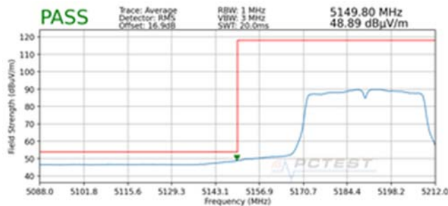
Plot 7-185. Radiated Lower Band Edge Plot SISO ANT1 (Average – UNII Band 1)
