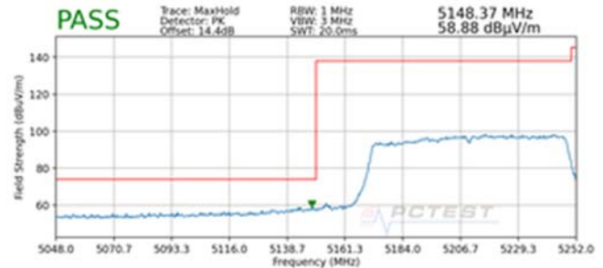
Plot 7-237. Radiated Lower Band Edge Plot MIMO (Peak – UNII Band 1)
