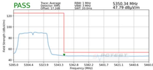
Plot 7-208. Radiated Upper Band Edge Plot SISO ANT2 (Average – UNII Band 2A)
