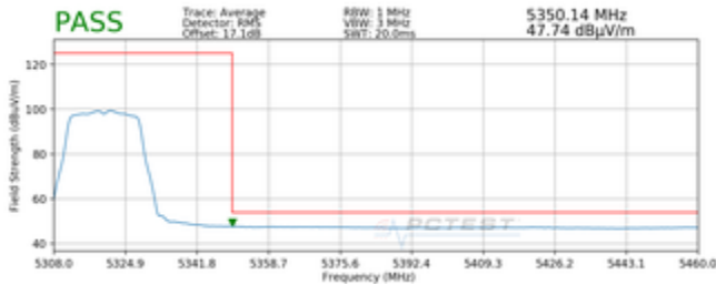
Plot 7-3. Radiated Upper Band Edge Plot SISO ANT1 (Average – UNII Band 2A)
