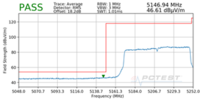
Plot 7-49. Radiated Lower Band Edge Plot MIMO (Average – UNII Band 1)
