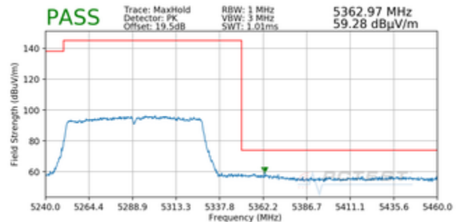
Plot 7-52. Radiated Upper Band Edge Plot MIMO (Peak – UNII Band 2A)
