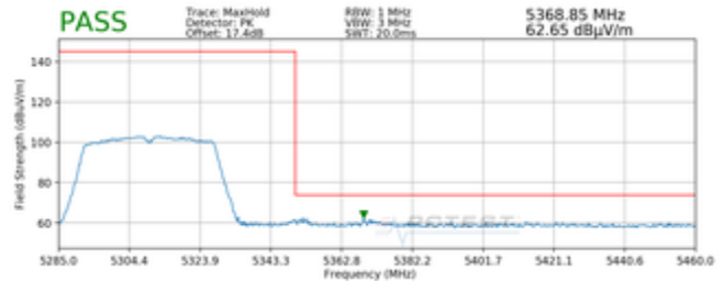
Plot 7-11. Radiated Upper Band Edge Plot SISO ANT1 (Peak – UNII Band 2A)
