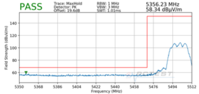
Plot 7-27. Radiated Lower Band Edge Plot CDD (Peak – UNII Band 2C)
