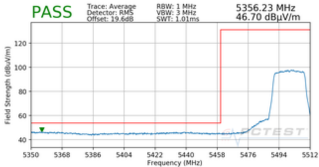
Plot 7-35. Radiated Lower Band Edge Plot MIMO (Average – UNII Band 2C)
