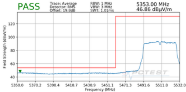
Plot 7-44. Radiated Lower Band Edge Plot MIMO (Average – UNII Band 2C)
