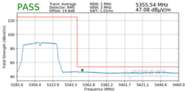
Plot 7-42. Radiated Upper Band Edge Plot MIMO (Average – UNII Band 2A)
