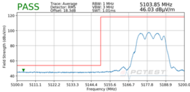
Plot 7-22. Radiated Lower Band Edge Plot CDD (Average – UNII Band 1)
