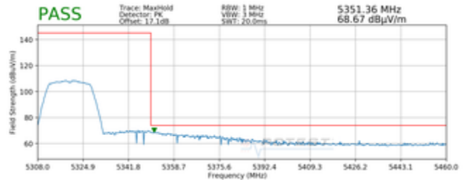
Plot 7-4. Radiated Upper Band Edge Plot SISO ANT1 (Peak – UNII Band 2A)
