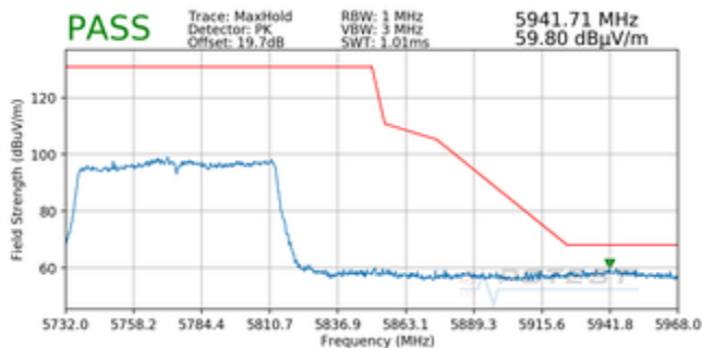
Plot 7-55. Radiated Upper Band Edge Plot MIMO (Peak – UNII Band 3)
