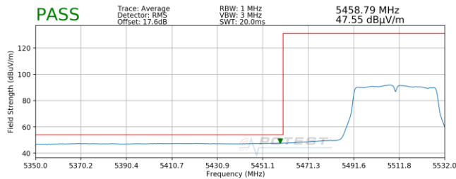
Plot 7-12. Radiated Lower Band Edge Plot SISO ANT1 (Average – UNII Band 2C)
