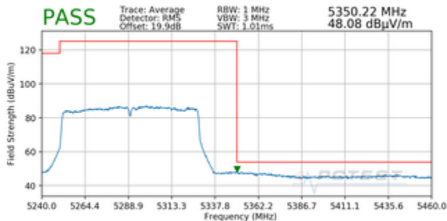
Plot 7-51. Radiated Upper Band Edge Plot MIMO (Average – UNII Band 2A)
