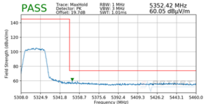
Plot 7-34. Radiated Upper Band Edge Plot MIMO (Peak – UNII Band 2A)
