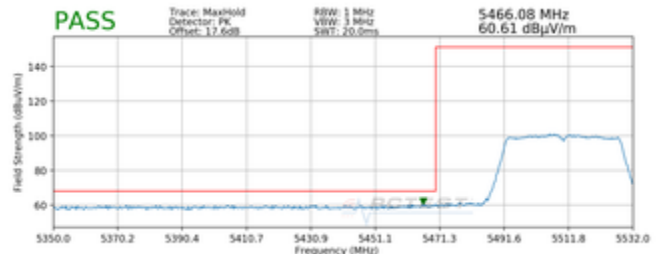
Plot 7-13. Radiated Lower Band Edge Plot SISO ANT1 (Peak – UNII Band 2C)
