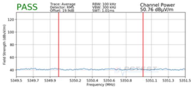
Plot 7-56. Radiated Upper Band Edge Plot MIMO (Average – UNII Band 2A) with Dual Display Cover
