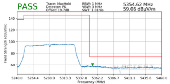
Plot 7-18. Radiated Upper Band Edge Plot SISO ANT1 (Peak – UNII Band 2A)
