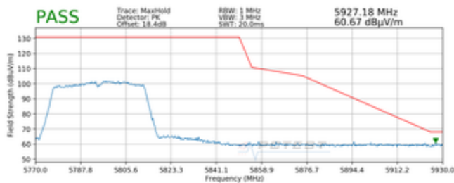
Plot 7-14. Radiated Upper Band Edge Plot SISO ANT1 (Peak – UNII Band 3)
