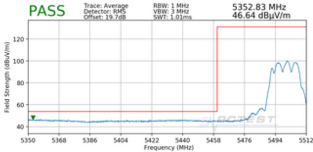
Plot 7-26. Radiated Lower Band Edge Plot CDD (Average – UNII Band 2C)
