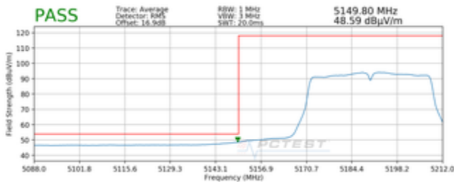
Plot 7-8. Radiated Lower Band Edge Plot SISO ANT1 (Average – UNII Band 1)
