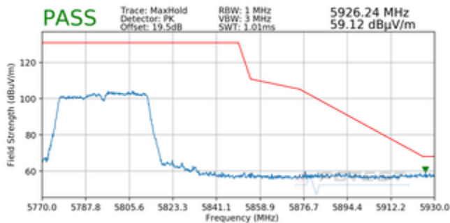
Plot 7-46. Radiated Upper Band Edge Plot MIMO (Peak – UNII Band 3)
