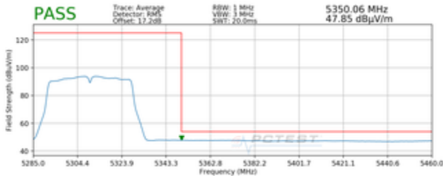
Plot 7-10. Radiated Upper Band Edge Plot SISO ANT1 (Average – UNII Band 2A)
