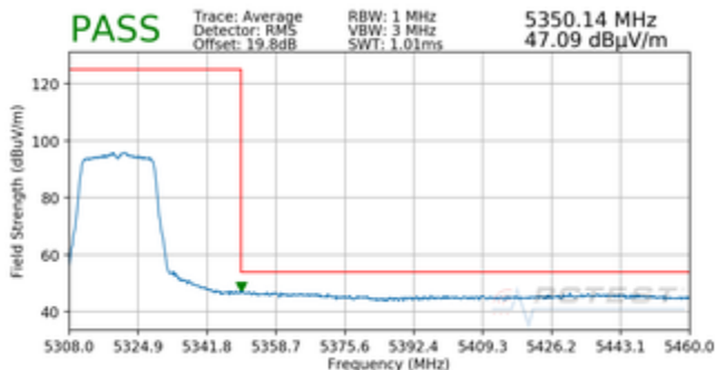
Plot 7-33. Radiated Upper Band Edge Plot MIMO (Average – UNII Band 2A)
