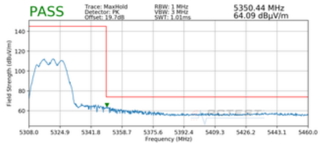
Plot 7-30. Radiated Upper Band Edge Plot CDD (Peak – UNII Band 2A) Dual Display Cover
