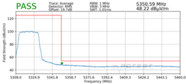
Plot 7-38. Radiated Upper Band Edge Plot MIMO (Average – UNII Band 2A) with Dual Display Cover
