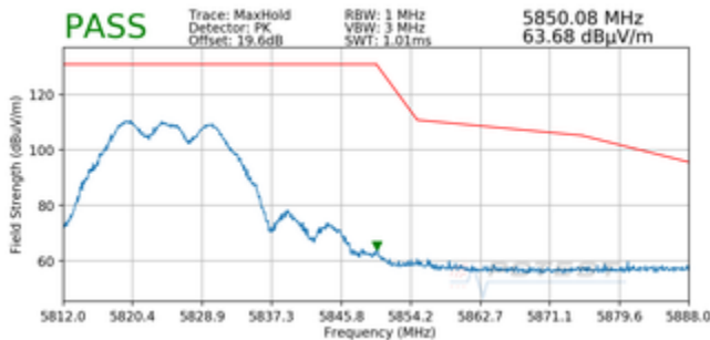
Plot 7-28. Radiated Upper Band Edge Plot CDD (Peak – UNII Band 3)
