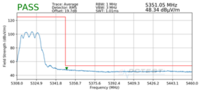
Plot 7-29. Radiated Upper Band Edge Plot CDD (Average – UNII Band 2A) with Dual Display Cover
