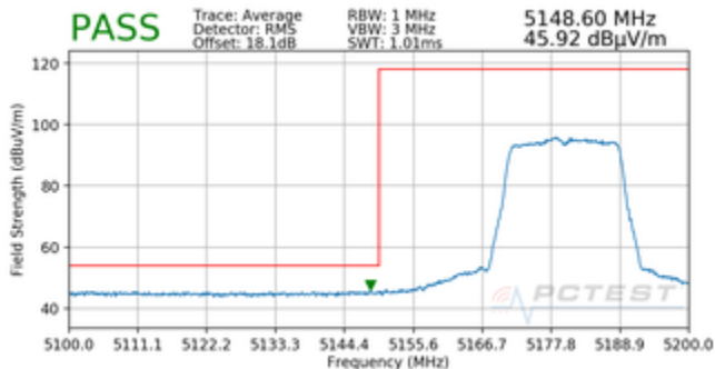
Plot 7-31. Radiated Lower Band Edge Plot MIMO (Average – UNII Band 1)
