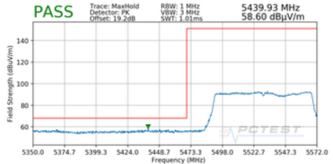
Plot 7-20. Radiated Lower Band Edge Plot SISO ANT1 (Peak – UNII Band 2C)
