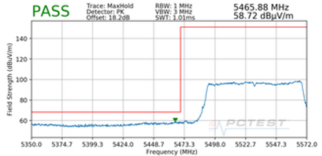
Plot 7-54. Radiated Lower Band Edge Plot MIMO (Peak – UNII Band 2C)
