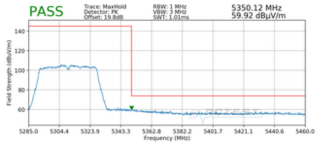
Plot 7-48. Radiated Upper Band Edge Plot MIMO (Peak – UNII Band 2A) with Dual Display Cover
