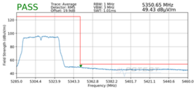
Plot 7-47. Radiated Upper Band Edge Plot MIMO (Average – UNII Band 2A) with Dual Display Cover
