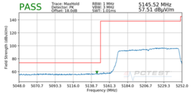
Plot 7-50. Radiated Lower Band Edge Plot MIMO (Peak – UNII Band 1)
