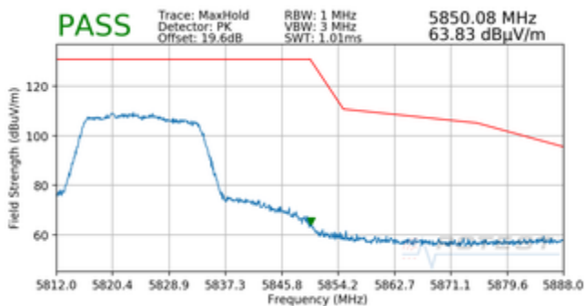
Plot 7-37. Radiated Upper Band Edge Plot MIMO (Peak – UNII Band 3)
