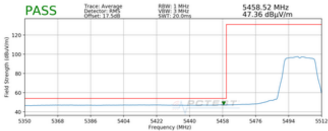
Plot 7-5. Radiated Lower Band Edge Plot SISO ANT1 (Average – UNII Band 2C)
