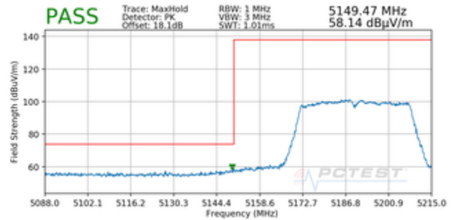
Plot 7-41. Radiated Lower Band Edge Plot MIMO (Peak – UNII Band 1)
