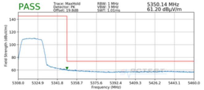
Plot 7-39. Radiated Upper Band Edge Plot MIMO (Peak – UNII Band 2A) with Dual Display Cover
