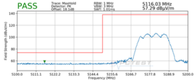
Plot 7-23. Radiated Lower Band Edge Plot CDD (Peak – UNII Band 1)
