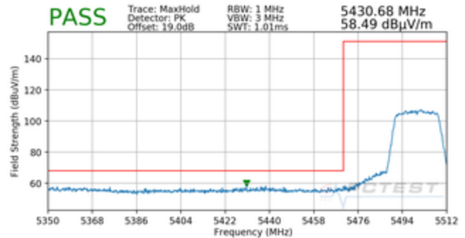
Plot 7-36. Radiated Lower Band Edge Plot MIMO (Peak – UNII Band 2C)
