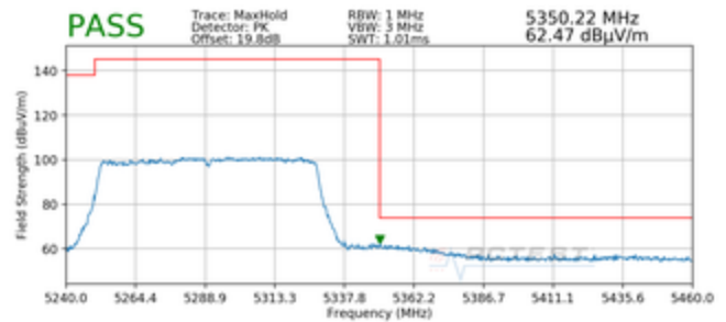
Plot 7-57. Radiated Upper Band Edge Plot MIMO (Peak – UNII Band 2A) with Dual Display Cover
