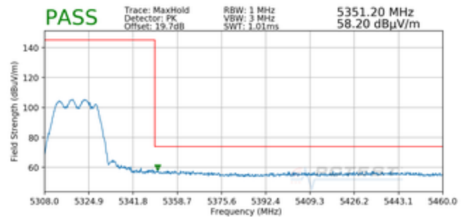
Plot 7-25. Radiated Upper Band Edge Plot CDD (Peak – UNII Band 2A)
