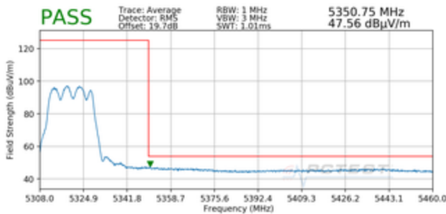
Plot 7-24. Radiated Upper Band Edge Plot CDD (Average – UNII Band 2A)
