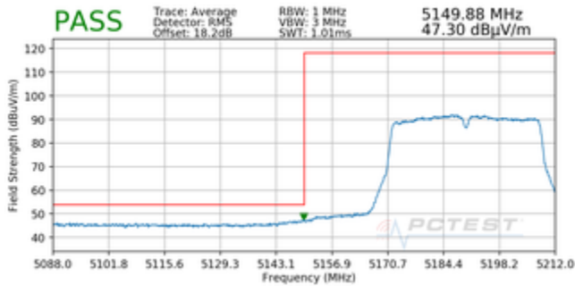
Plot 7-40. Radiated Lower Band Edge Plot MIMO (Average – UNII Band 1)
