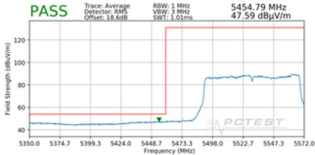
Plot 7-53. Radiated Lower Band Edge Plot MIMO (Average – UNII Band 2C)
