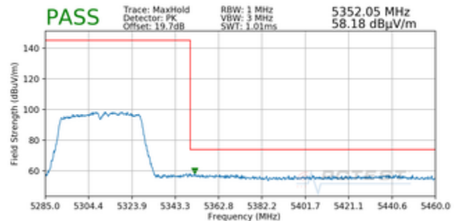
Plot 7-43. Radiated Upper Band Edge Plot MIMO (Peak – UNII Band 2A)
