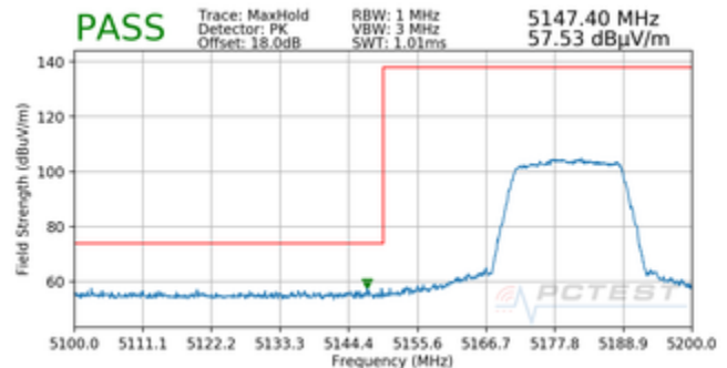
Plot 7-32. Radiated Lower Band Edge Plot MIMO (Peak – UNII Band 1)
