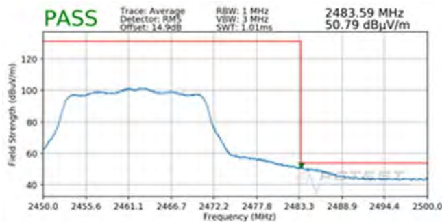
Plot 7-95. Radiated Restricted Upper Band Edge Measurement MIMO (Average)
