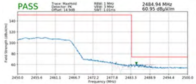
Plot 7-94. Radiated Restricted Upper Band Edge Measurement MIMO (Peak)
