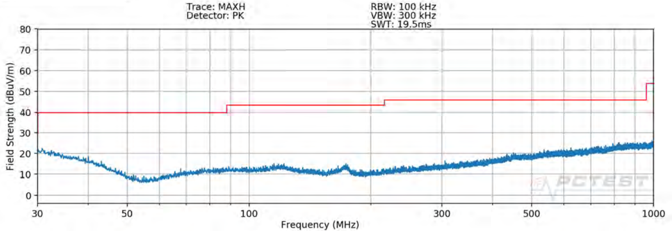
Plot 7-99. Radiated Spurious Plot below 1GHz SISO ANT1
