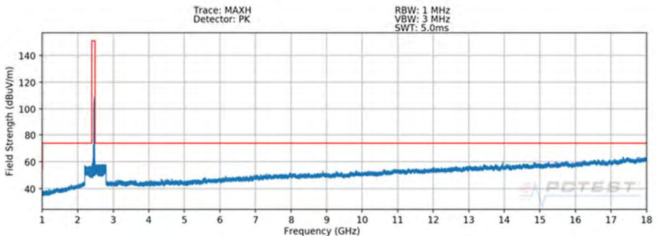
Plot 7-63. Radiated Spurious Plot above 1GHz SISO ANT1 (802.11b – Ch. 11)
