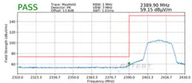
Plot 7-82. Radiated Restricted Lower Band Edge Measurement SISO ANT2 (Peak)
