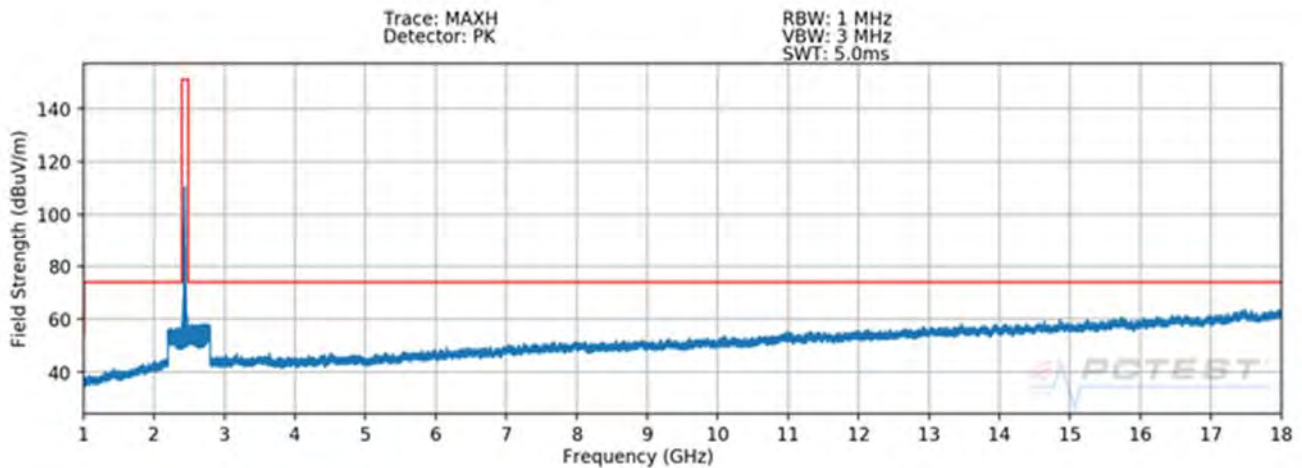
Plot 7-62. Radiated Spurious Plot above 1GHz SISO ANT1 (802.11b – Ch. 6)
