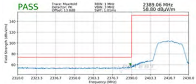
Plot 7-84. Radiated Restricted Lower Band Edge Measurement SISO ANT2 (Peak)
