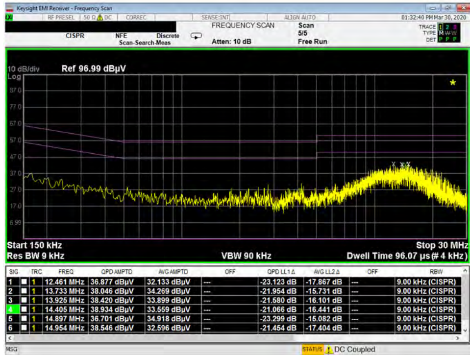
Plot 7-101. Line Conducted Plot with 802.11b (L1)
