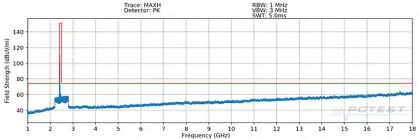
Plot 7-69. Radiated Spurious Plot above 1GHz MIMO/CDD (802.11g – Ch. 1)
