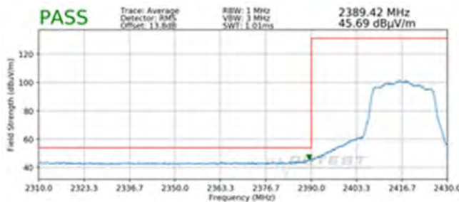
Plot 7-75. Radiated Restricted Lower Band Edge Measurement SISO ANT1 (Average)
