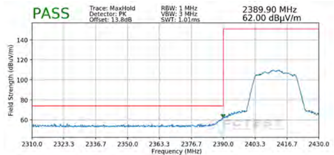
Plot 7-90. Radiated Restricted Lower Band Edge Measurement MIMO (Peak)
