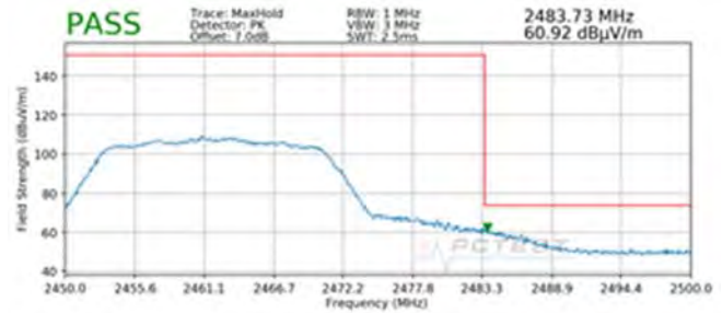
Plot 7-98. Radiated Restricted Band Edge Measurement MIMO with WCP (Peak)
