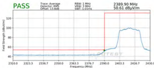
Plot 7-73. Radiated Restricted Lower Band Edge Measurement SISO ANT1 (Average)
