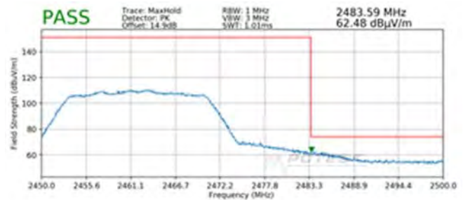
Plot 7-96. Radiated Restricted Upper Band Edge Measurement MIMO (Peak)
