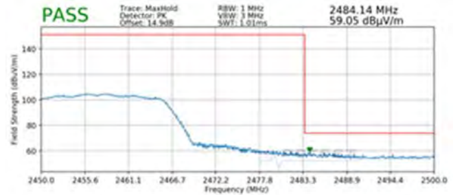
Plot 7-86. Radiated Restricted Upper Band Edge Measurement SISO ANT2 (Peak)
