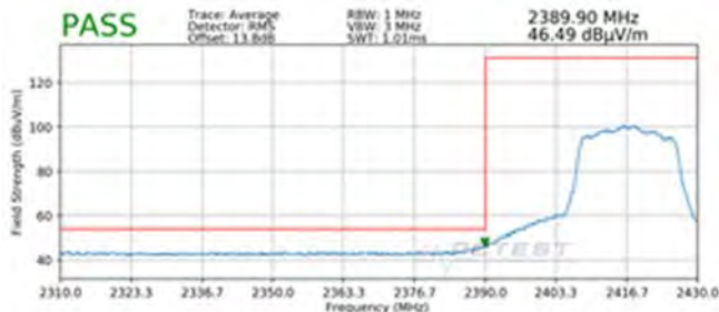
Plot 7-91. Radiated Restricted Lower Band Edge Measurement MIMO (Average)
