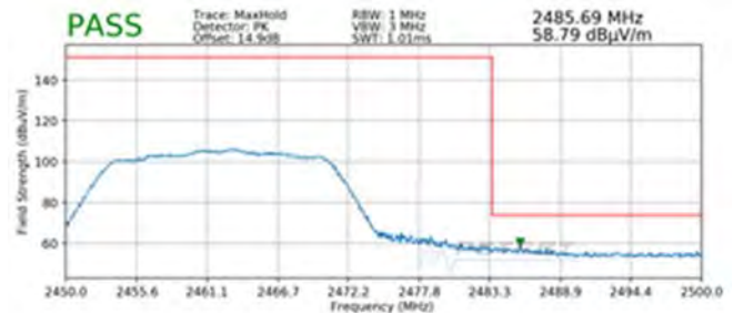
Plot 7-88. Radiated Restricted Upper Band Edge Measurement SISO ANT2 (Peak)
