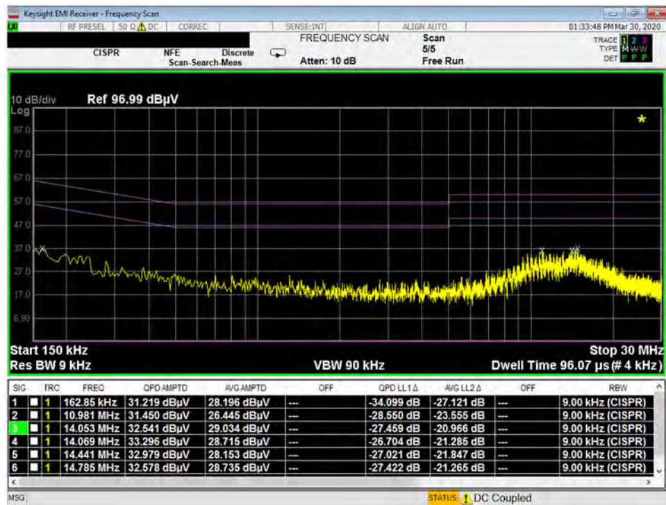
Plot 7-102. Line Conducted Plot with 802.11b (N)
