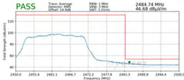
Plot 7-87. Radiated Restricted Upper Band Edge Measurement SISO ANT2 (Average)
