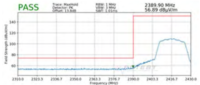
Plot 7-76. Radiated Restricted Lower Band Edge Measurement SISO ANT1 (Peak)
