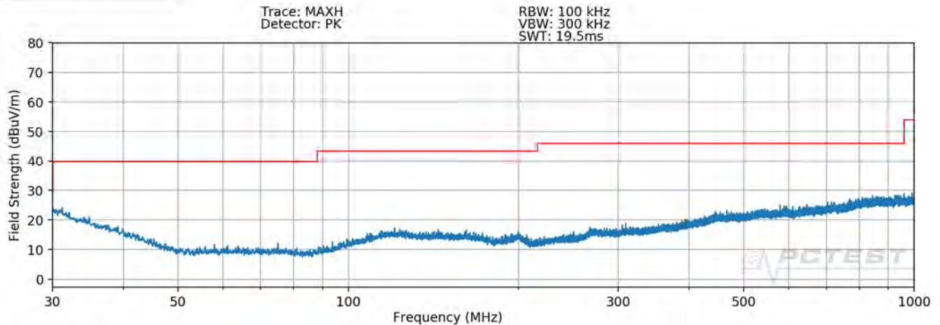
Plot 7-100. Radiated Spurious Plot below 1GHz SISO ANT2
