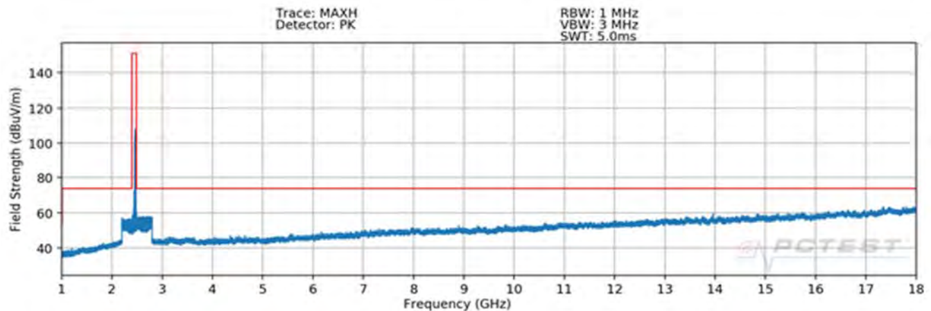
Plot 7-71. Radiated Spurious Plot above 1GHz MIMO/CDD (802.11g – Ch. 11)
