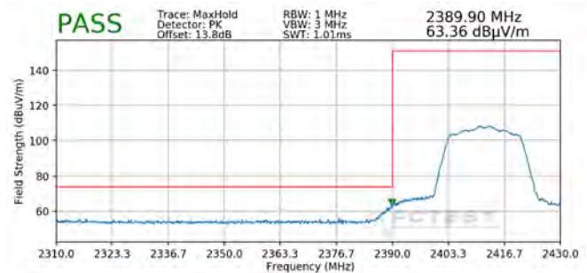
Plot 7-74. Radiated Restricted Lower Band Edge Measurement SISO ANT1 (Peak)
