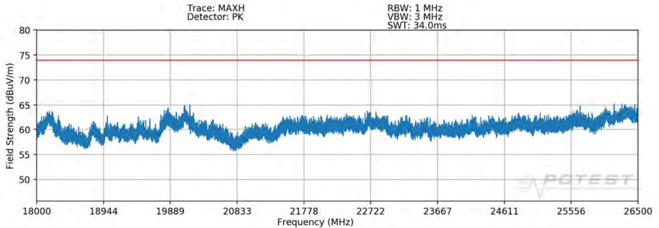
Plot 7-72. Radiated Spurious Plot above 18GHz MIMO/CDD
