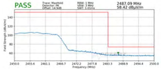
Plot 7-78. Radiated Restricted Upper Band Edge Measurement SISO ANT1 (Peak)
