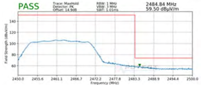
Plot 7-80. Radiated Restricted Upper Band Edge Measurement SISO ANT1 (Peak)
