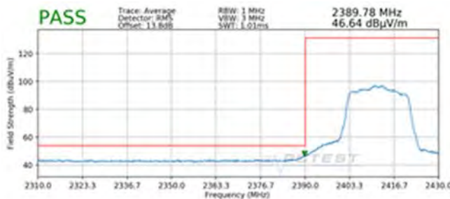
Plot 7-81. Radiated Restricted Lower Band Edge Measurement SISO ANT2 (Average)
