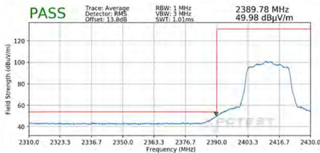
Plot 7-89. Radiated Restricted Lower Band Edge Measurement MIMO (Average)
