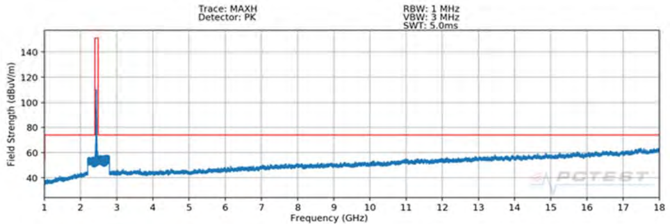
Plot 7-70. Radiated Spurious Plot above 1GHz MIMO/CDD (802.11g – Ch. 6)
