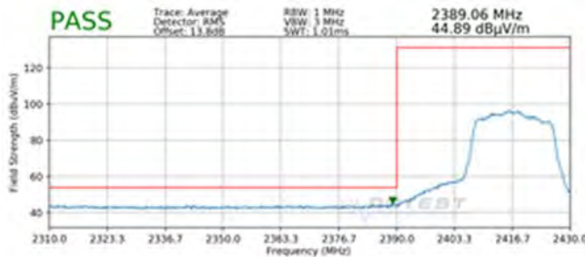
Plot 7-83. Radiated Restricted Lower Band Edge Measurement SISO ANT2 (Average)
