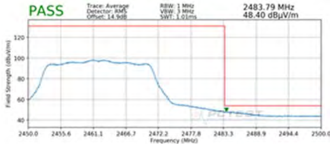
Plot 7-79. Radiated Restricted Upper Band Edge Measurement SISO ANT1 (Average)
