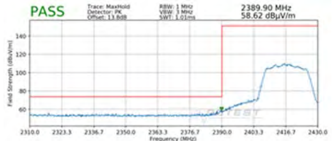
Plot 7-92. Radiated Restricted Lower Band Edge Measurement MIMO (Peak)
