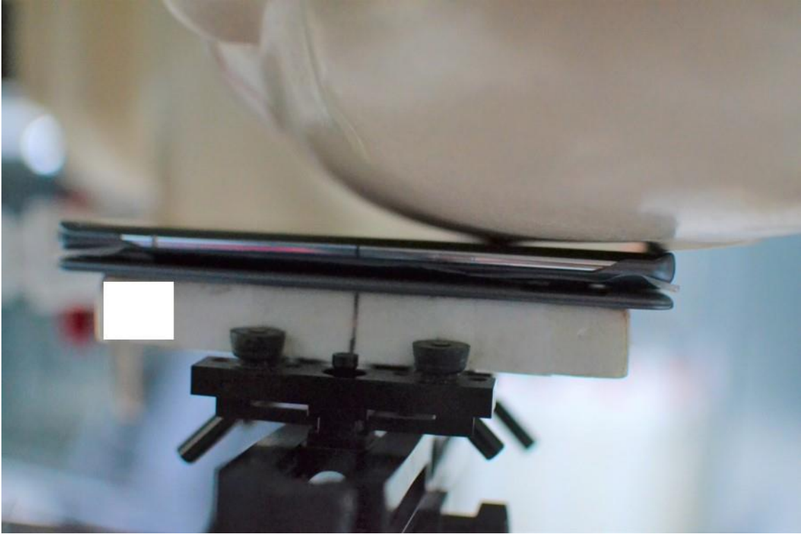
SAR Test Setup Photo 7 – Left Cheek with Dual Display Accessory Position #3
