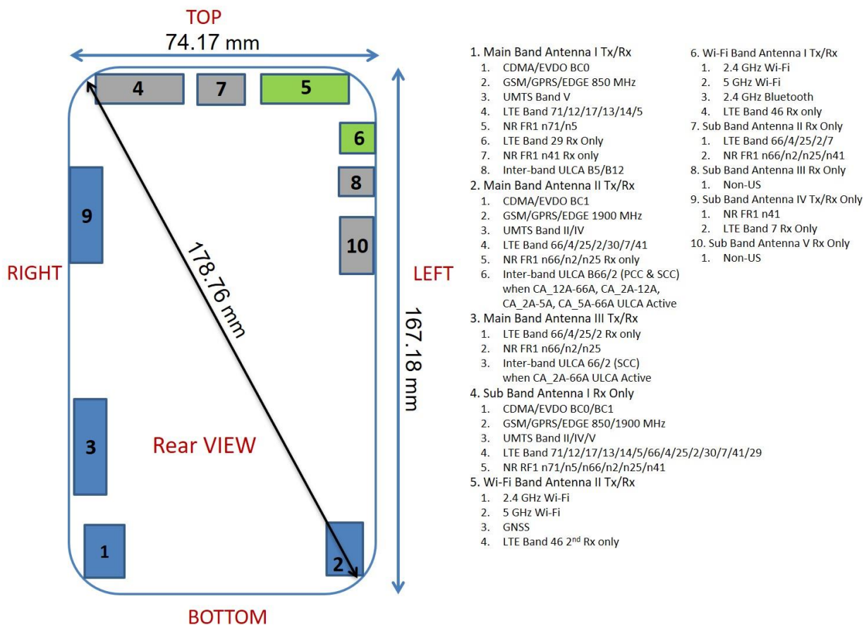
Figure E-1 DUT Antenna Locations
