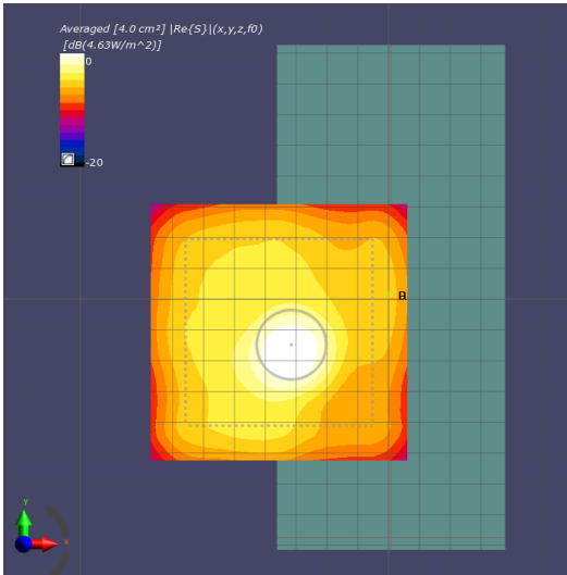
Figure 12-2 4cm 2 psPD distribution measured at input.power.limit of 4.5 dBm on the back surface for n260 beam 31
