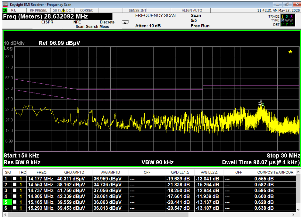
Plot 7-9. Line-Conducted Test Plot (N, Antenna Removed)
