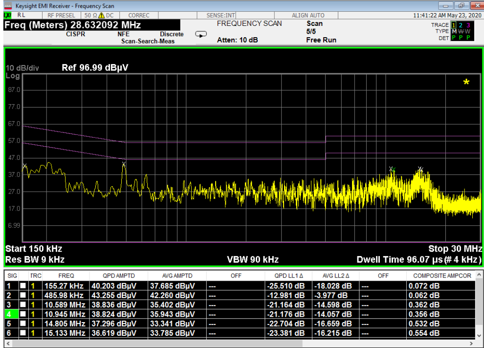
Plot 7-8. Line-Conducted Test Plot (L1, Antenna Removed)
