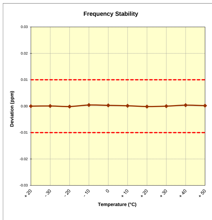
Figure 7-3. Frequency Stability Plot
