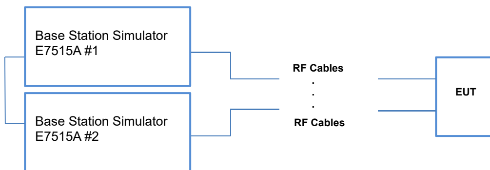
Figure E.3.1 DL 4CA Power Measurement Setup
