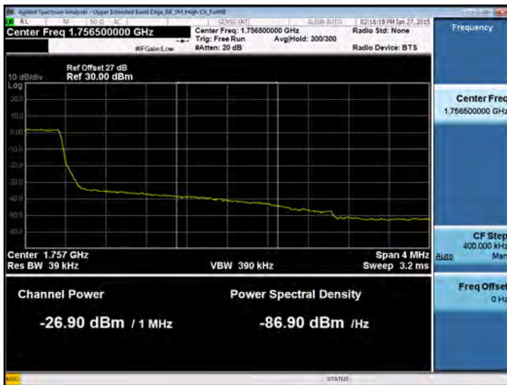
BAND 4. Upper Extended Band Edge Plot (3M BW Ch.20385 QPSK_RB15_0) -3
