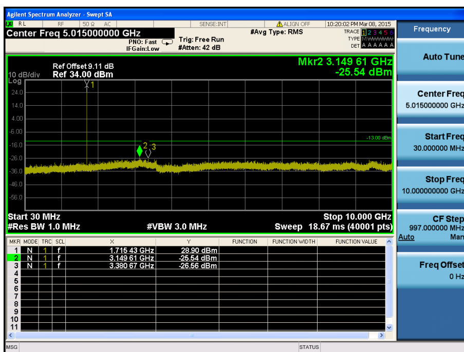
LTE Band 4 / 10MHz / 16QAM - RB Size/Offset (1/25) – Low Channel
