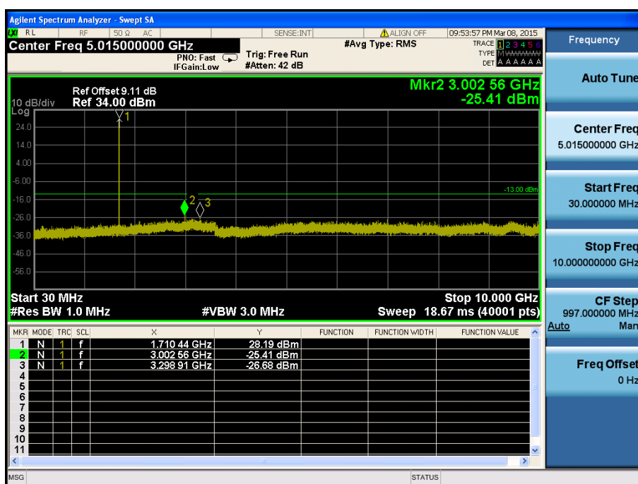
LTE Band 4 / 3MHz / 16QAM - RB Size/Offset (1/0) – Low Channel
