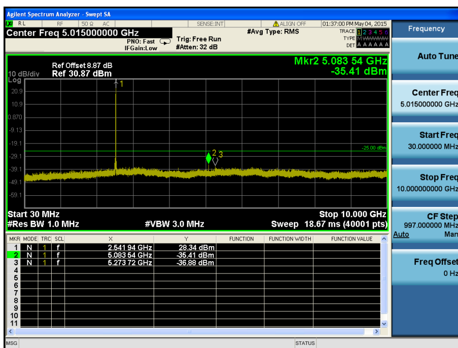
LTE Band 7 / 15MHz / QPSK - RB Size/Offset (1/74) – Mid Channel
