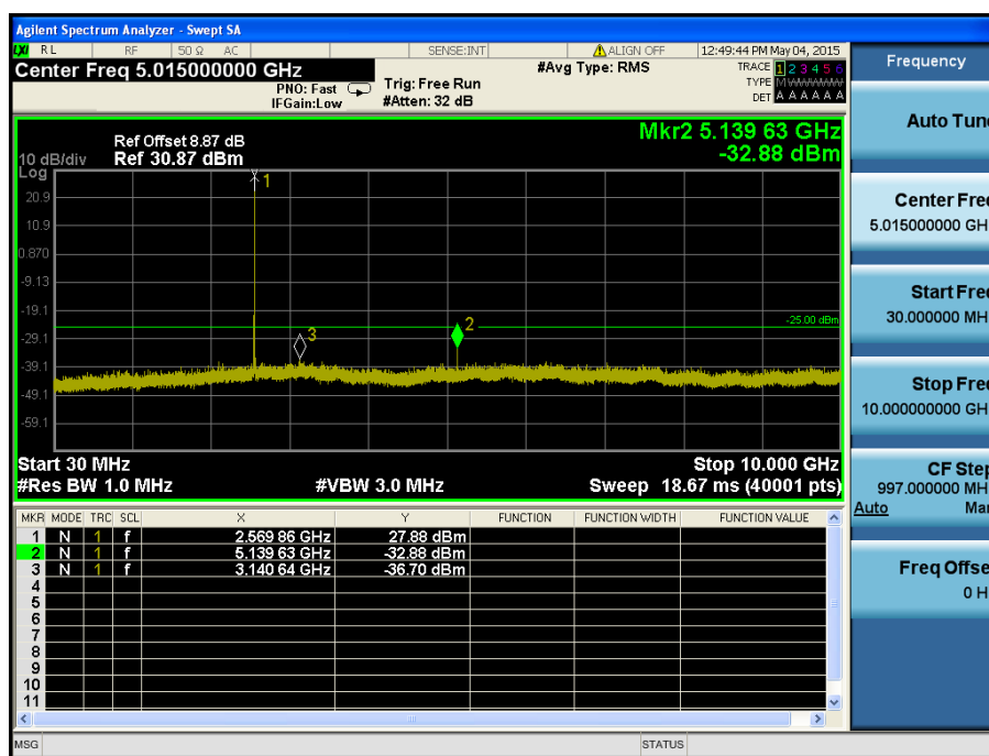
LTE Band 7 / 5MHz / QPSK - RB Size/Offset (1/24) – High Channel
