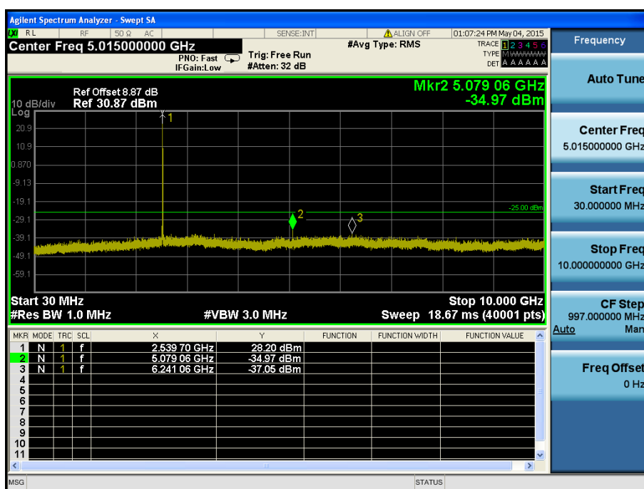
LTE Band 7 / 10MHz / QPSK - RB Size/Offset (1/49) – Mid Channel
