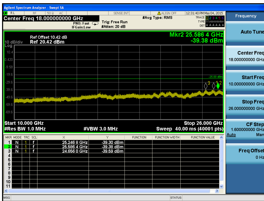
LTE Band 7 / 5MHz / QPSK - RB Size/Offset (1/0) – Low Channel
