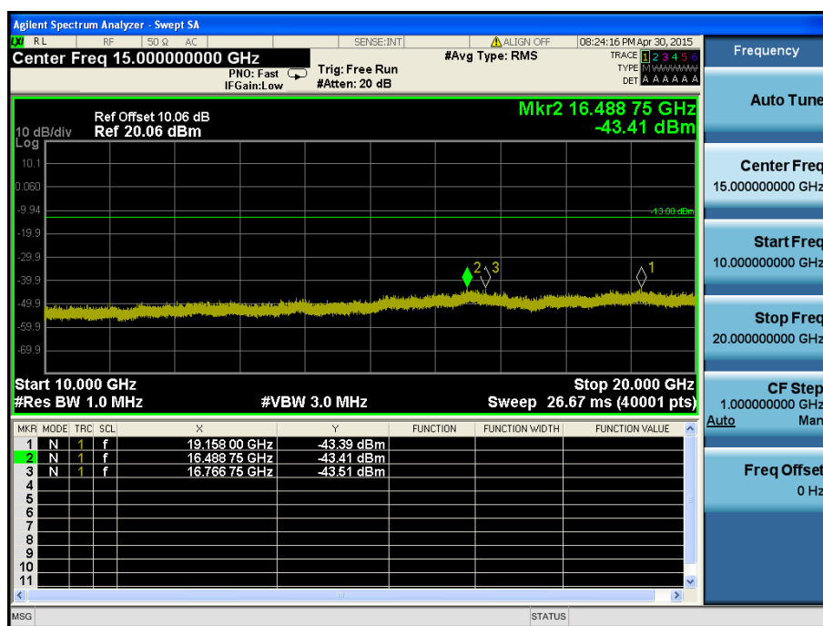
LTE Band 2 / 20MHz / 16QAM - RB Size/Offset (1/50) – Low Channel
