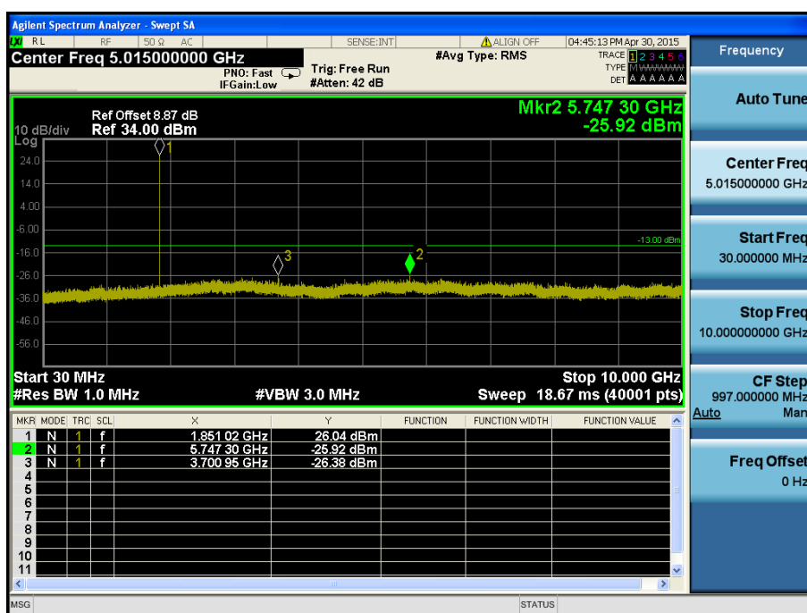
LTE Band 2 / 1.4MHz / 16QAM - RB Size/Offset (6/0) – Low Channel
