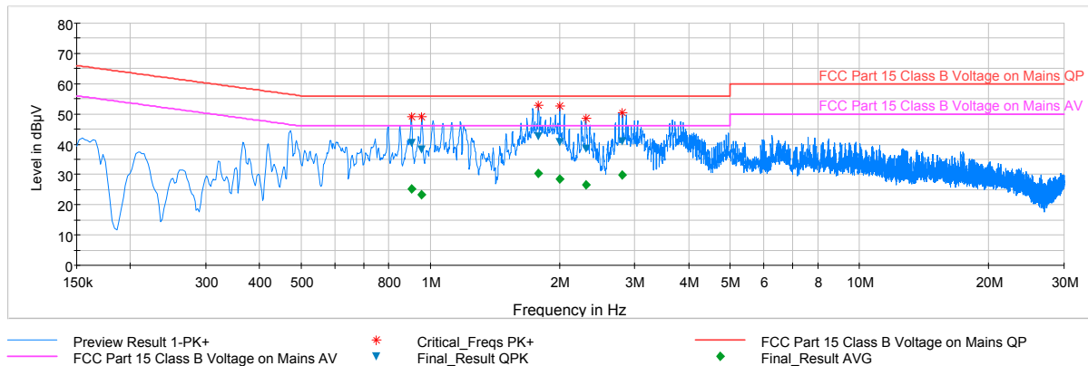
Plot 6-30. Line Conducted Plot with Bluetooth LE (L1)
