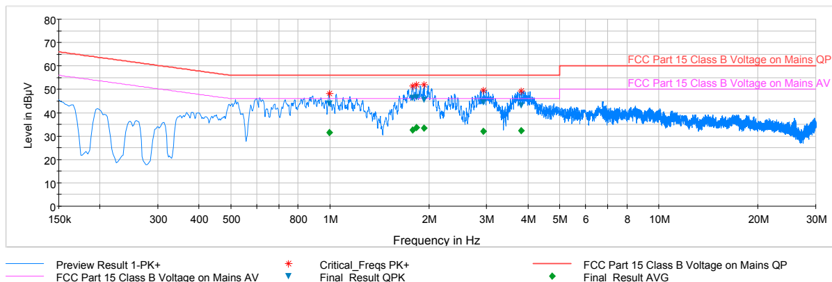
Plot 6-31. Line Conducted Plot with Bluetooth LE (N)
