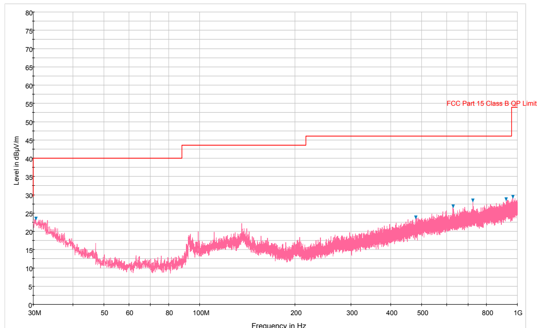
Plot 6-28. Radiated Spurious Plot below 1GHz (Pol. H)
