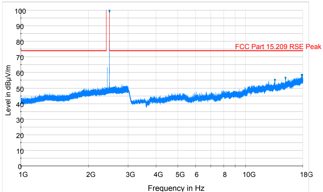
Plot 6-23. Radiated Spurious Plot above 1GHz (BTLE – Ch. 39, Ant. Pol. V)
