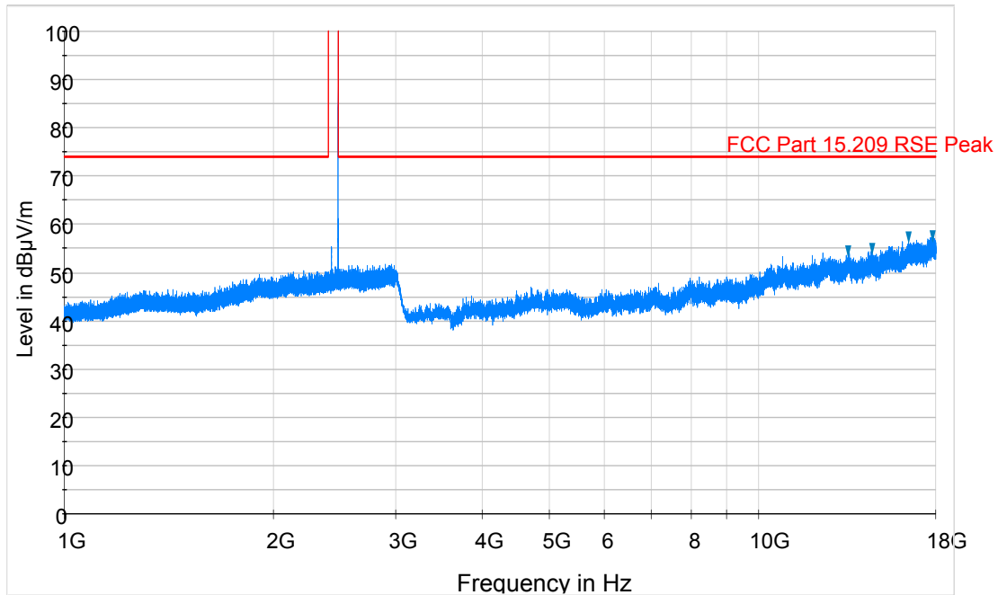
Plot 6-22. Radiated Spurious Plot above 1GHz (BTLE – Ch. 39, Ant. Pol. H)
