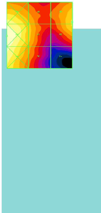
Figure 10-1 Sample E-field Scan Overlay (T-Coil Centered Scan pictured. See Test Setup Photographs for Acoustic Scan Overlay and actual WD overlay)
