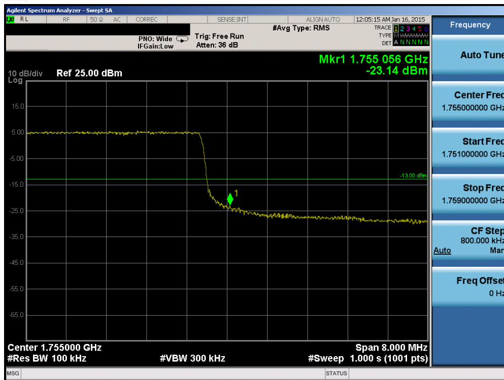
Plot 6-90. Upper Band Edge Plot (Band 4 – 10.0MHz QPSK – RB Size 50)
