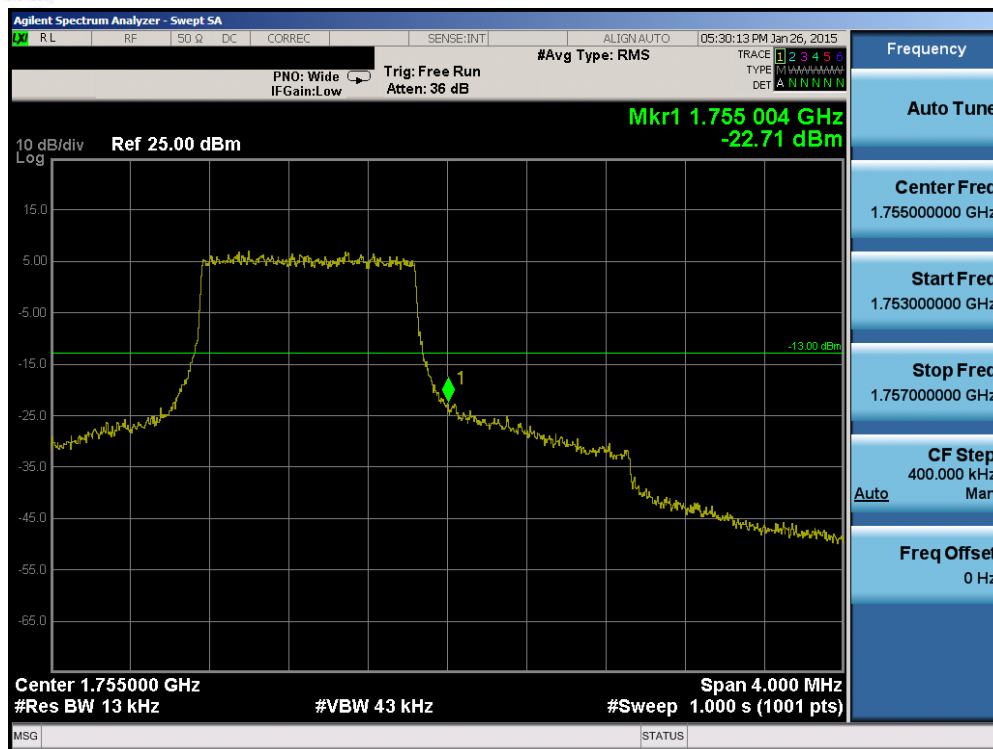
Plot 6-78. Upper Band Edge Plot (Band 4 – 1.4MHz QPSK – RB Size 6)
