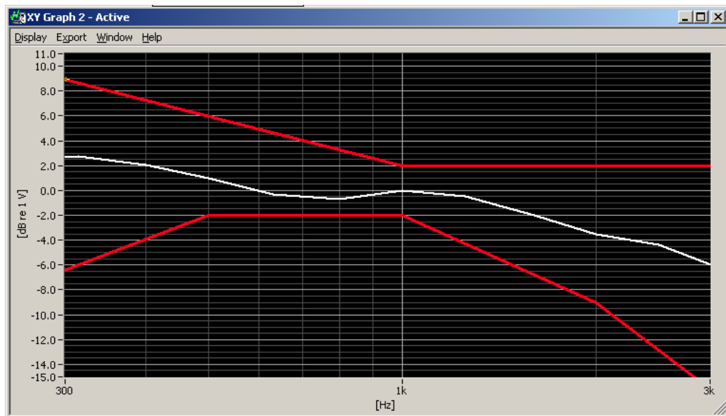
Figure 6-1 Axial Frequency Response
