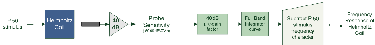
Figure 4-13 Frequency Response Block Diagram
