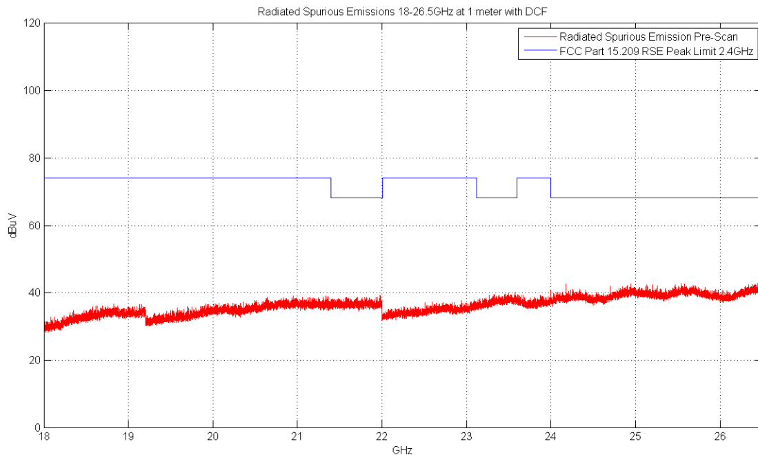
Plot 6-53. Radiated Spurious Plot above 18GHz (Pol. V)
