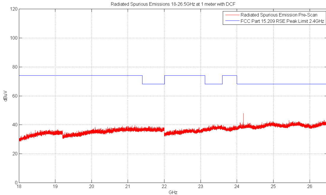
Plot 6-52. Radiated Spurious Plot above 18GHz (Pol. H)
