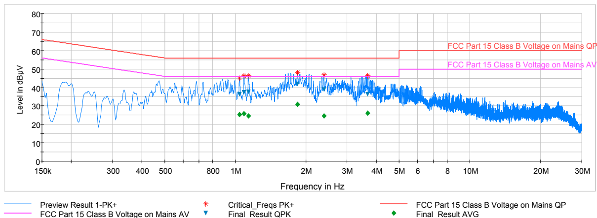
Plot 6-54. Line-Conducted Test Plot (L1)
