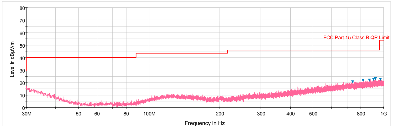
Plot 6-50. Radiated Spurious Plot below 1GHz (Pol. H)
