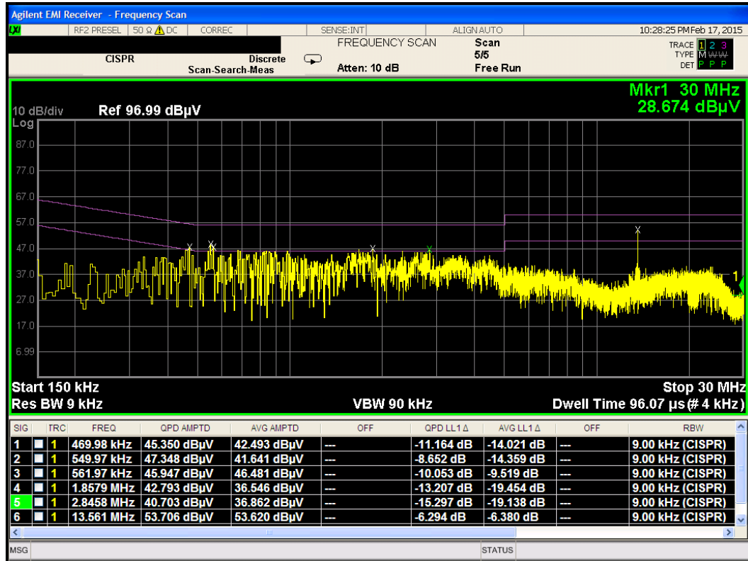
Plot 7-2. Line-Conducted Test Plot (N)
