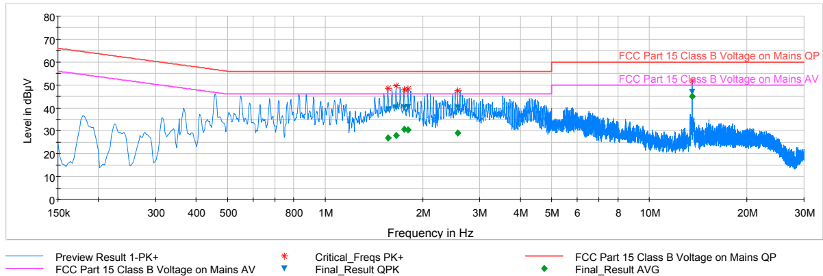
Plot 7-1. Line-Conducted Test Plot (L1)
