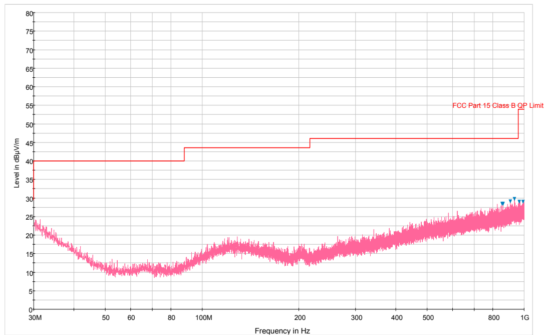
Plot 6-53. Radiated Spurious Plot below 1GHz (Pol. V)
