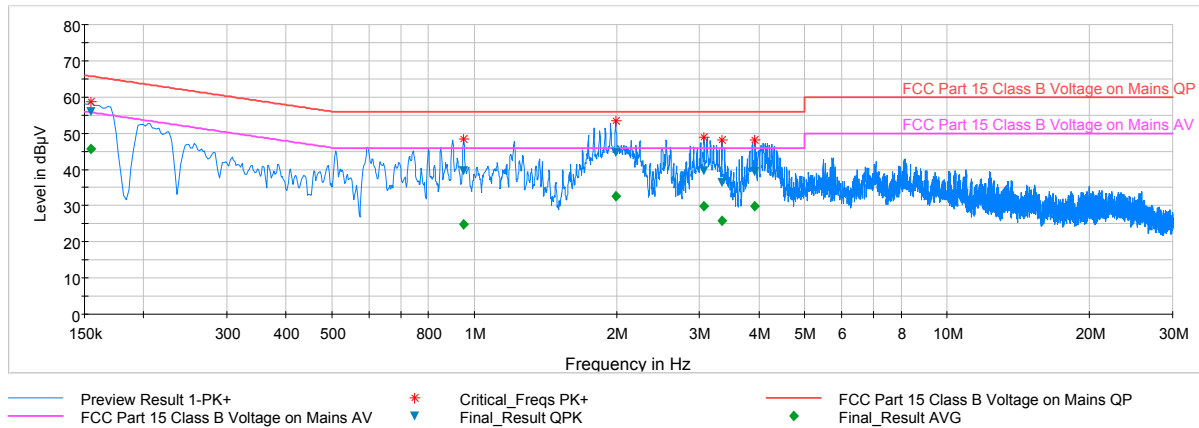
Plot 6-54. Line-Conducted Test Plot (L1)
