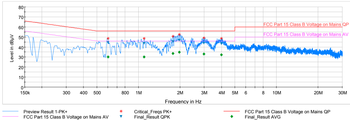
Plot 6-55. Line-Conducted Test Plot (N)
