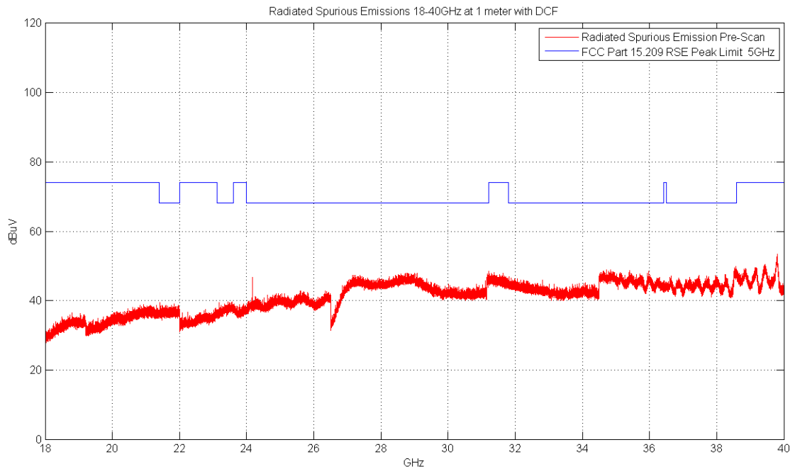
Plot 6-95. Radiated Spurious Plot above 18GHz (802.11a – Ant. Pol. H)
