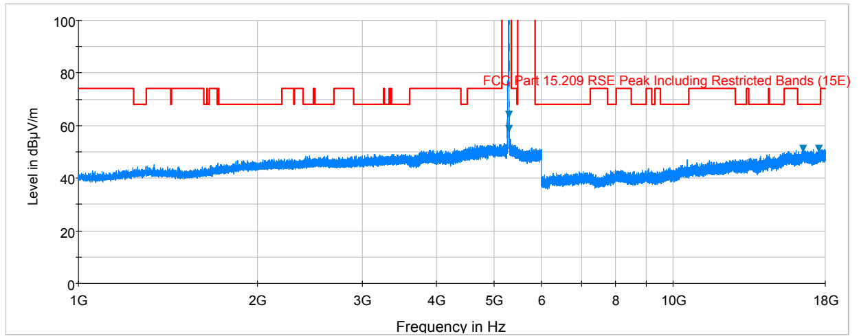
Plot 6-69. Radiated Spurious Plot above 1GHz (802.11a – U2A, Ant. Pol. H)
