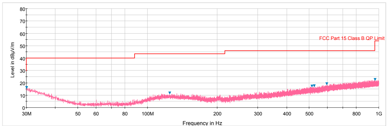
Plot 6-94. Radiated Spurious Plot below 1GHz (802.11a – U3, Ant. Pol. V)
