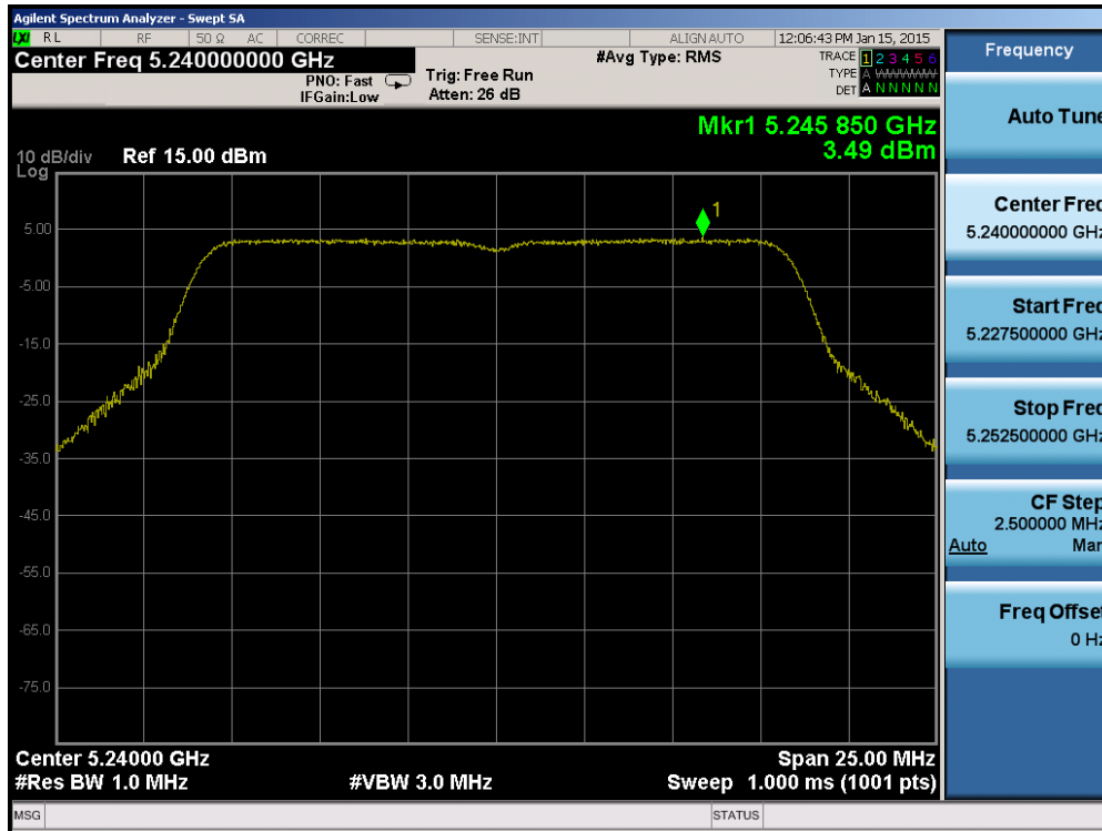
Plot 6-36. Peak Power Spectral Density Plot (802.11a (UNII Band 1) – Ch. 48)
