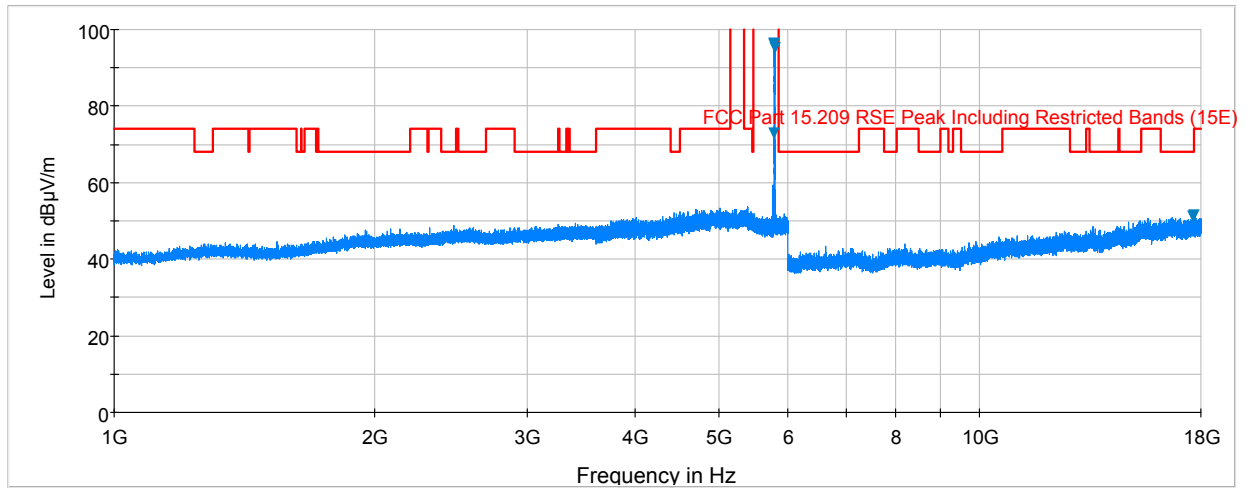
Plot 6-74. Radiated Spurious Plot above 1GHz (802.11a – U3, Ant. Pol. V)
