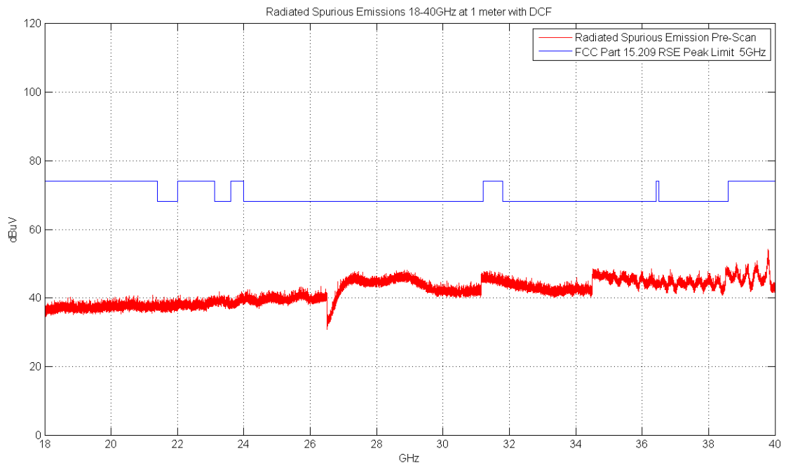
Plot 6-96. Radiated Spurious Plot above 18GHz (802.11a – Ant. Pol. V)
