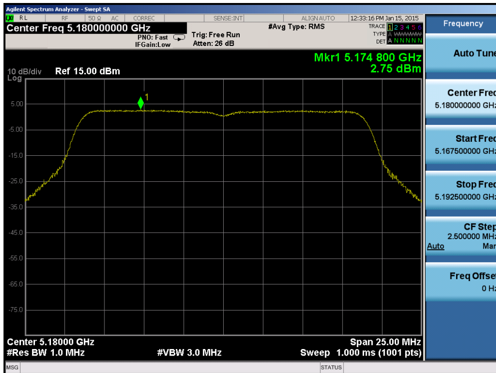
Plot 6-37. Peak Power Spectral Density Plot (20MHz BW 802.11n (UNII Band 1) – Ch. 36)
