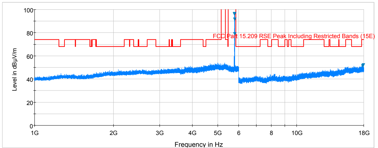
Plot 6-73. Radiated Spurious Plot above 1GHz (802.11a – U3, Ant. Pol. H)
