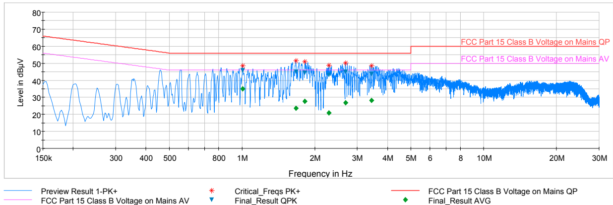
Plot 6-98. Line Conducted Plot with 802.11a UNII Band 1 (N)
