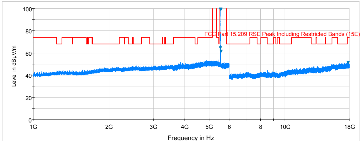
Plot 6-72. Radiated Spurious Plot above 1GHz (802.11a – U2C, Ant. Pol. V)
