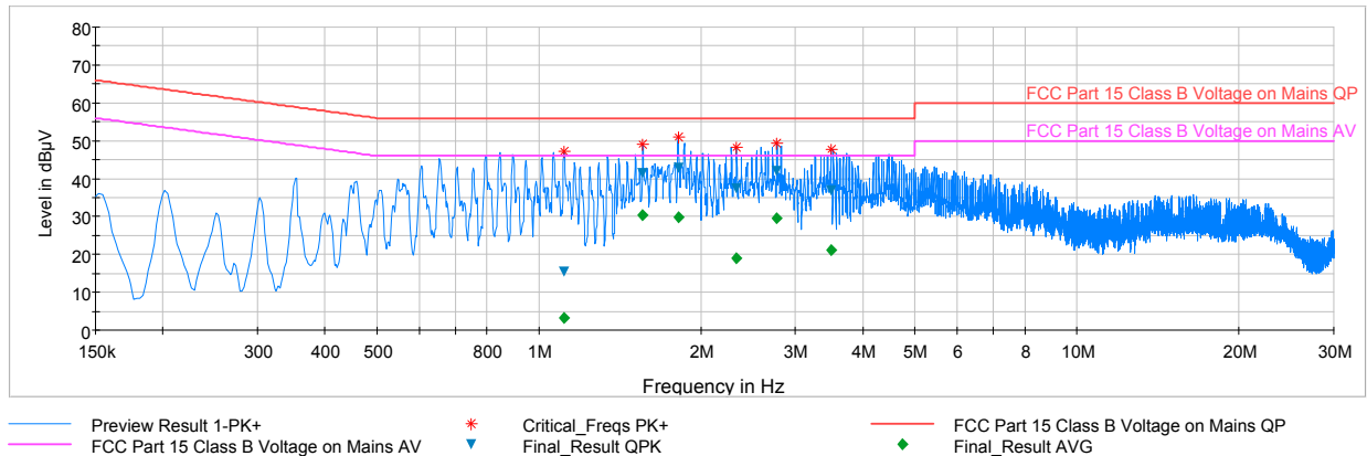
Plot 6-99. Line Conducted Plot with 802.11a UNII Band 2A (L1)
