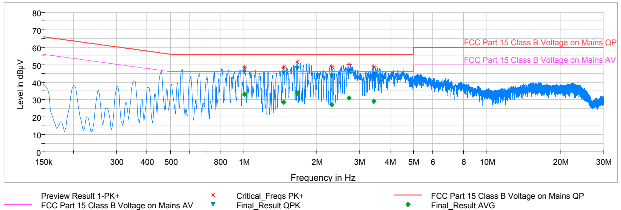
Plot 6-100. Line Conducted Plot with 802.11a UNII Band 2A (N)
