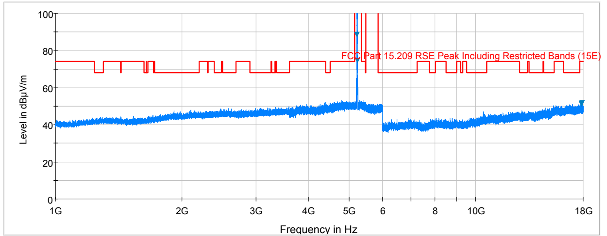
Plot 6-68. Radiated Spurious Plot above 1GHz (802.11a – U1, Ant. Pol. V)
