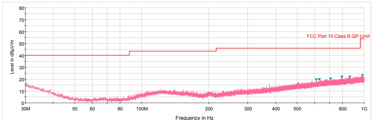
Plot 6-93. Radiated Spurious Plot below 1GHz (802.11a – U3, Ant. Pol. H)
