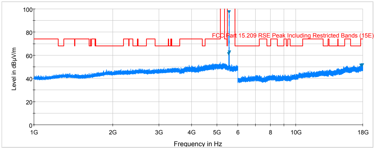
Plot 6-71. Radiated Spurious Plot above 1GHz (802.11a – U2C, Ant. Pol. H)
