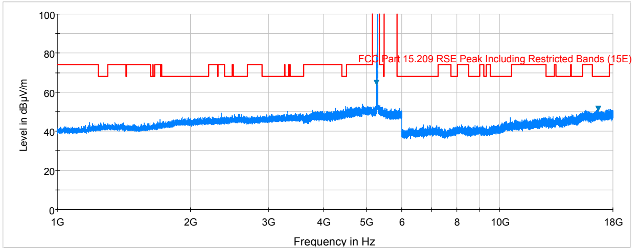
Plot 6-70. Radiated Spurious Plot above 1GHz (802.11a – U2A, Ant. Pol. V)
