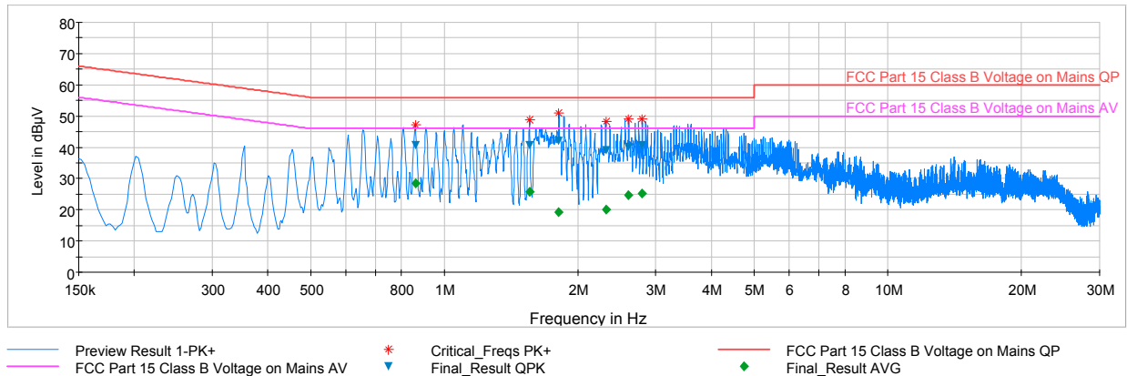
Plot 6-101. Line Conducted Plot with 802.11a UNII Band 2C (L1)
