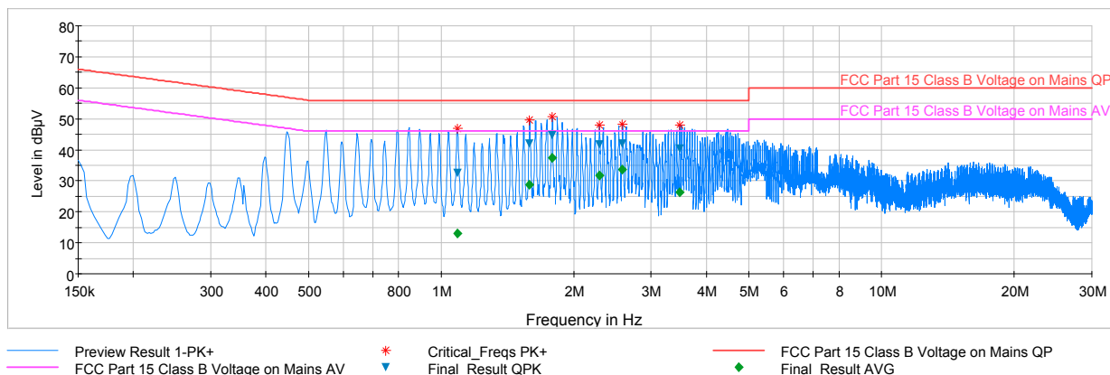
Plot 6-97. Line Conducted Plot with 802.11a UNII Band 1 (L1)
