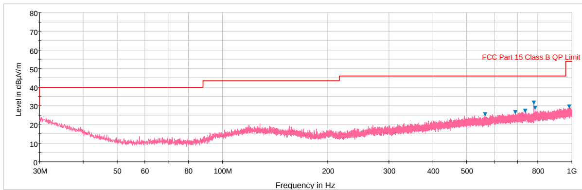
Plot 6-96. Radiated Spurious Plot below 1GHz (802.11a – U3 Ch. 157, Ant. Pol. V)
