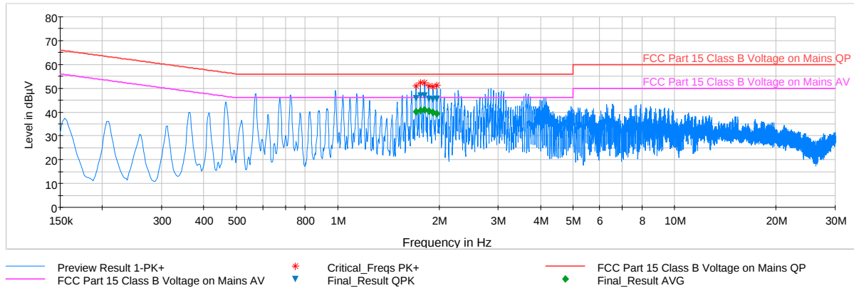
Plot 6-103. Line Conducted Plot with 802.11a UNII Band 3 (L1)
