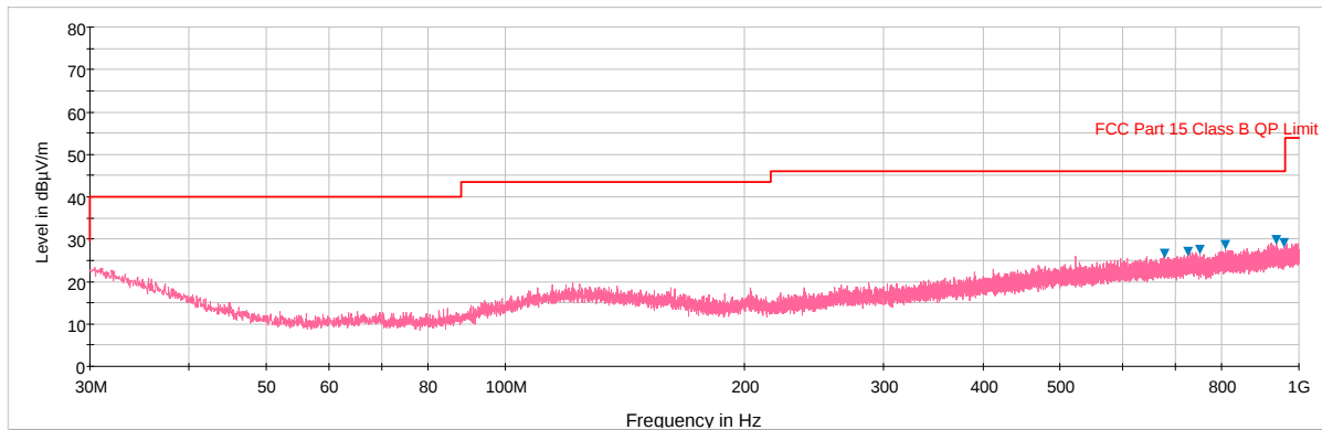
Plot 6-95. Radiated Spurious Plot below 1GHz (802.11a – U3 Ch. 157, Ant. Pol. H)
