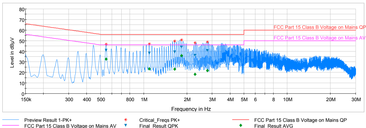
Plot 6-45. Line Conducted Plot with 802.11b (L1)
