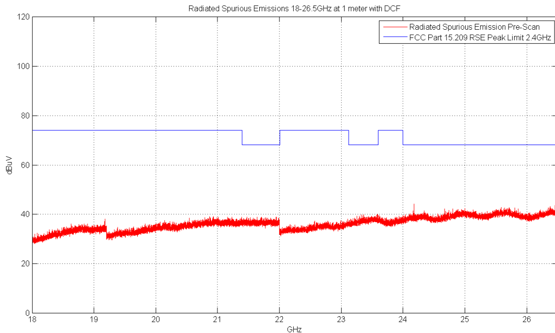
Plot 6-44. Radiated Spurious Plot above 18GHz (Pol. V)
