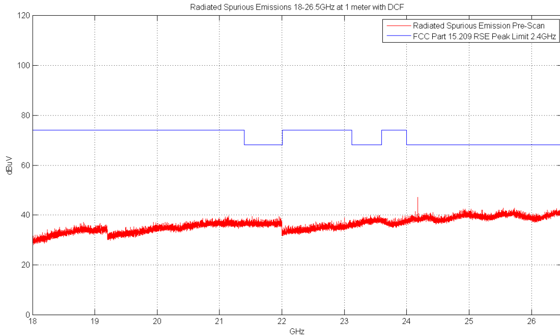
Plot 6-43. Radiated Spurious Plot above 18GHz (Pol. H)
