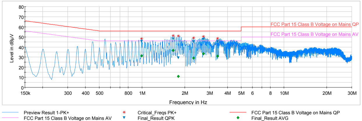
Plot 6-46. Line Conducted Plot with 802.11b (N)
