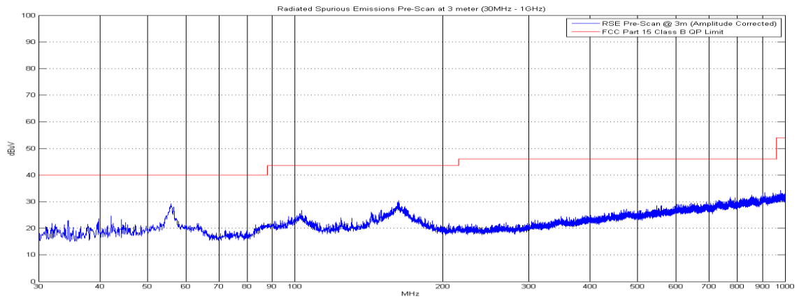
Plot 6-21. Radiated Spurious Plot below 1GHz (Pol. V)
