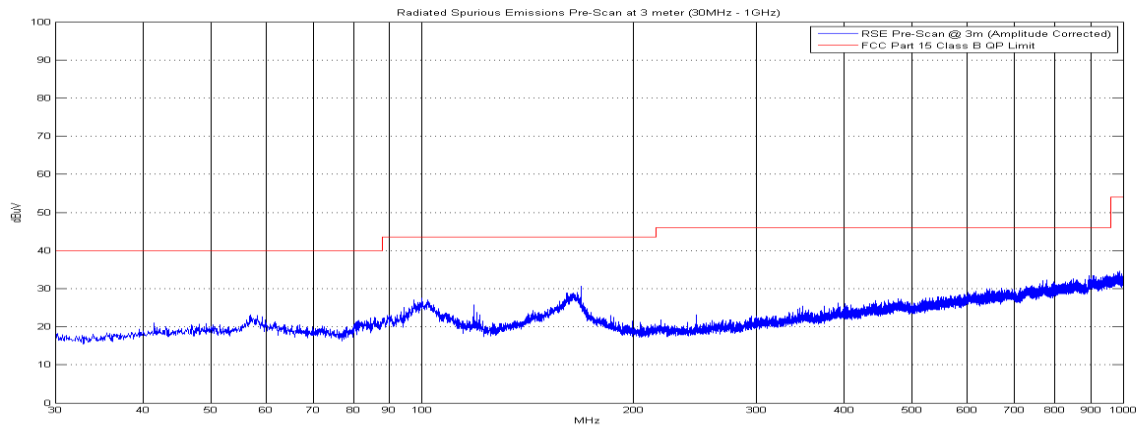
Plot 6-20. Radiated Spurious Plot below 1GHz (Pol. H)
