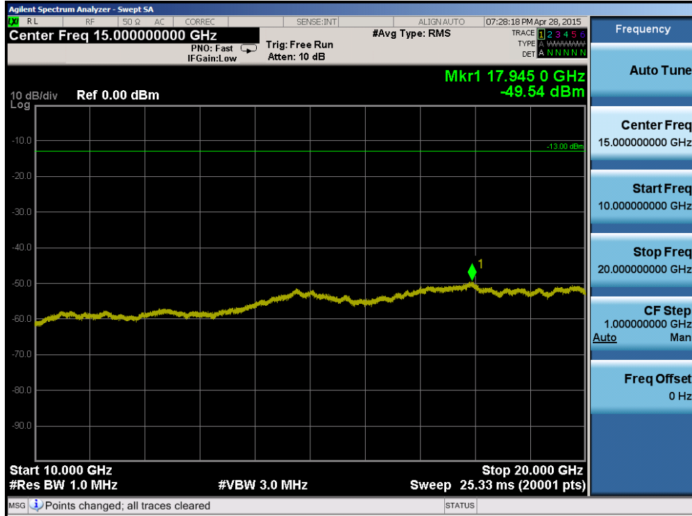
Plot 6-69. Conducted Spurious Plot (Band 2 – 20.0MHz QPSK – RB Size 1, RB Offset 0 – Mid Channel)
