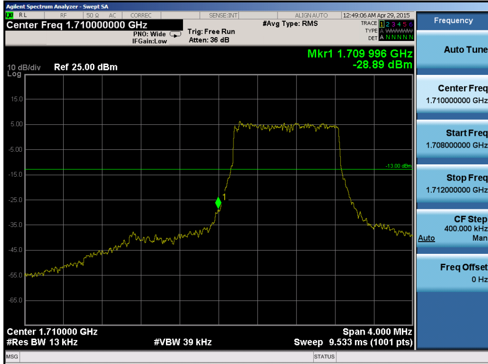
Plot 6-95. Lower Band Edge Plot (Band 4 – 1.4MHz QPSK – RB Size 6)
