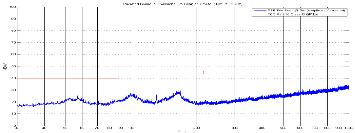
Plot 6-52. Radiated Spurious Plot below 1GHz (Pol. H)
