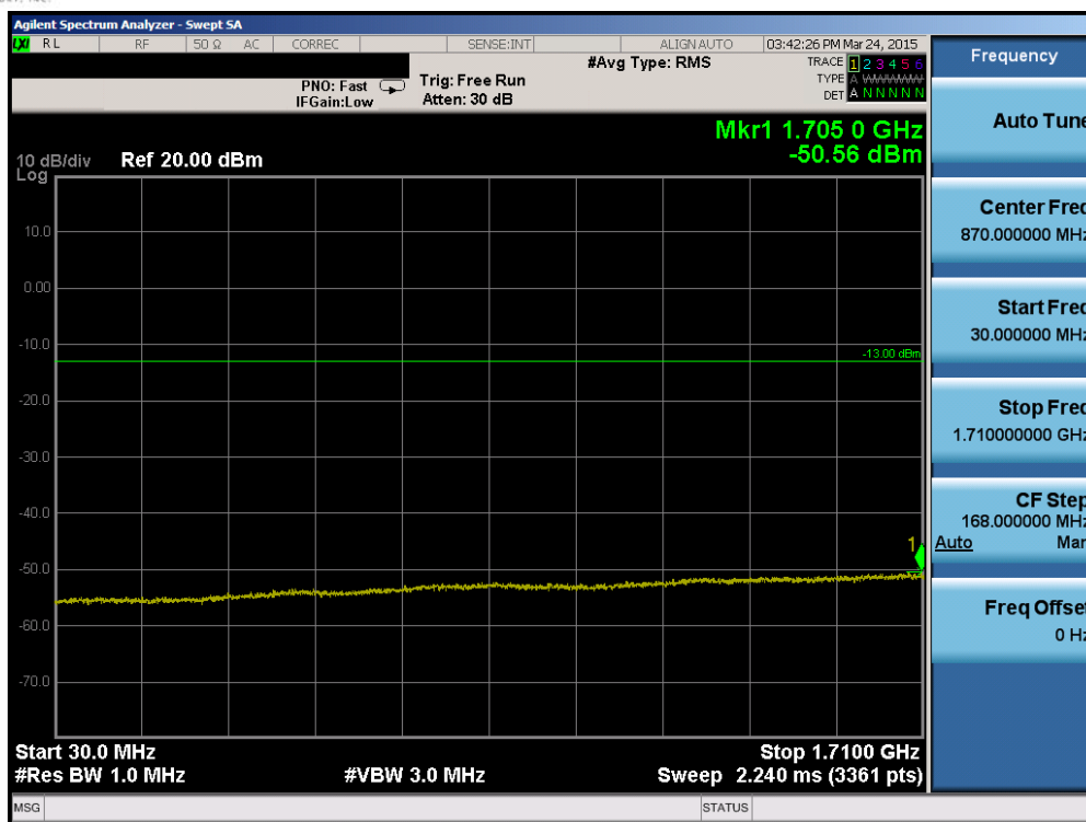
Plot 6-73. Conducted Spurious Plot (Band 4 – 10.0MHz QPSK – RB Size 1, RB Offset 0 – High Channel)
