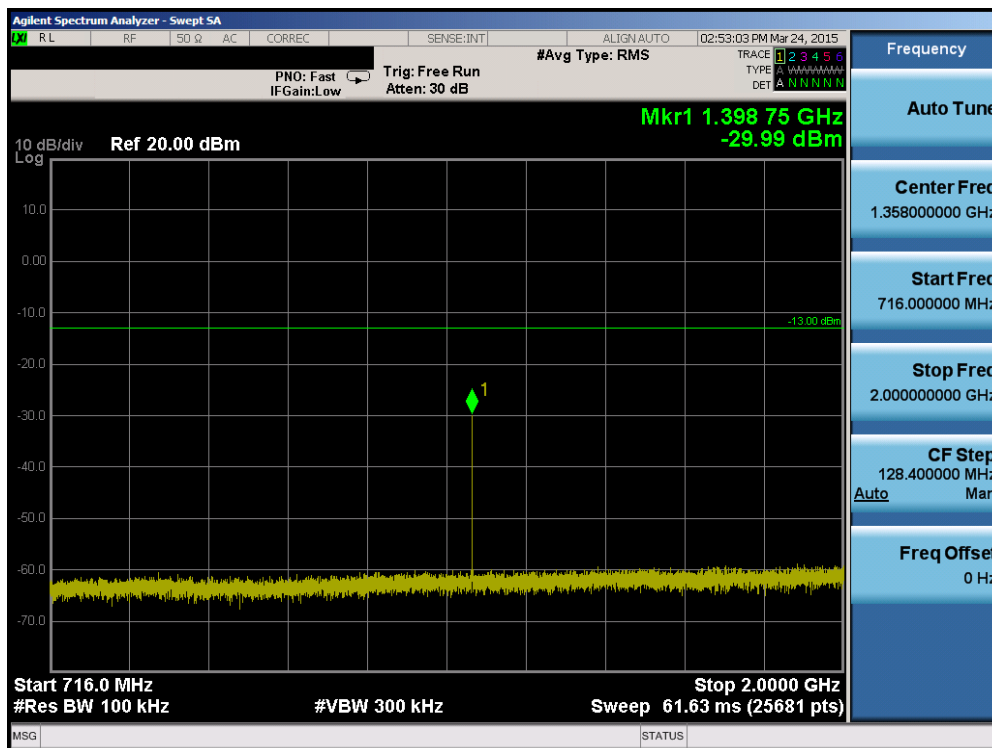
Plot 6-50. Conducted Spurious Plot (Band 12 – 5.0MHz QPSK – RB Size 1, RB Offset 0 – Low Channel)
