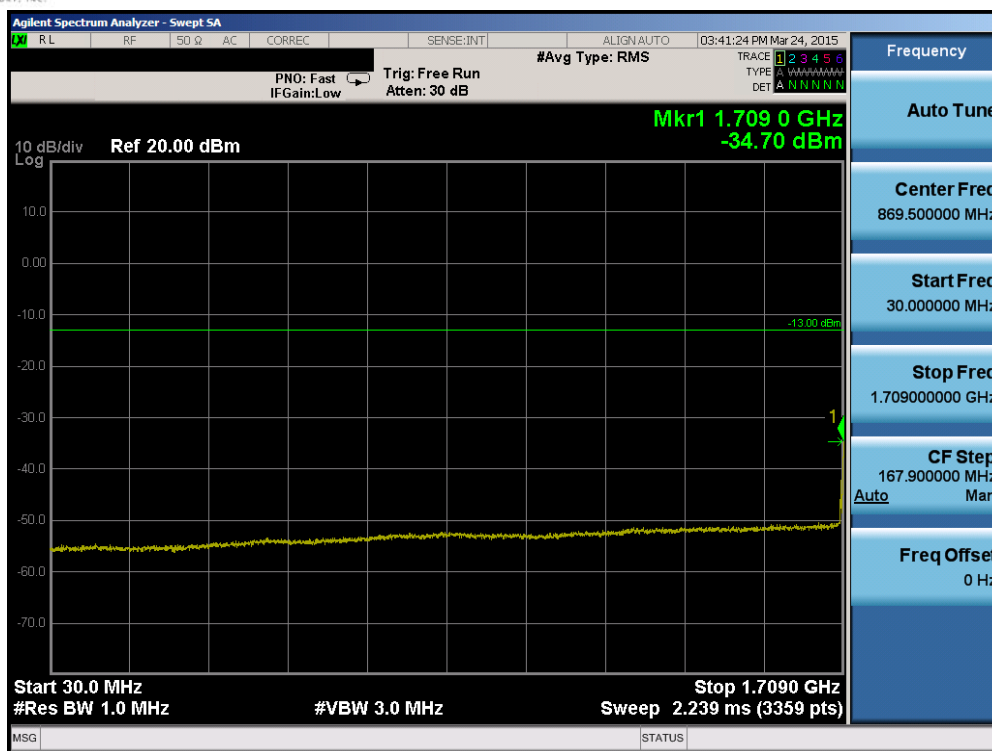
Plot 6-67. Conducted Spurious Plot (Band 4 – 10.0MHz QPSK – RB Size 1, RB Offset 0– Low Channel)
