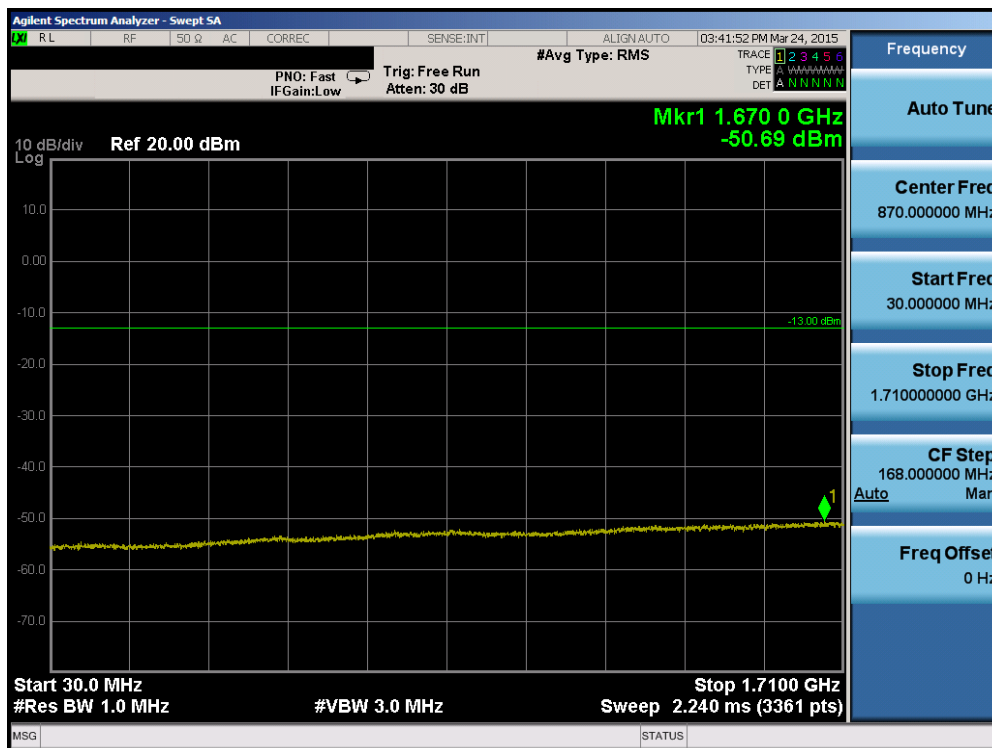
Plot 6-70. Conducted Spurious Plot (Band 4 – 10.0MHz QPSK – RB Size 1, RB Offset 0 – Mid Channel)
