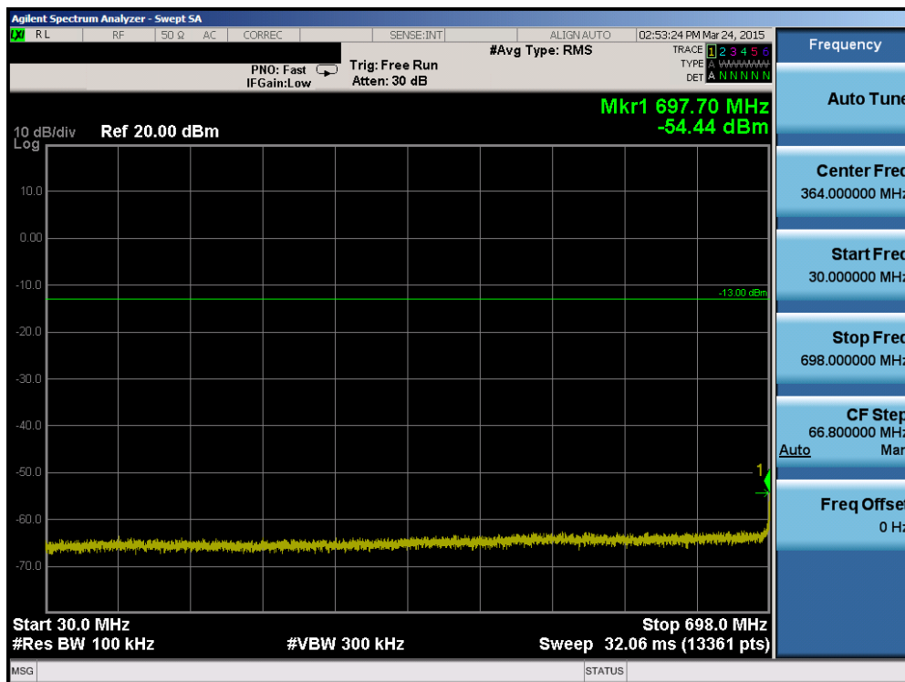
Plot 6-52. Conducted Spurious Plot (Band 12 – 5.0MHz QPSK – RB Size 1, RB Offset 0 – Mid Channel)
