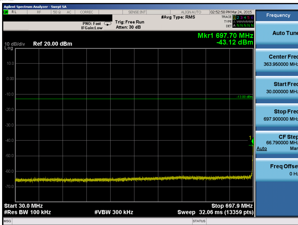
Plot 6-49. Conducted Spurious Plot (Band 12 – 5.0MHz QPSK – RB Size 1, RB Offset 0 – Low Channel)
