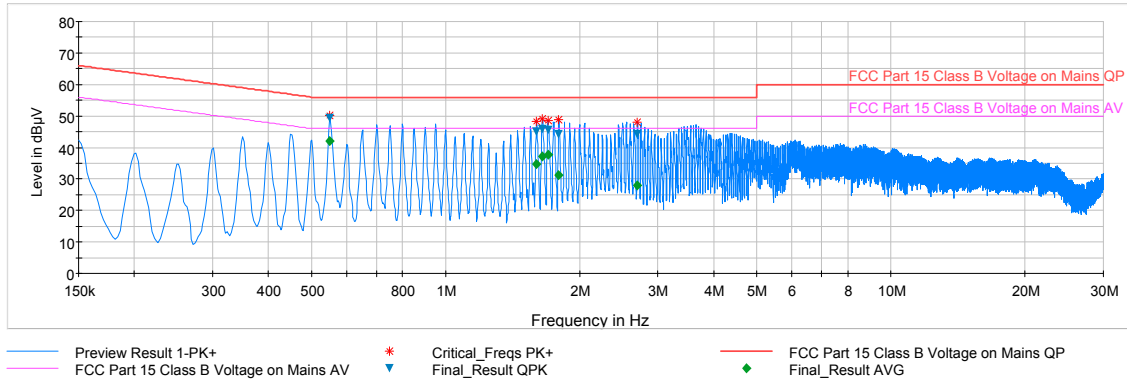
Plot 6-55. Line-Conducted Test Plot (N)
