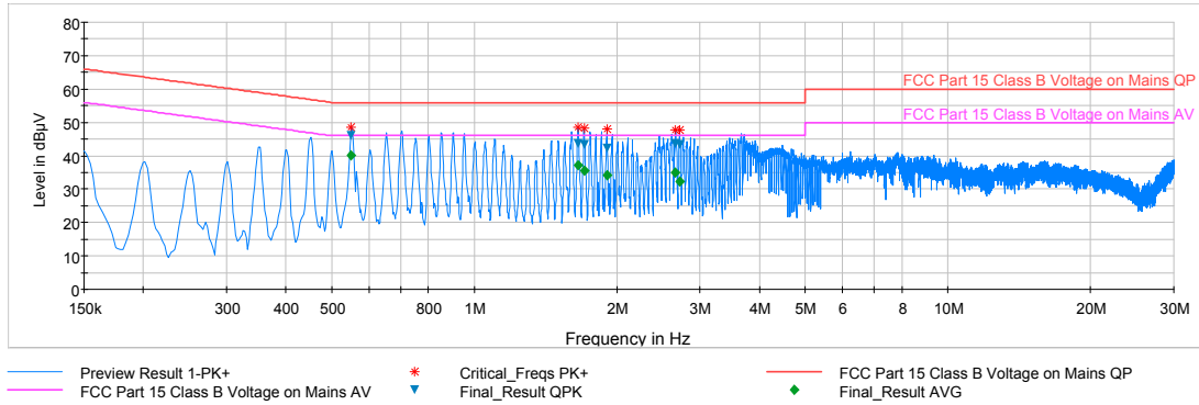
Plot 6-54. Line-Conducted Test Plot (L1)
