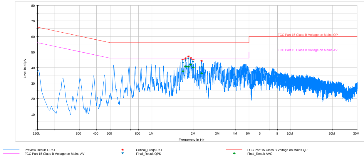
Plot 6-101. Line Conducted Plot with 802.11a UNII Band 2C (L1)
