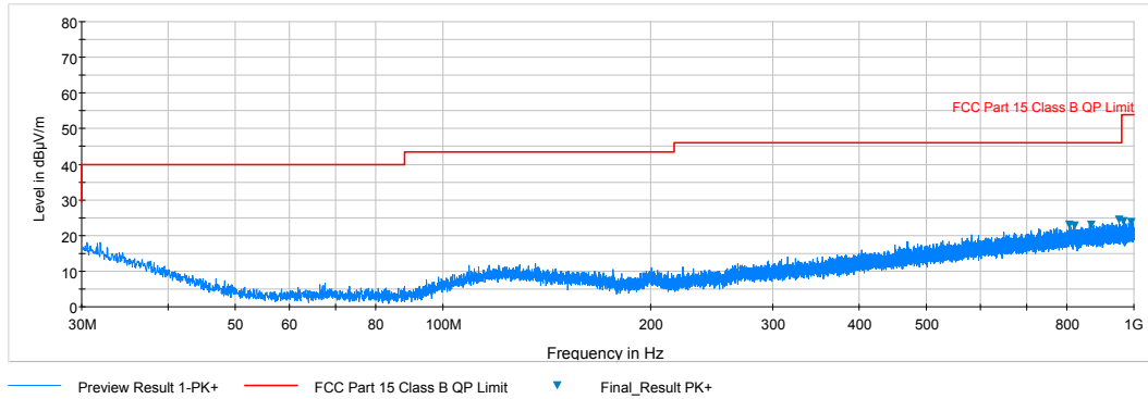
Plot 6-43. Radiated Spurious Plot below 1GHz (Pol. H)
