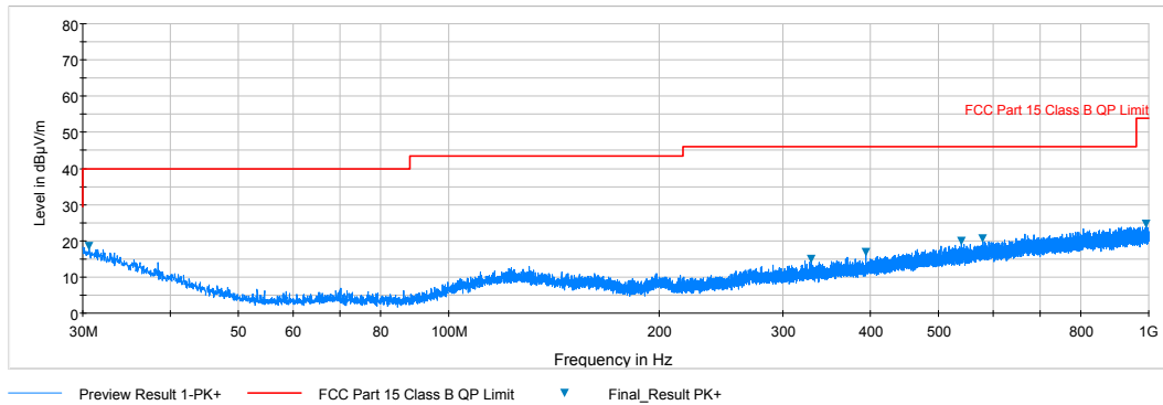
Plot 6-44. Radiated Spurious Plot below 1GHz (Pol. V)
