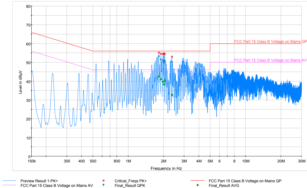
Plot 6-46. Line Conducted Plot with 802.11b (N)
