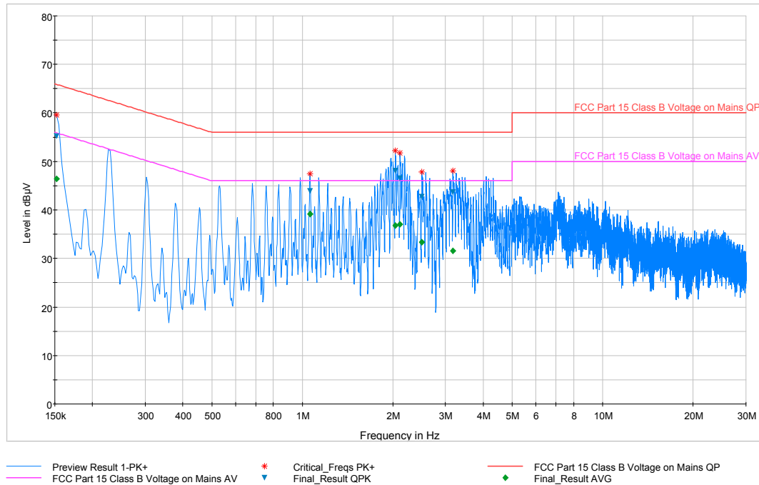
Plot 6-45. Line Conducted Plot with 802.11b (L1)
