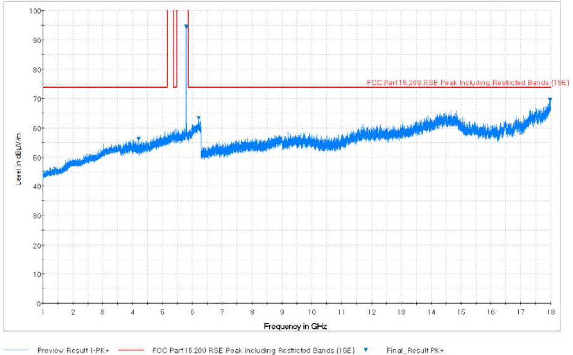
Plot 7-81. Radiated Spurious Plot above 1GHz (802.11a – U3 Ch. 157, Ant. Pol. H)
