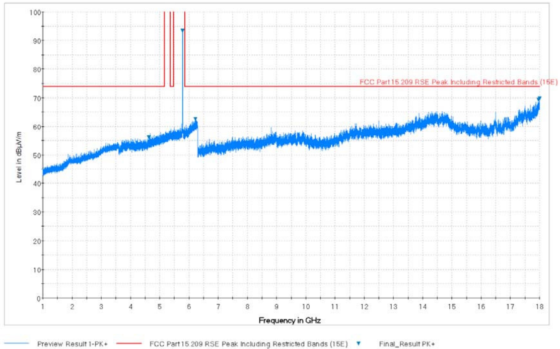
Plot 7-82. Radiated Spurious Plot above 1GHz (802.11a – U3 Ch. 157, Ant. Pol. V)
