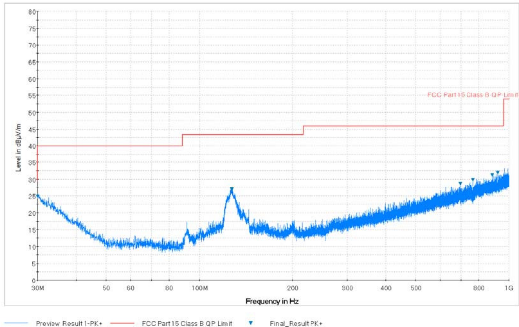
Plot 7-109. Radiated Spurious Plot below 1GHz (802.11a – U3 Ch. 157, Ant. Pol. V)
