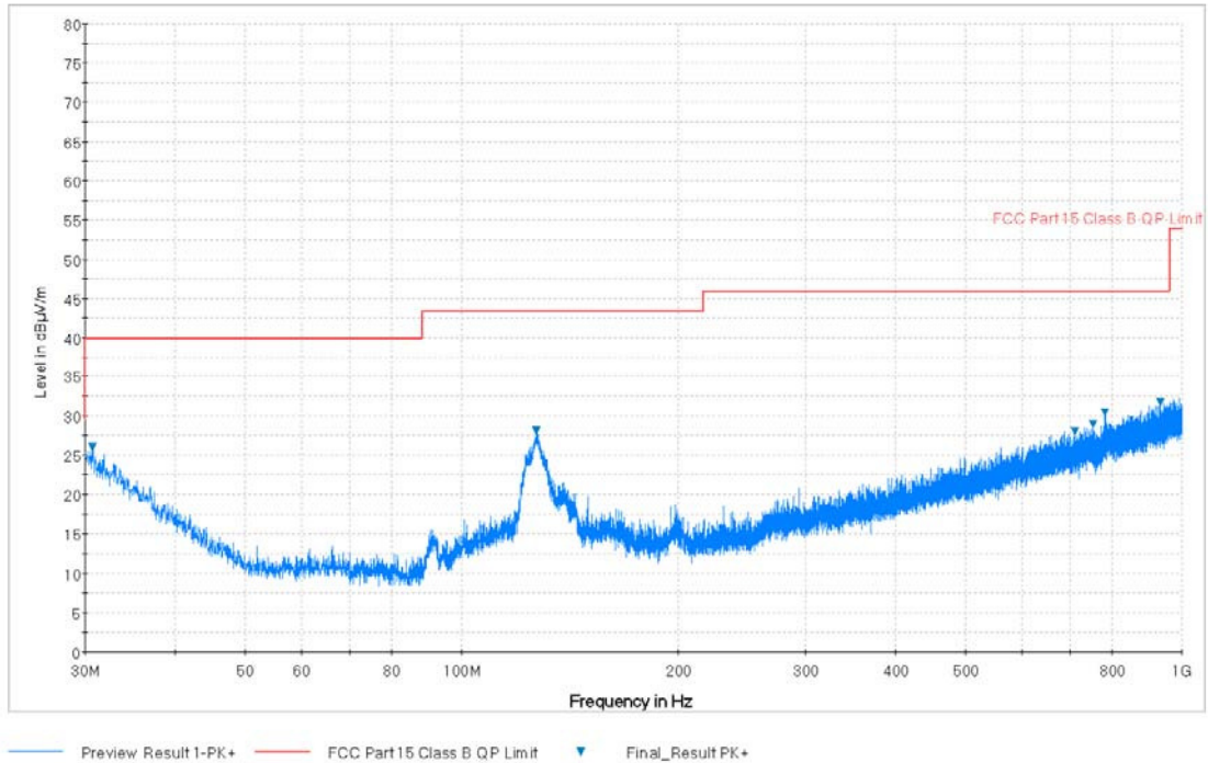
Plot 7-108. Radiated Spurious Plot below 1GHz (802.11a – U3 Ch. 157, Ant. Pol. H)
