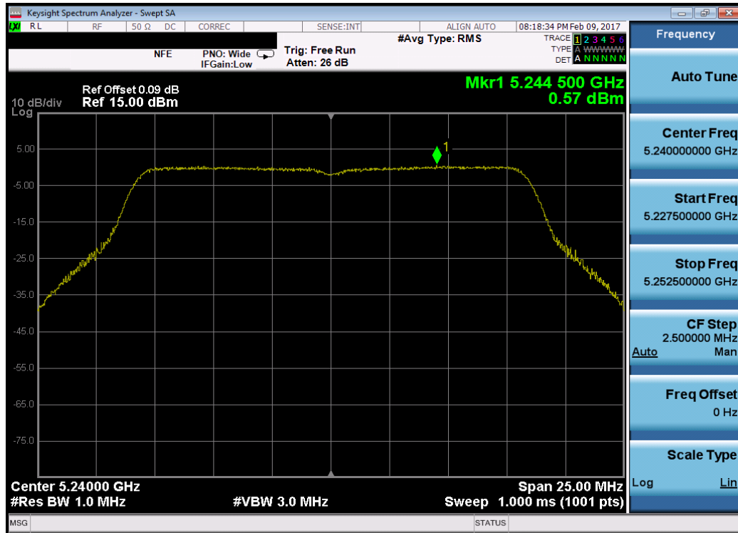
Plot 7-40. Power Spectral Density Plot (802.11a (UNII Band 1) – Ch. 48)
