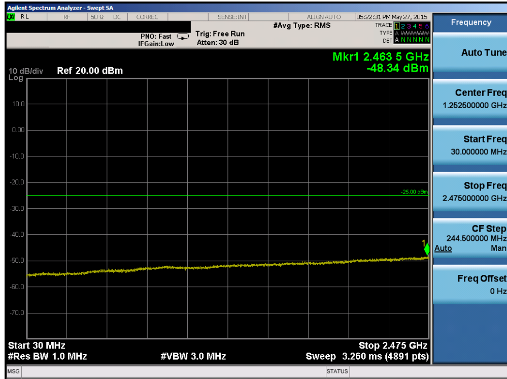
Plot 6-109. Conducted Spurious Plot (Band 7 – 15.0MHz QPSK – RB Size 1, RB Offset 0 – High Channel)
