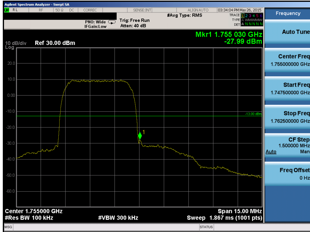
Plot 6-63. Band Edge Plot (AWS WCDMA Mode – Ch. 1862)
