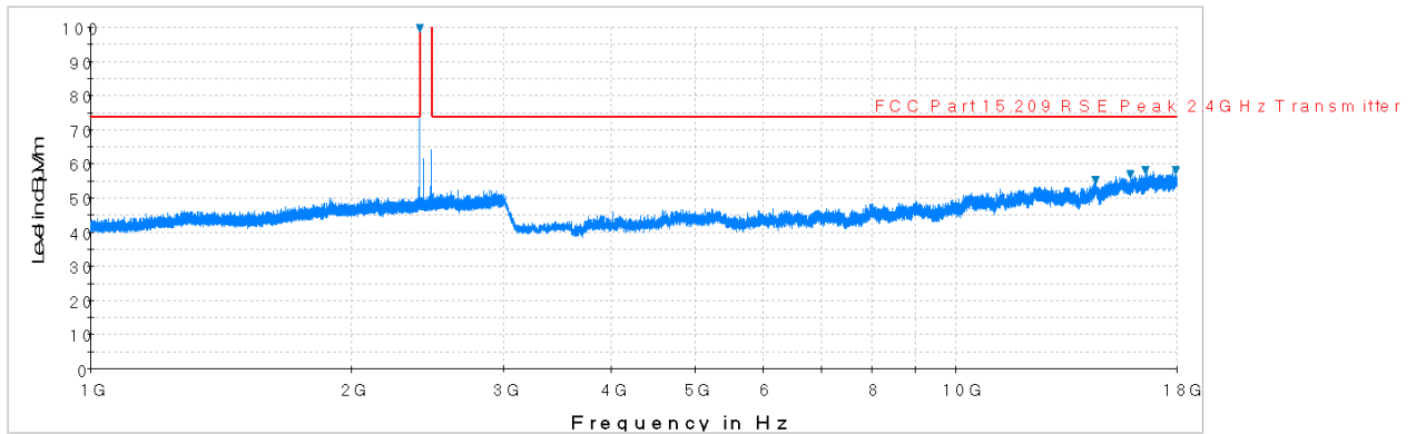
Plot 6-42. Radiated Spurious Plot above 1GHz (BT – Ch. 0, Ant. Pol. H)
