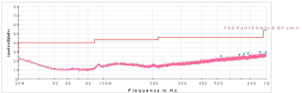
Plot 6-53. Radiated Spurious Plot below 1GHz (Pol. V)
