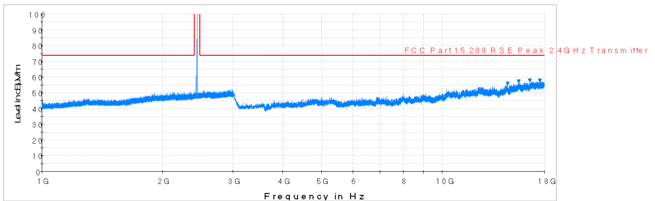
Plot 6-44. Radiated Spurious Plot above 1GHz (BT – Ch. 39, Ant. Pol. H)
