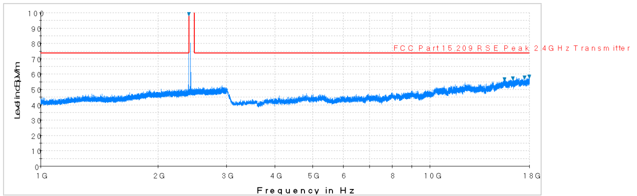
Plot 6-43. Radiated Spurious Plot above 1GHz (BT – Ch. 0, Ant. Pol. V)
