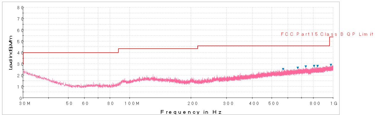
Plot 6-52. Radiated Spurious Plot below 1GHz (Pol. H)
