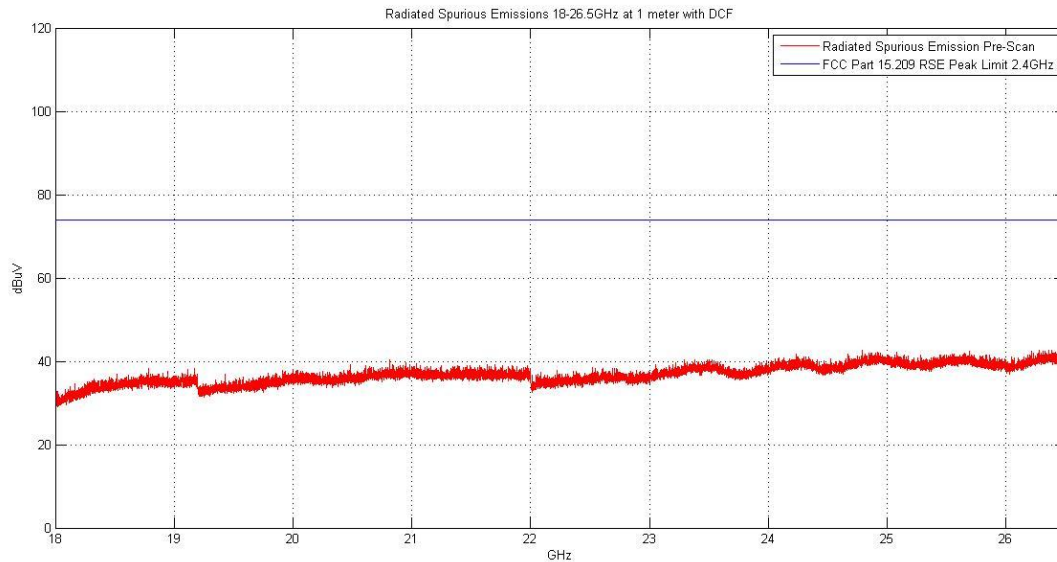
Plot 6-48. Radiated Spurious Plot above 18GHz (Pol. H)
