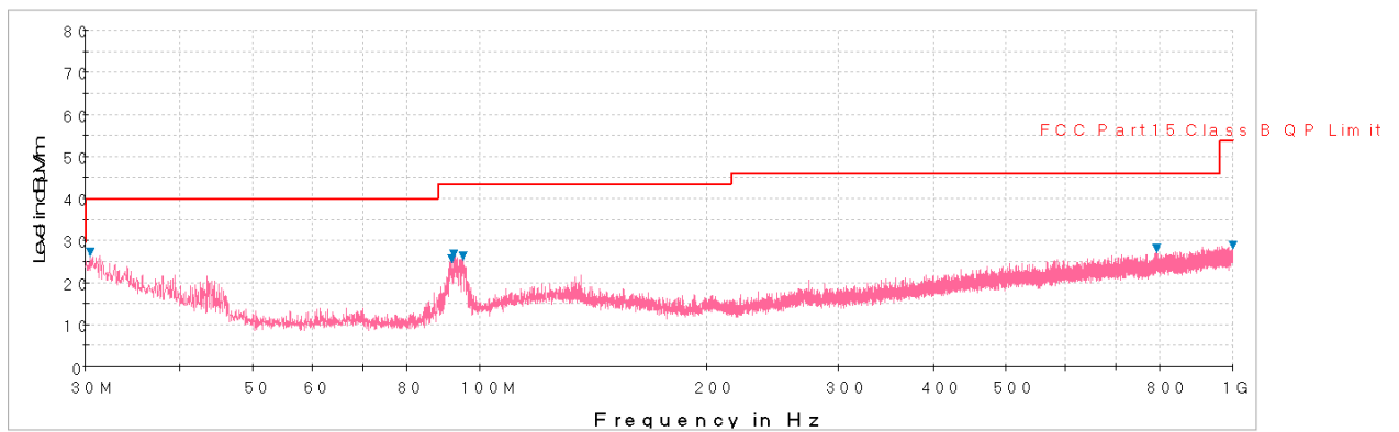
Plot 6-42. Radiated Spurious Plot below 1GHz (Pol. V)
