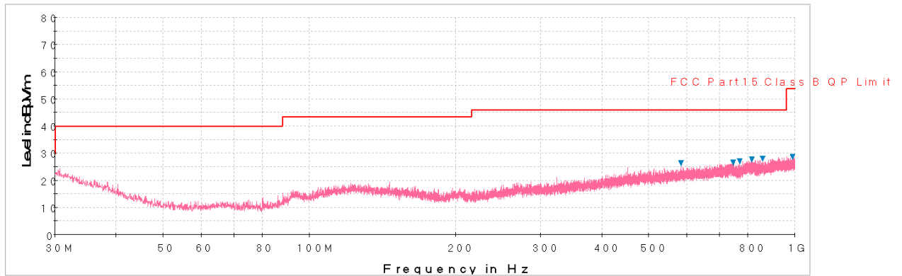
Plot 6-41. Radiated Spurious Plot below 1GHz (Pol. H)
