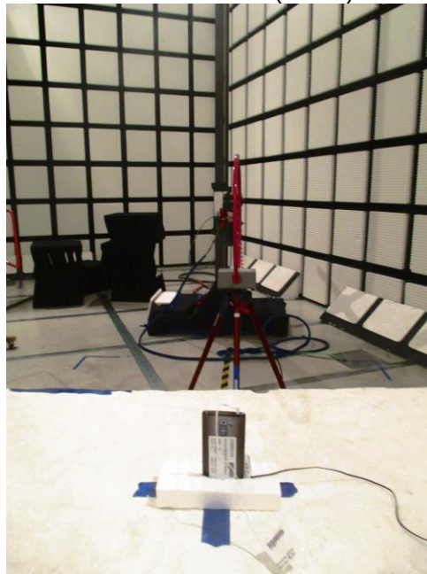
RADIATED EMISSIONS BELOW 30MHz (BACK)
