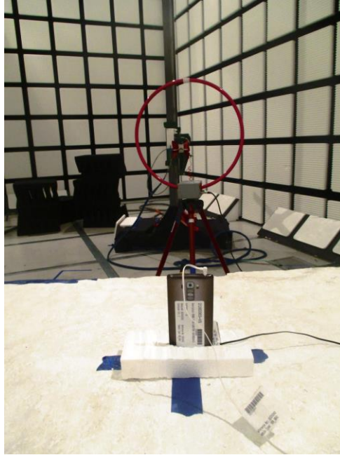
RADIATED EMISSIONS BELOW 30MHz (FRONT)
