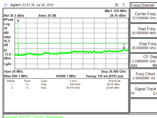
Band LTE26 15MHz CSE 16QAM Mid channel
