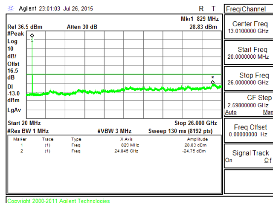
Band LTE26 15MHz CSE QPSK Mid channel
