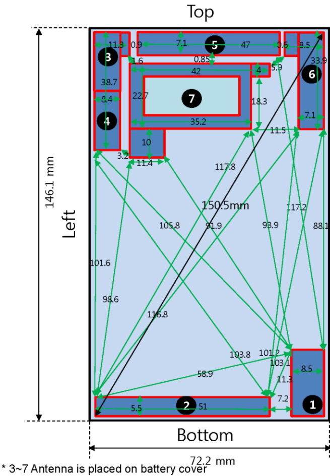
H790 Antenna Distance(Front View)
